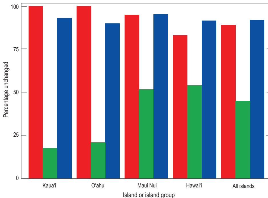
Figure 3.10. Plot of proportion of each island's current moisture-zone distribution projected to remain unchanged between now and the end of the century. Maui Nui includes the islands of Maui, Molokaʻi, Lānaʻi, and Kahoʻolawe.
