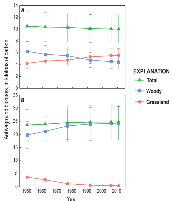
Figure 5.5. Plots of aboveground carbon partitioned into grassland and woody vegetation contained in the active, wildland-fire training area at Schofield Barracks, O‘ahu, Hawai‘i (A), an area subject to frequent wildland fires, and in the watershed area outside of the training area (B), where wildland fire breaks and suppression have limited wildland fire incursion. Mean values are shown with \pm 1 standard deviation error bars.
