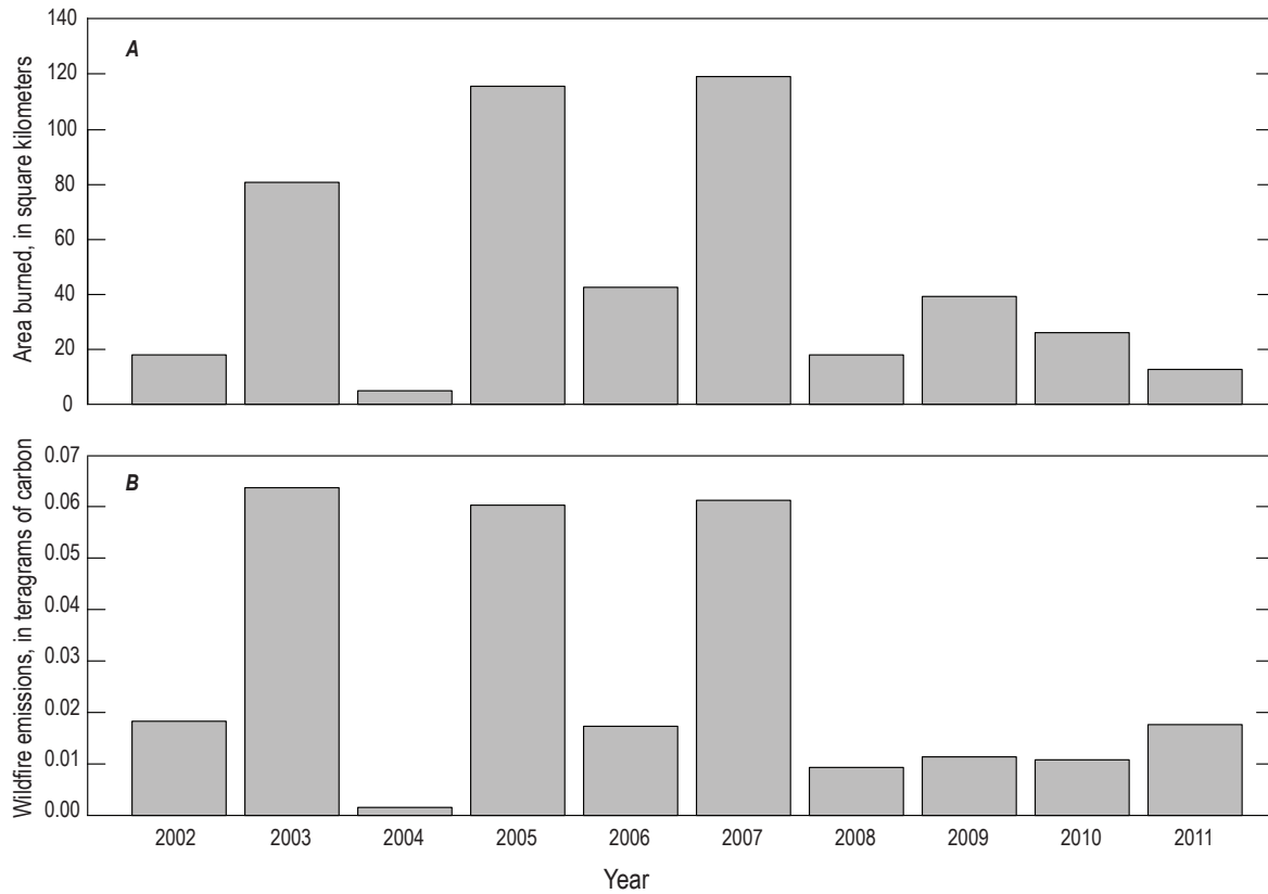
Figure 5.3. Plots of annual area burned (A) and wildland fire emissions (B) from 2002 to 2011 across all of the main Hawaiian Islands excluding Kaho'olawe and Lana'i.
