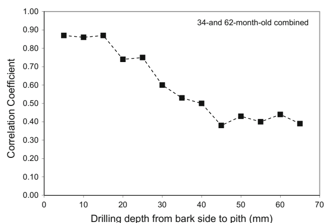
Fig. 8 Correlation coefficient for the relationship between measured drilling resistance (expressed as amplitude in resistance profile) and specific gravity of 34- and 62-month-old Eucalyptus grandis \times Eucalyptus urophylla trees as affected by the drilling depth (from Oliveira et al. 2017, with permission)
