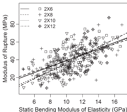
Figure 4. Linear regression plot of static MOE ( E_{SB} ) and MOR, each lumber size.
