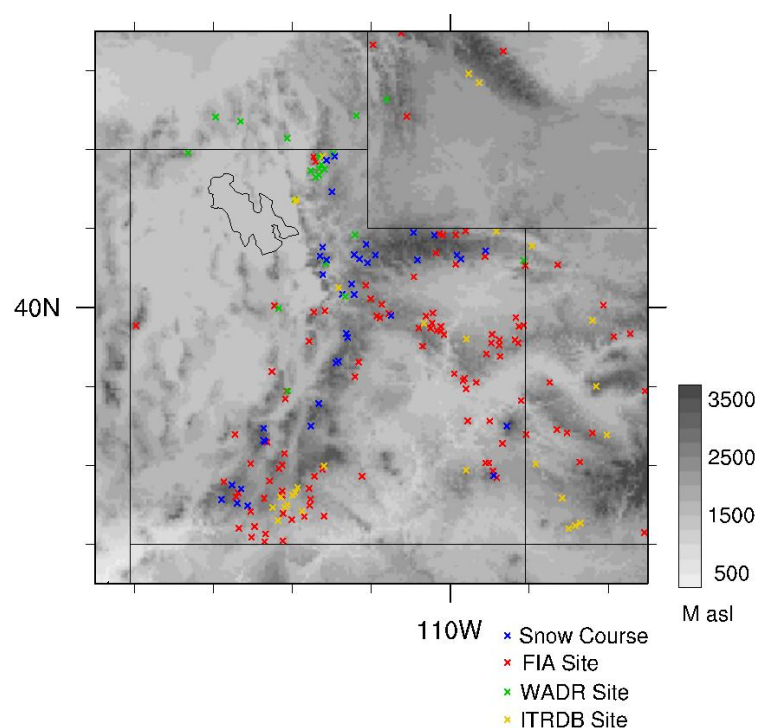
Figure 1. Terrain in the state of Utah (grayscale). Locations of snow course stations (blue x), and tree-ring data type, Forest Inventory and Analysis (FIA) plots (red x), Wasatch Dendroclimatology Research group (WADR) site (green x), and International Tree-Ring Data Bank (ITRDB) sites (yellow x). ITRDB and WADR sites are fully developed chronologies; FIA plots are locations of individual tree increment cores.
