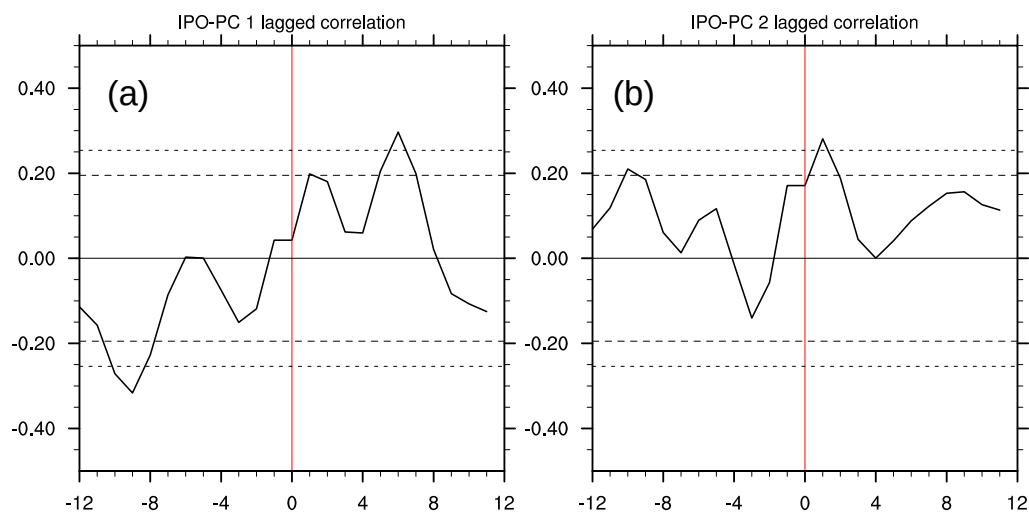
Figure 6. Lagged correlation of PC1 (a) and PC2 (b) with a four-year low-pass filtered IPO. Dashed lines denote significant correlation at 95% and 99% confidence levels.
