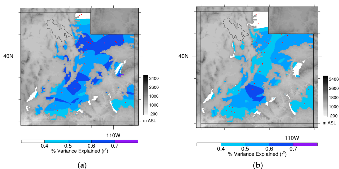
Figure 4. Point-to-point R^2 map of reconstructed-to-observed April 1 SWE, (a) including and (b) excluding FIA tree-ring data. Red points are snow courses.
