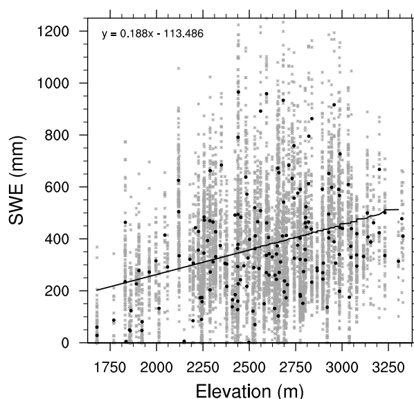
Figure 2. April 1 SWE vs. elevation in Utah. Bold black points show the mean value for each snow course, and grey points show the individual measurements. The solid line is the linear regression of the mean snow course values with respect to elevation; the regression function is shown in the top left.
