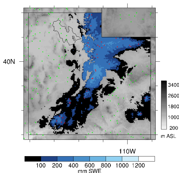
Figure 3. Sample regridded April 1 SWE. Red points indicate the locations of snow courses, green points indicate the locations of dummy observations used in zero-padding conditioning prior to Cressman interpolation.
