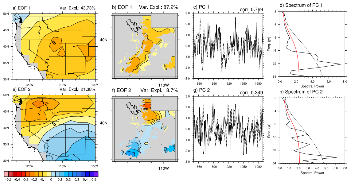
Figure 5. (a) EOF 1 for NADA; (b) EOF 1 for FIA; (c) PC1 of reconstructed SWE for (a,b) (solid: FIA, dashed: NADA); and (d) spectral power of FIA PC1. In (d), the red line depicts the red noise spectrum and the dashed line indicates red noise exceedance at 95% confidence. (e–h) Same as (a–d) but for EOF 2 and FIA PC 2.
