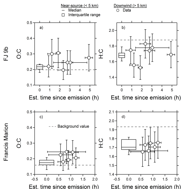
Figure 5. Evolution of elemental ratios derived from AMS data. (a) O:C for the FJ 9b fire; (b) H:C for the FJ 9b fire; (c) O:C for the Francis Marion fire; (d) H:C for the Francis Marion fire. For both fires, changes in O:C with increasing estimated time since emission are statistically significant. Dashed line is the value of the parameter in the background measurements outside of plume penetrations. Box-and-whisker plots and markers are used in the same way as those in Figs. 2 and 3.
