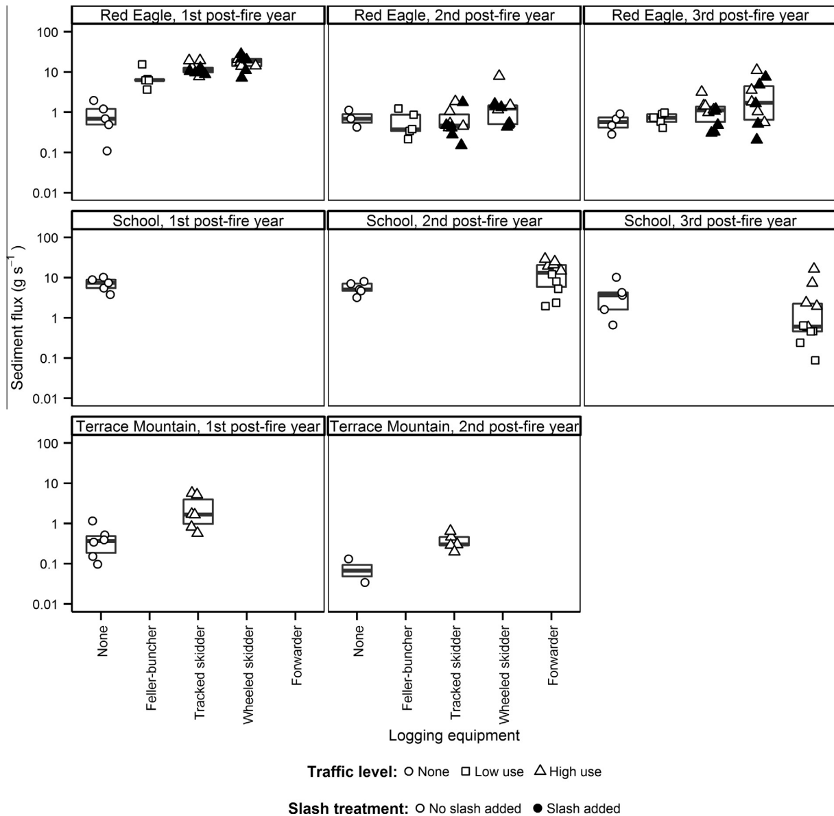
Fig. 4. Mean plot sediment flux by type of logging equipment and post-fire year for each site. Symbol fill indicates slash treatment and symbol shape indicates traffic level. Boxplot characteristics are the same as in Fig. 2. Individual plot values are shown in Supplemental material and results of statistical analyses are shown in Table A3.
