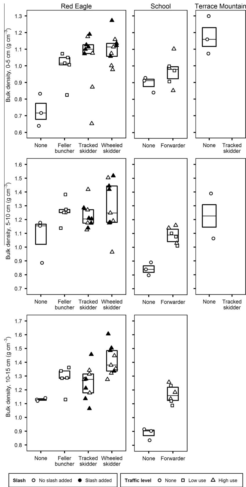
Fig. 2. Soil bulk density at depths of 0–5 cm, 5–10 cm, and 10–15 cm by type of logging equipment and site. Symbol fill indicates slash treatment and symbol shape indicates traffic level. At Terrace Mountain, bulk density was not sampled in skid trail plots or below 10 cm depth. Each box represents the median, first quartile, and third quartile; points are individual observations. Individual plot values are shown in Supplemental material and results of statistical analyses are shown in Table A1 .
