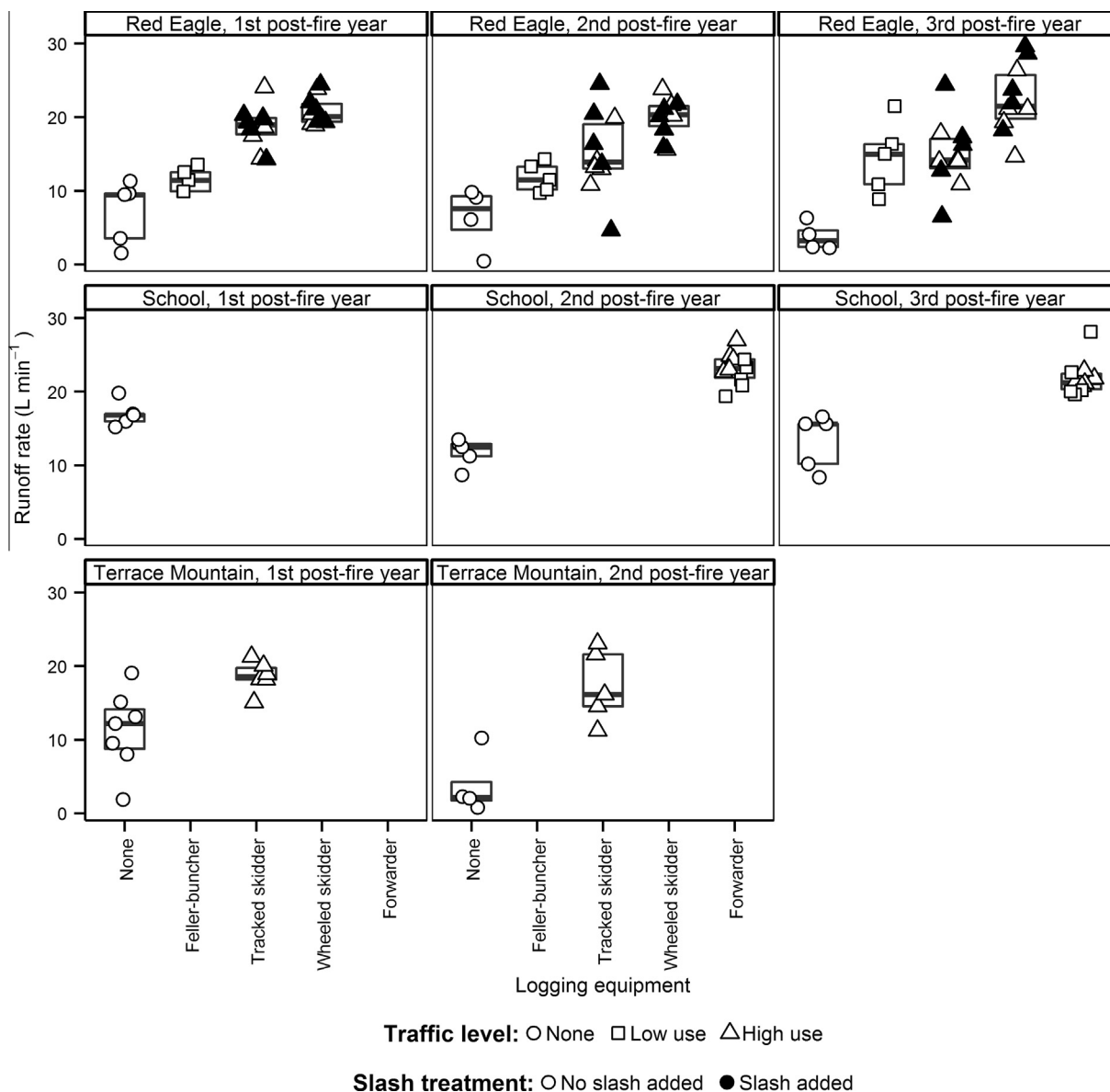
Fig. 3. Mean plot runoff rate by type of logging equipment and post-fire year for each site. Symbol fill indicates slash treatment and symbol shape indicates traffic level. Boxplot characteristics are the same as in Fig. 2. Individual plot values are shown in Supplemental material and results of statistical analyses are shown in Table A2.
