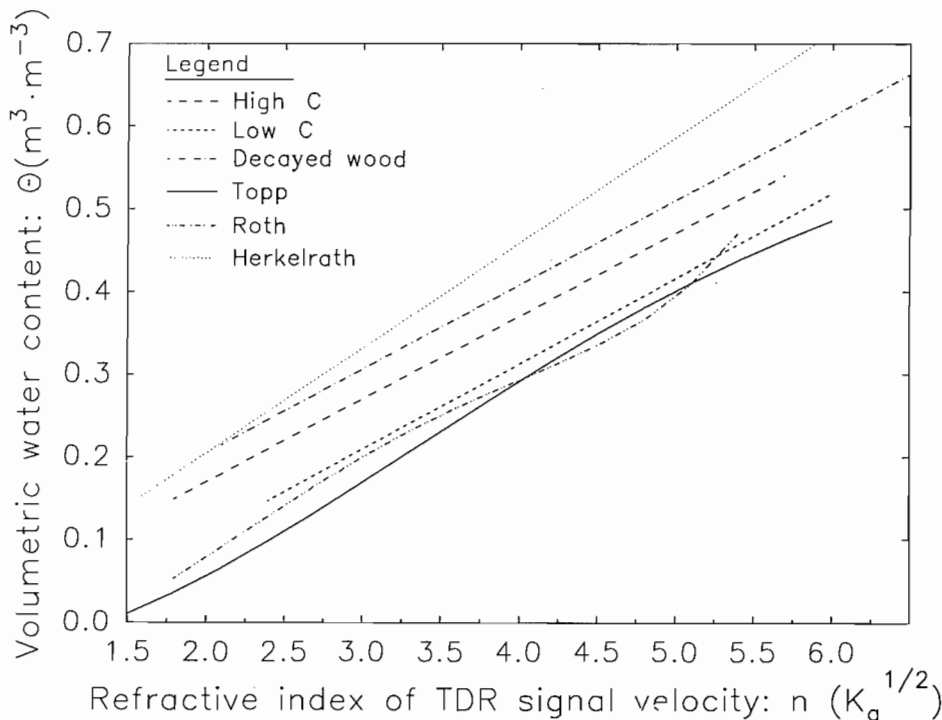
Fig. 5. TDR calibration equations from Topp et al. (1980), Herkelrath et al. (1991), and Roth et al. (1992) are compared with low-C, High-C, and decayed wood equations from this study.
