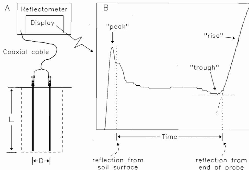
Fig. 1. (A) Schematic of TDR probes in soil illustrating cable and alligator clip connection to steel rods. Most of the volume sampled is equal to \pi D^2 L . (B) Trace resulting from signal reflections to the reflectometer, illustrating use of tangent lines to define probe end reflection.
