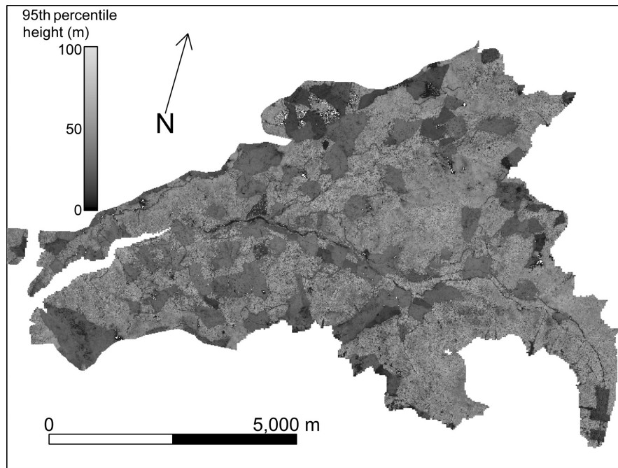
FIG. 2. Canopy height (m; 95th percentile) for lidar first returns more than 1 meter above the ground within 5-m footprints.
