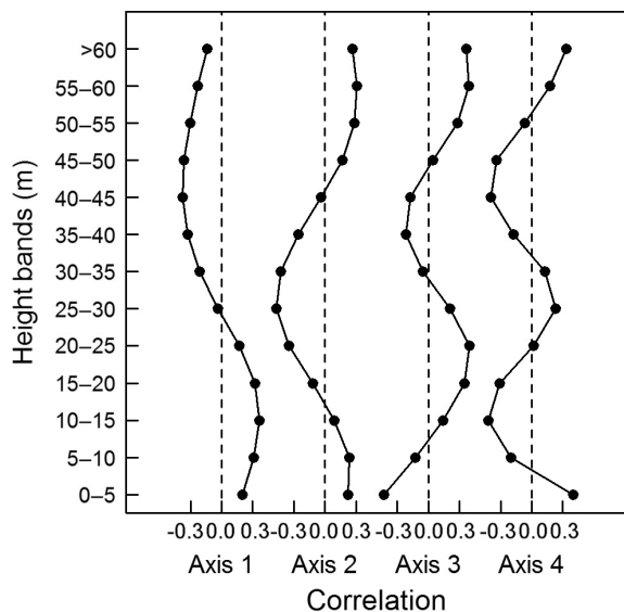
FIG. 3. Correlations between the first four axes of a principal components analysis (PCA) and the proportion of returns for an individual pixel falling into different 5-m height bands.
