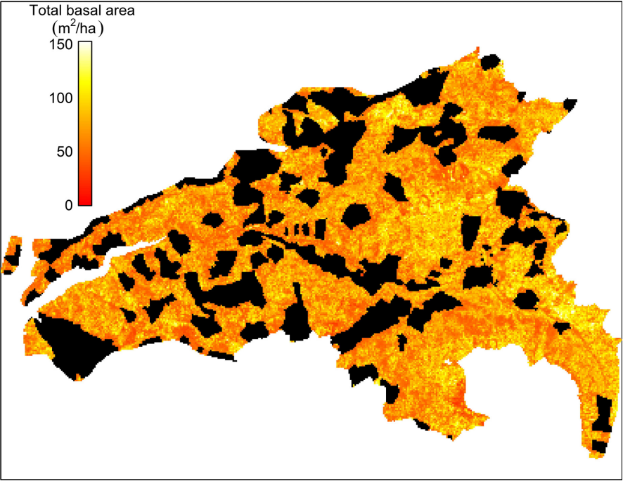
FIG. 4. Mean predicted total tree basal area (lower canopy + upper canopy trees) for the study area. Black areas represent timber harvests and were not modeled (Fig. 1b). [Color figure can be viewed at wileyonlinelibrary.com ]
