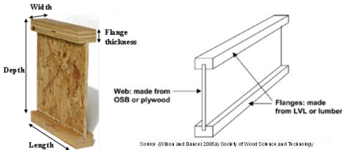
Figure 2. Typical composite I-joists shown here made with laminated veneer lumber (LVL) flanges and an oriented strandboard (OSB) web.
