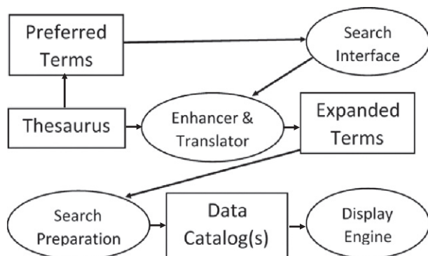
Fig. 3. Diagram of multilingual search system elements.
