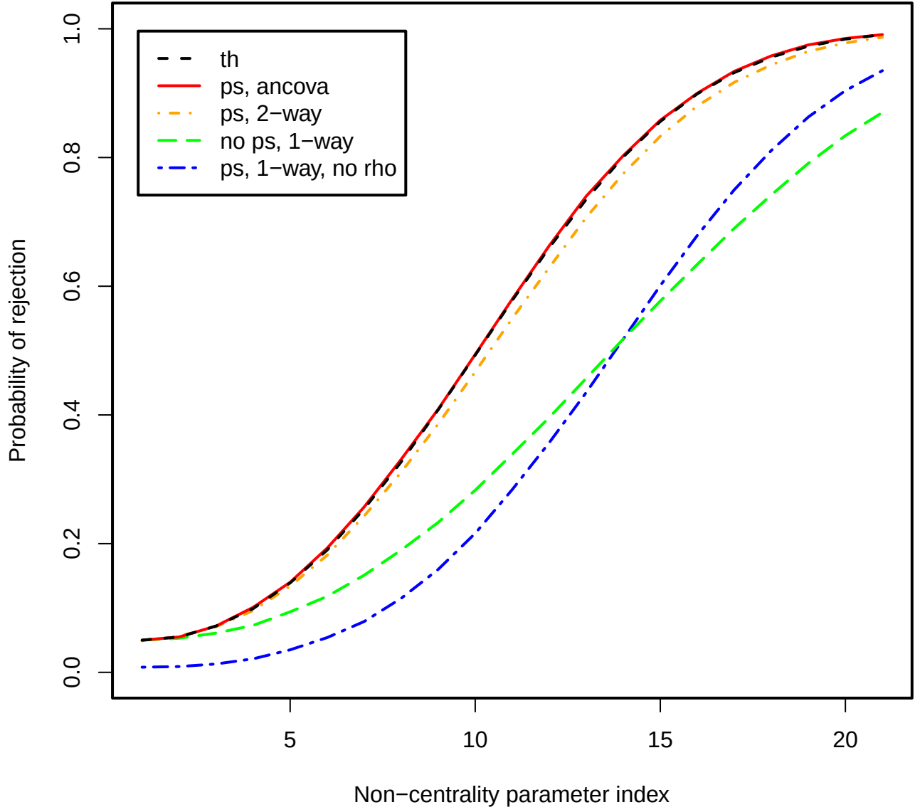
Figure 8: Power plot, \rho = 0.7 , J = 2 , I = 20 .
