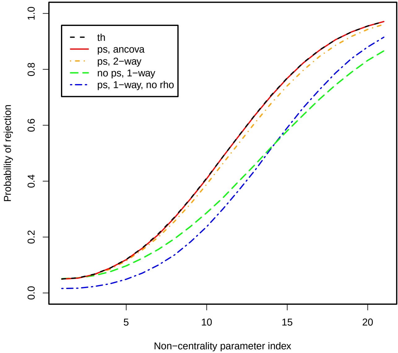
Figure 6: Power plot, \rho = 0.6 , J = 2 , I = 20 .
