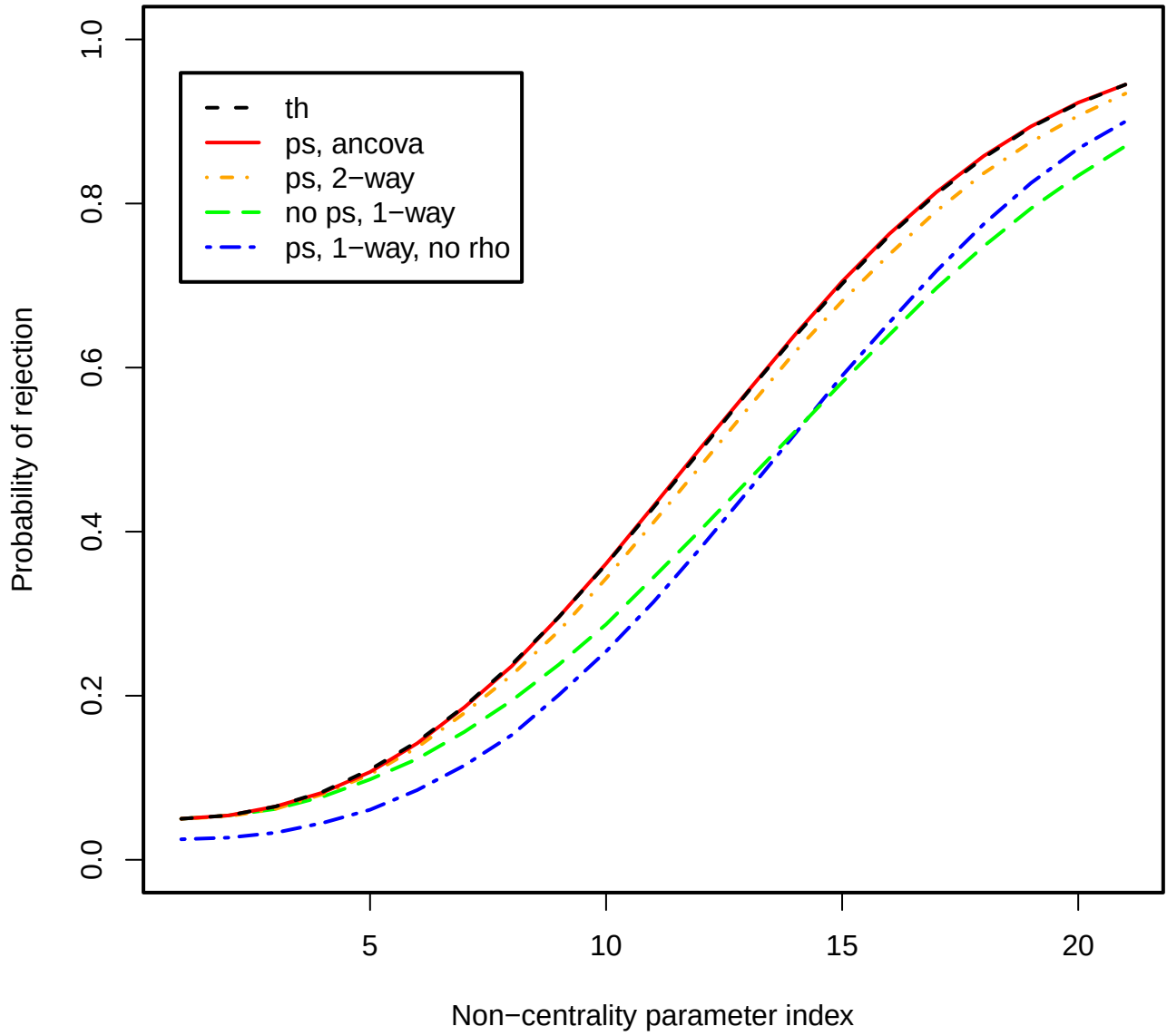
Figure 4: Power plot, \rho = 0.5 , J = 2 , I = 20 .
