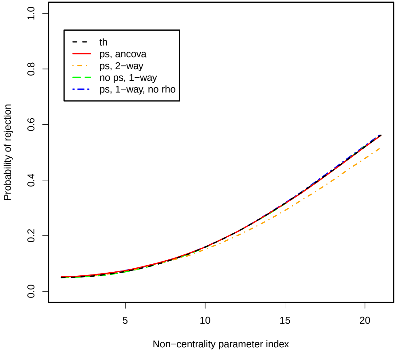
Figure 1: Power plot, \rho = 0.0 , J = 2 , I = 10 .
