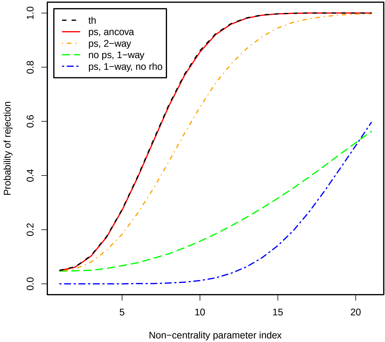
Figure 13: Power plot, \rho = 0.95 , J = 2 , I = 10 .
