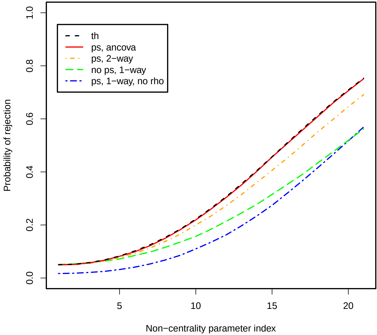
Figure 5: Power plot, \rho = 0.6 , J = 2 , I = 10 .
