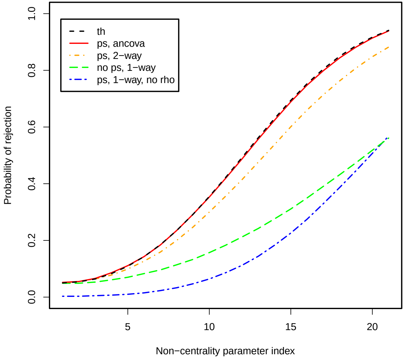
Figure 9: Power plot, \rho = 0.8 , J = 2 , I = 10 .
