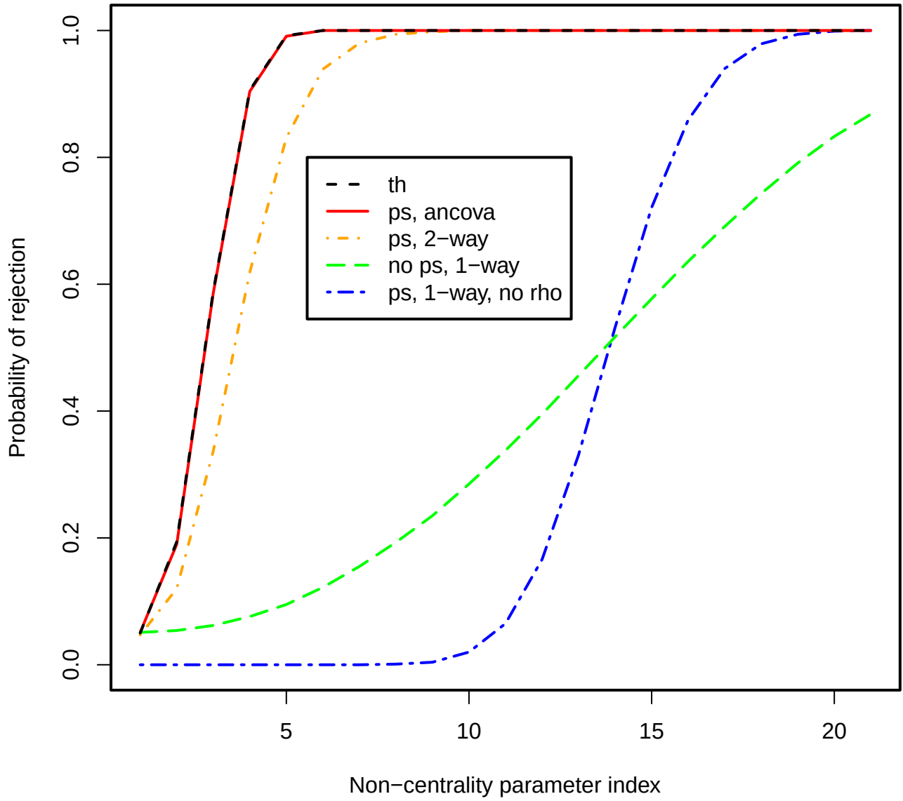
Figure 16: Power plot, \rho = 0.99 , J = 2 , I = 20 .
