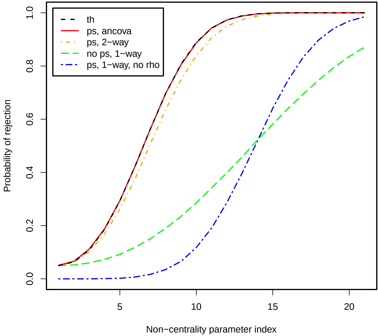
Figure 12: Power plot, \rho = 0.9 , J = 2 , I = 20 .
