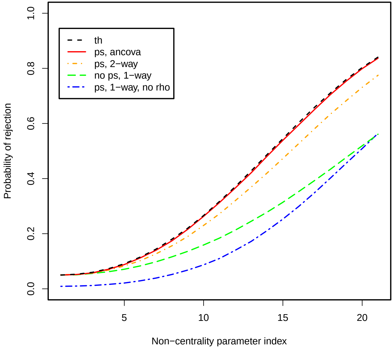
Figure 7: Power plot, \rho = 0.7 , J = 2 , I = 10 .
