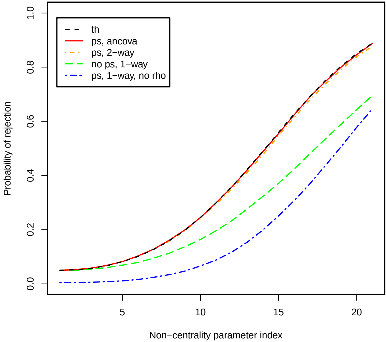
Figure 22: Power plot, \rho = 0.6 , J = 5 , I = 20 .
