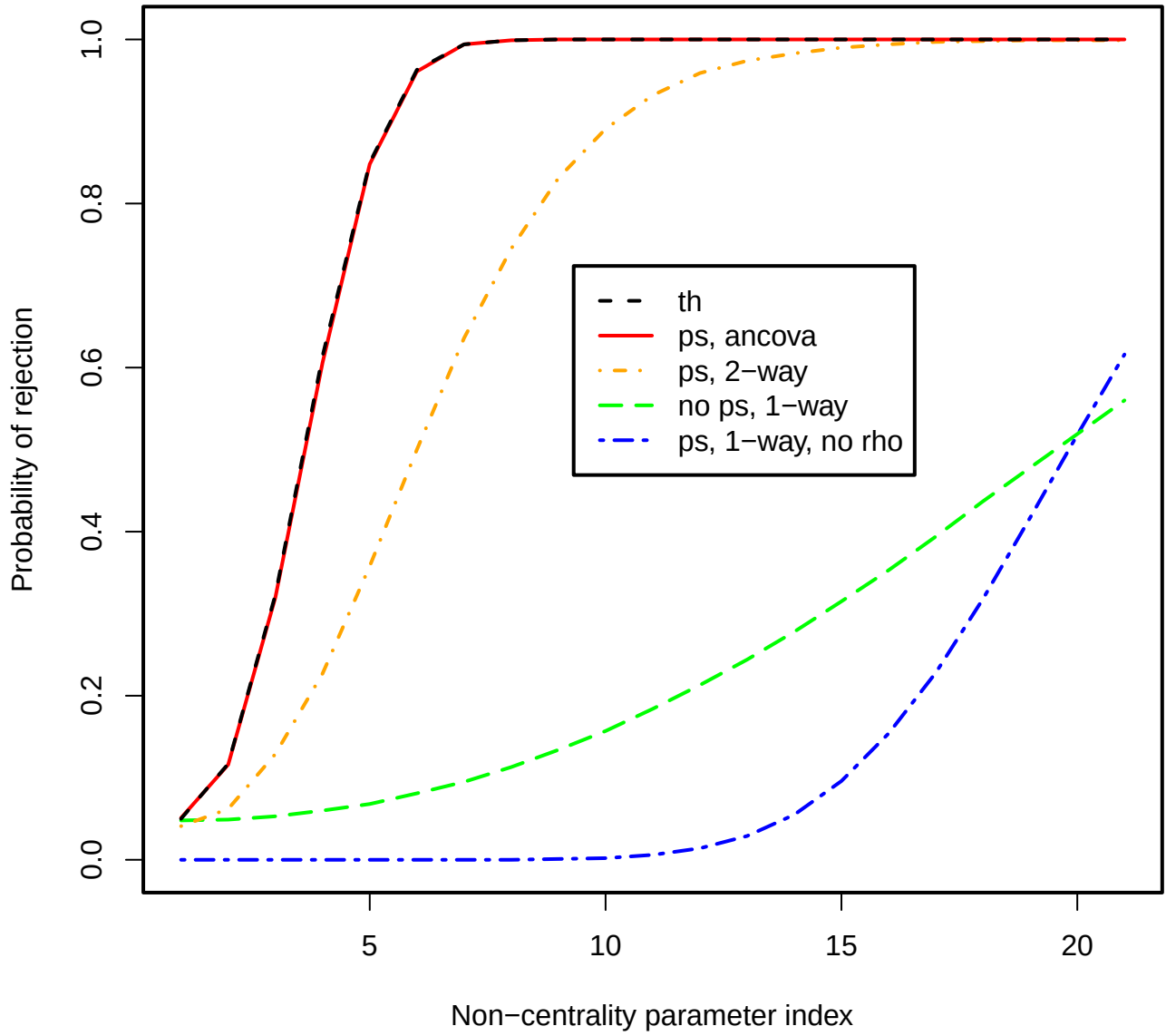
Figure 15: Power plot, \rho = 0.99 , J = 2 , I = 10 .
