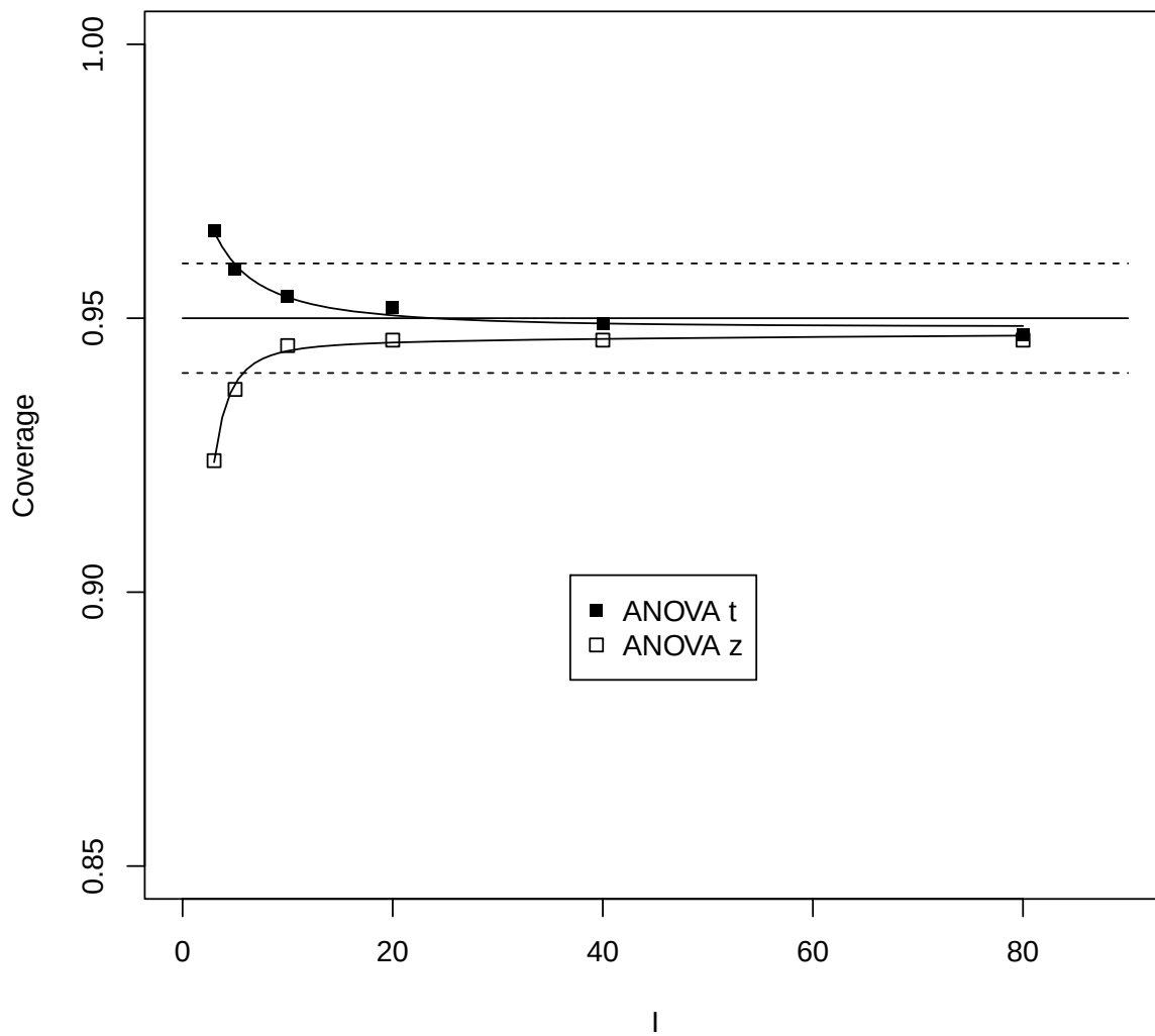
Figure 37: Simulation coverages of ANOVA t and ANOVA z nominal 95% confidence intervals, \rho = 0.80 , J = 3 . Dotted lines at 0.94 and 0.96.
