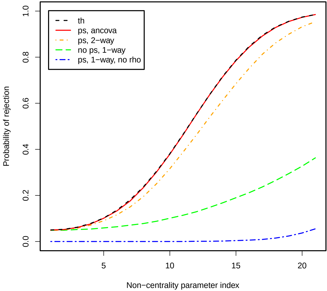
Figure 27: Power plot, \rho = 0.9 , J = 5 , I = 10 .
