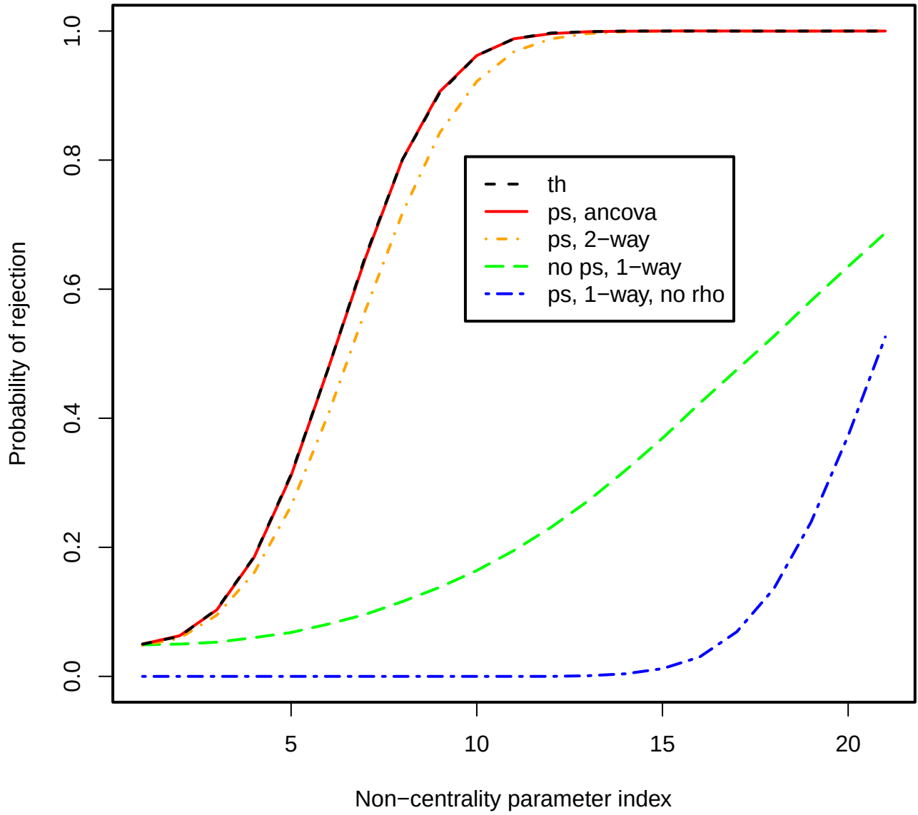
Figure 30: Power plot, \rho = 0.95 , J = 5 , I = 20 .
