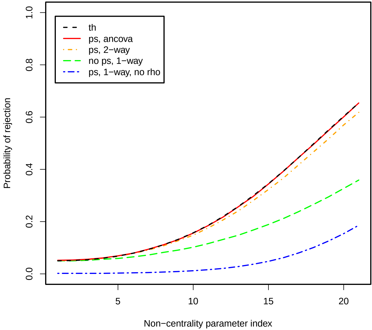
Figure 23: Power plot, \rho = 0.7 , J = 5 , I = 10 .
