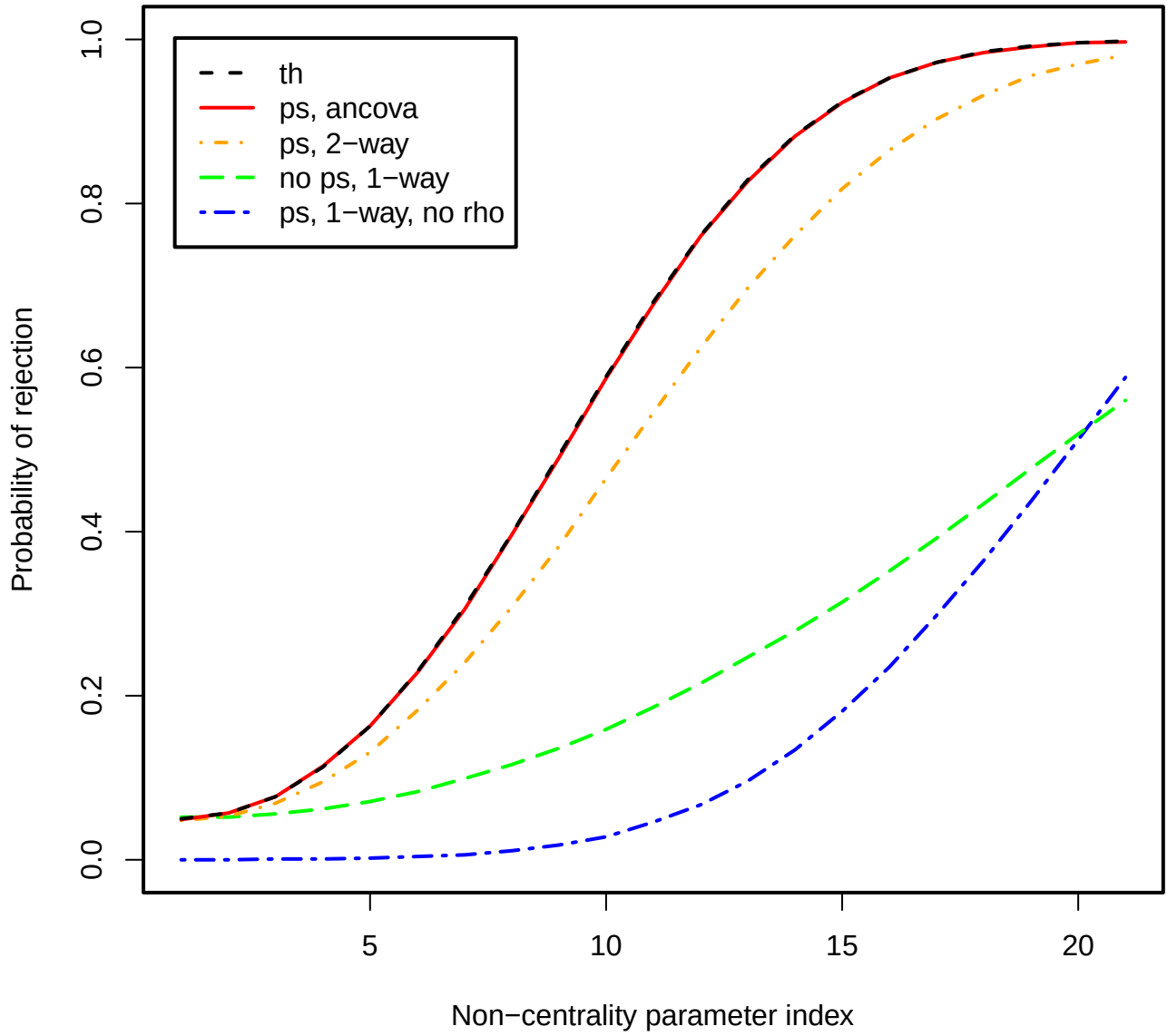
Figure 11: Power plot, \rho = 0.9 , J = 2 , I = 10 .
