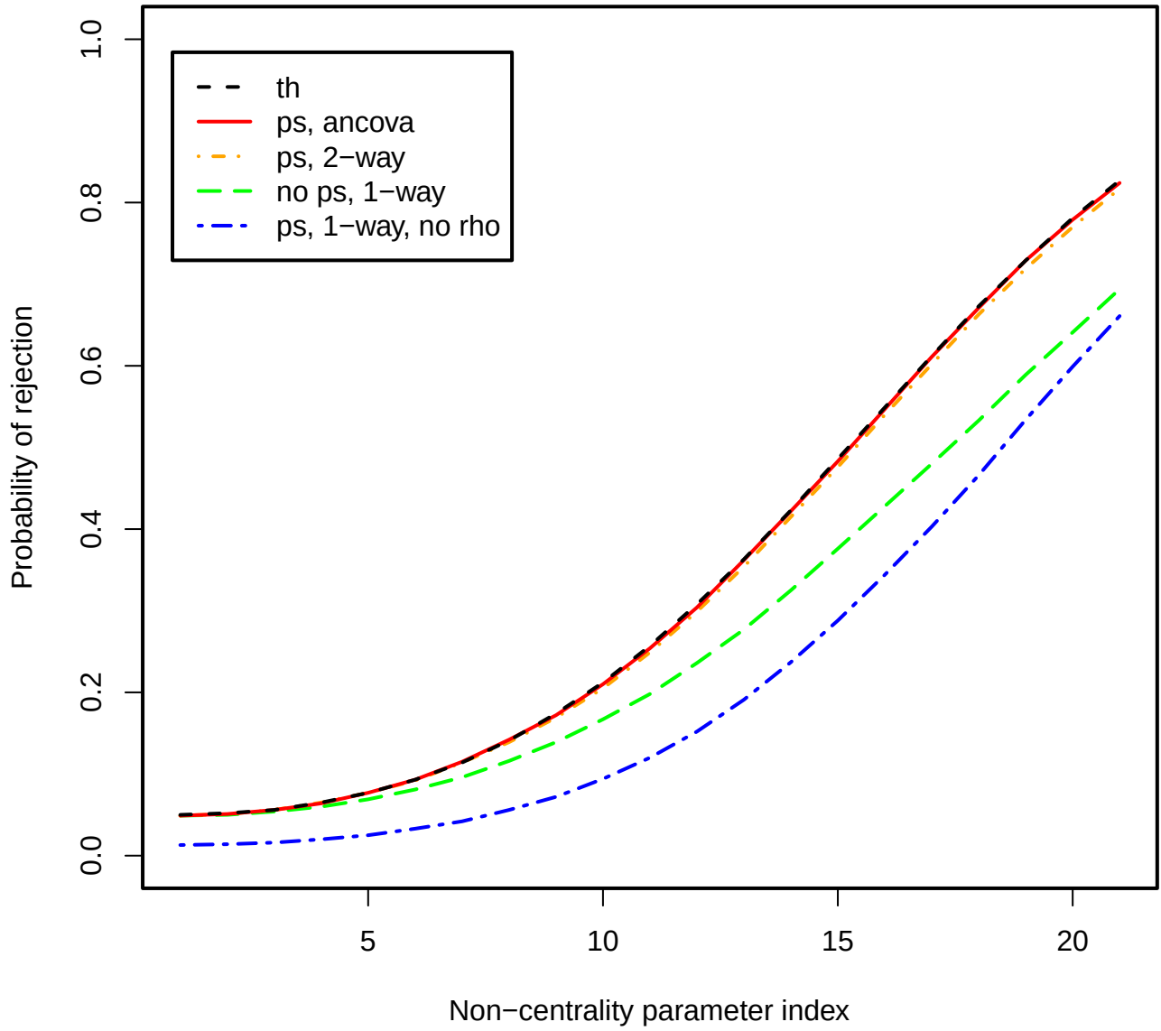
Figure 20: Power plot, \rho = 0.5 , J = 5 , I = 20 .
