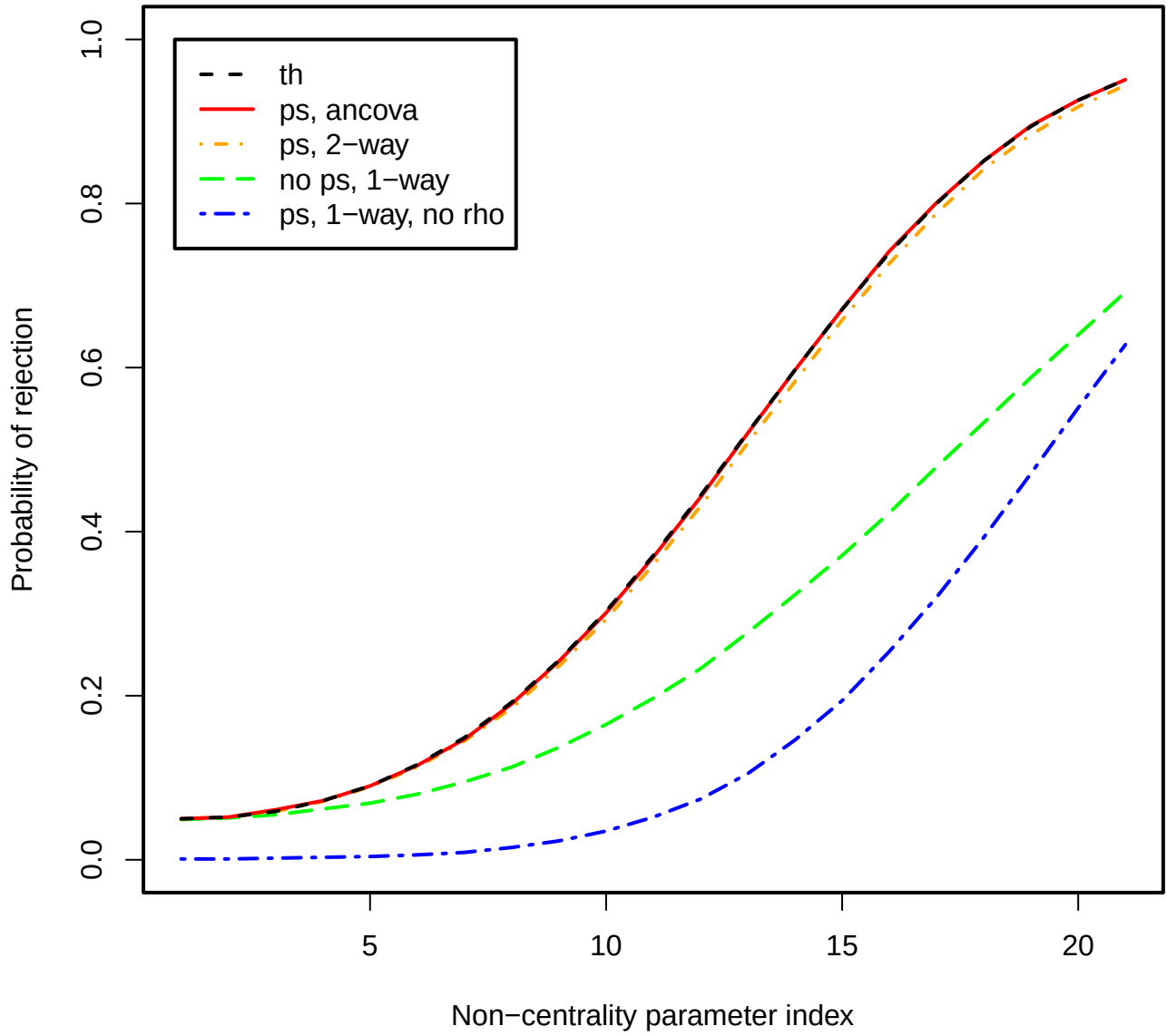
Figure 24: Power plot, \rho = 0.7 , J = 5 , I = 20 .
