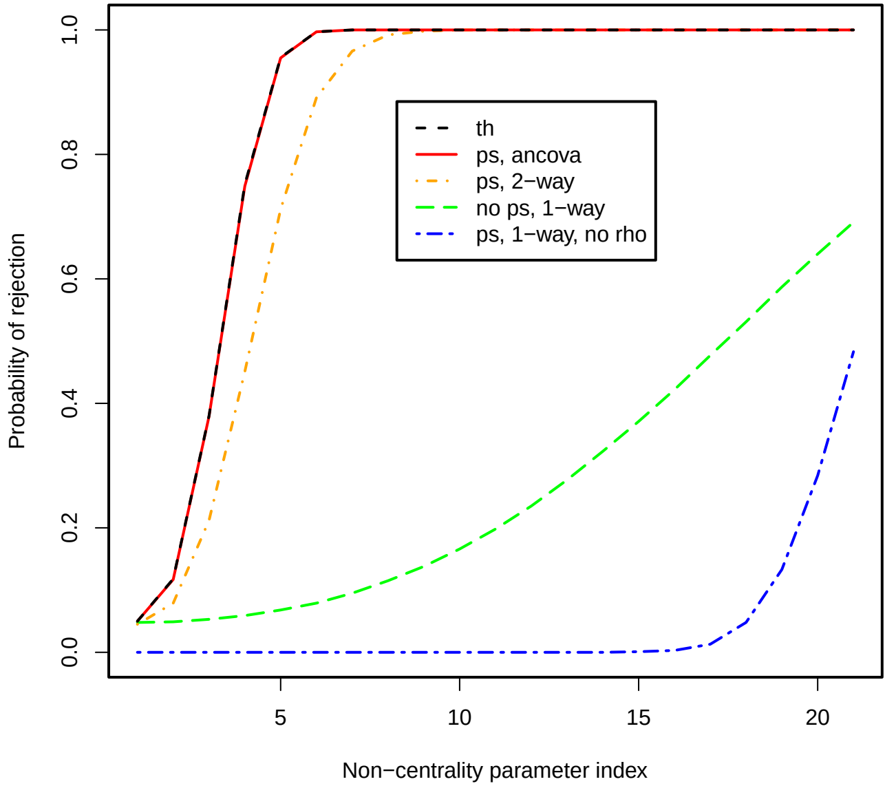
Figure 32: Power plot, \rho = 0.99 , J = 5 , I = 20 .
