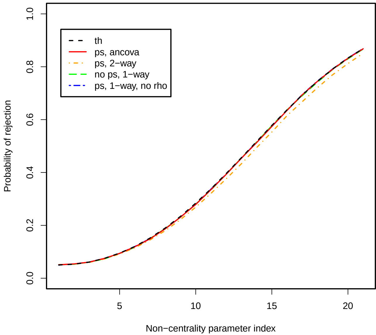
Figure 2: Power plot, \rho = 0.0 , J = 2 , I = 20 .
