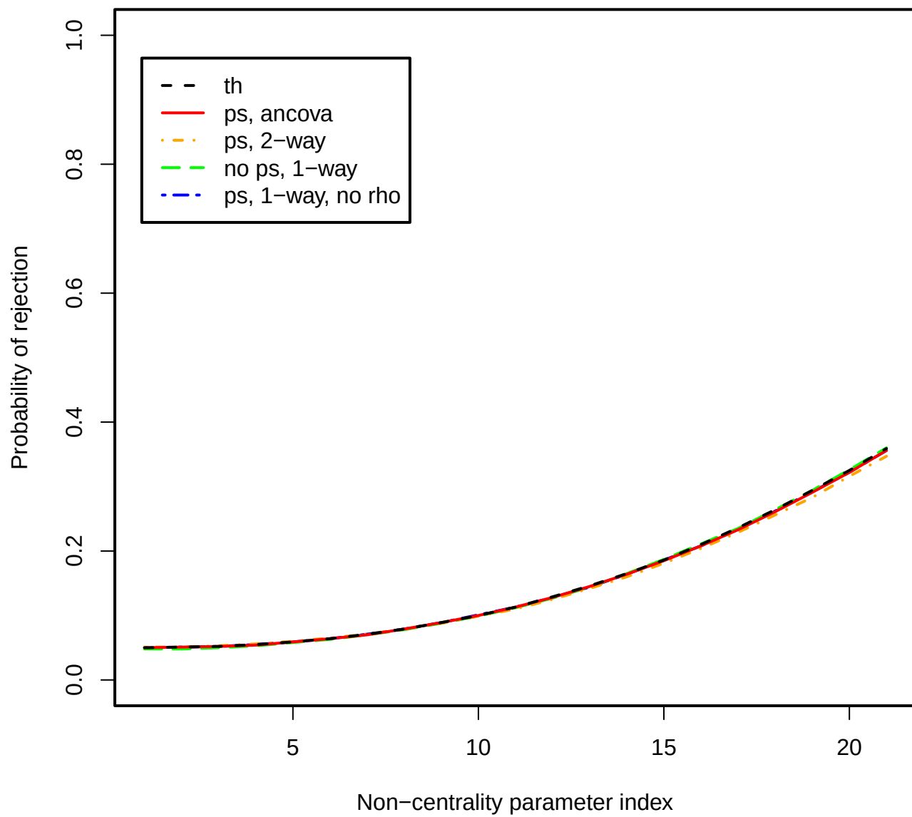
Figure 17: Power plot, \rho = 0.0 , J = 5 , I = 10 .
