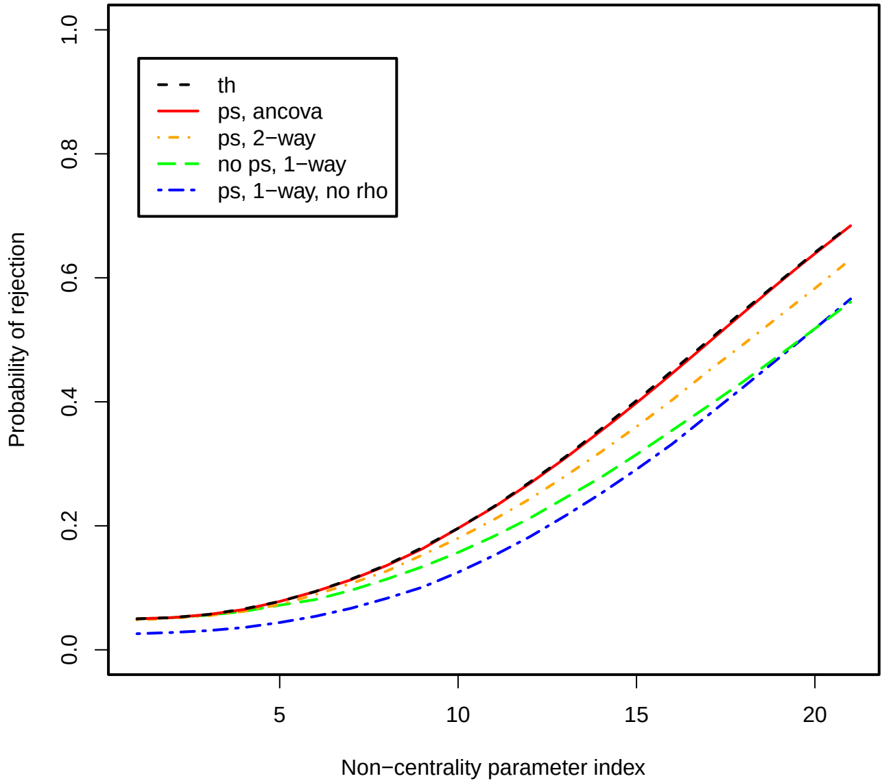
Figure 3: Power plot, \rho = 0.5 , J = 2 , I = 10 .
