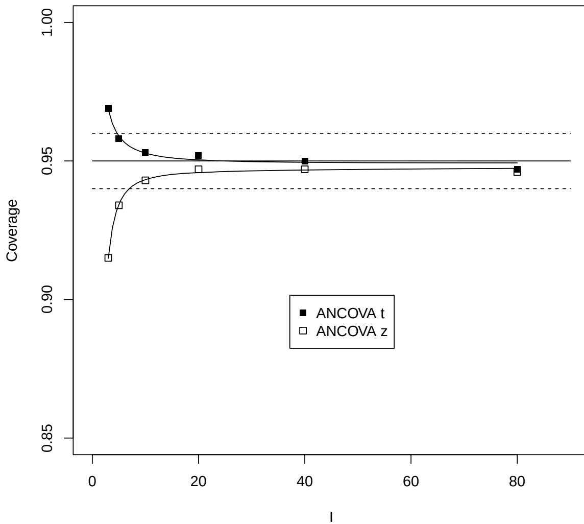
Figure 38: Simulation coverages of ANCOVA t and ANCOVA z nominal 95% confidence intervals, \rho = 0.80 , J = 3 . Dotted lines at 0.94 and 0.96.
