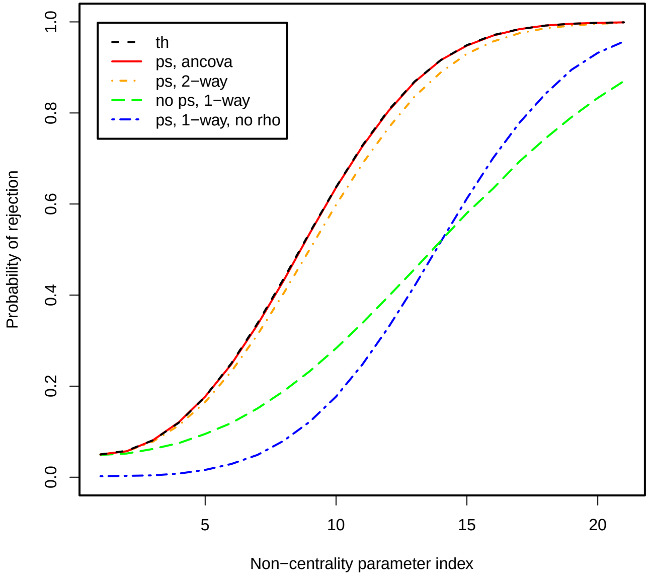
Figure 10: Power plot, \rho = 0.8 , J = 2 , I = 20 .
