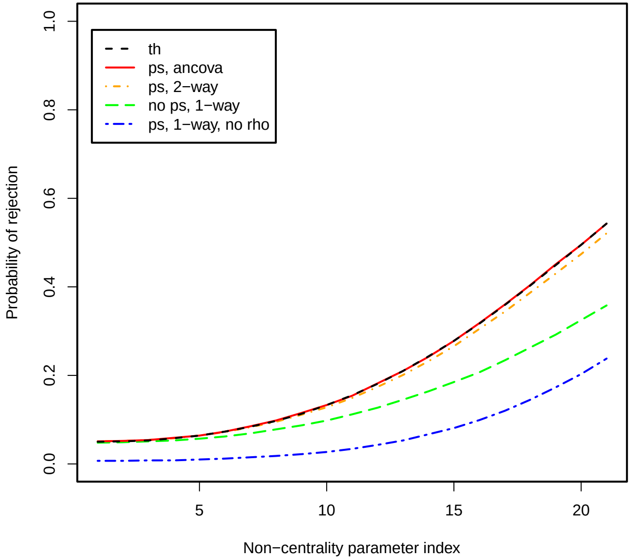
Figure 21: Power plot, \rho = 0.6 , J = 5 , I = 10 .
