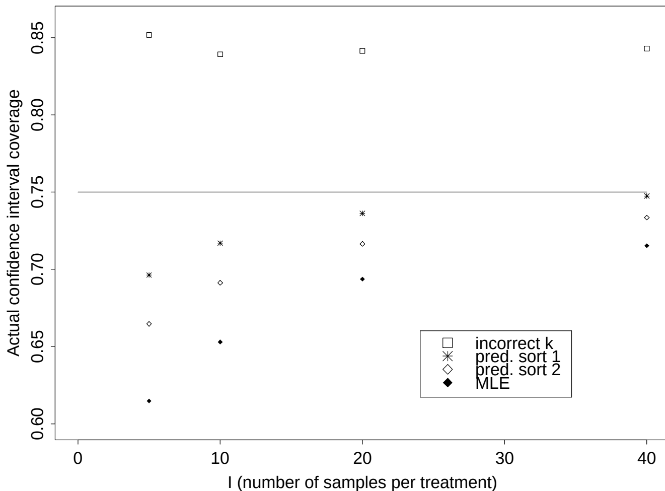
Figure 39: Approach of actual confidence interval coverage to nominal (0.75) coverage as sample size increases. For this figure, the correlation between the predictor and the response was 0.85. The number of treatments, J , was four. The confidence interval was for the 0.01 quantile. (See table 2 in Verrill et al. 2004.)
