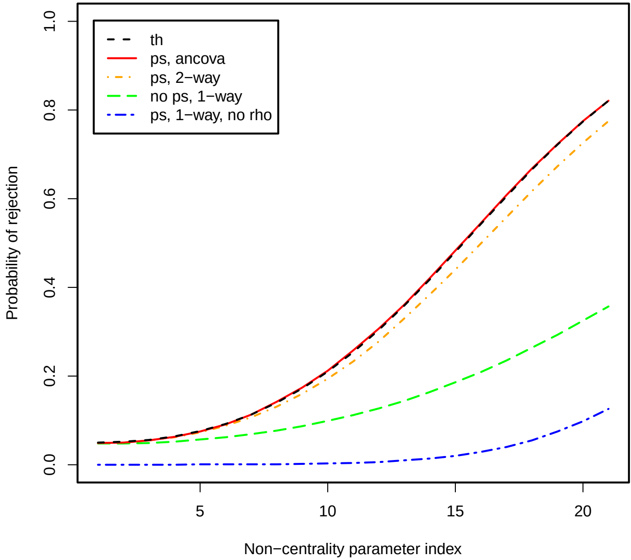
Figure 25: Power plot, \rho = 0.8 , J = 5 , I = 10 .
