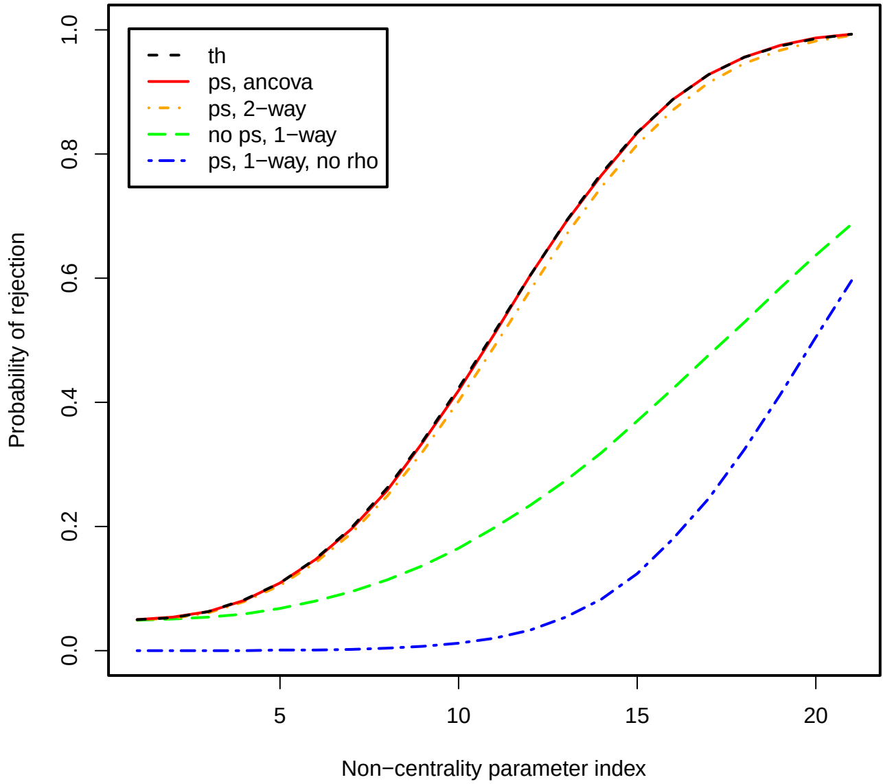
Figure 26: Power plot, \rho = 0.8 , J = 5 , I = 20 .
