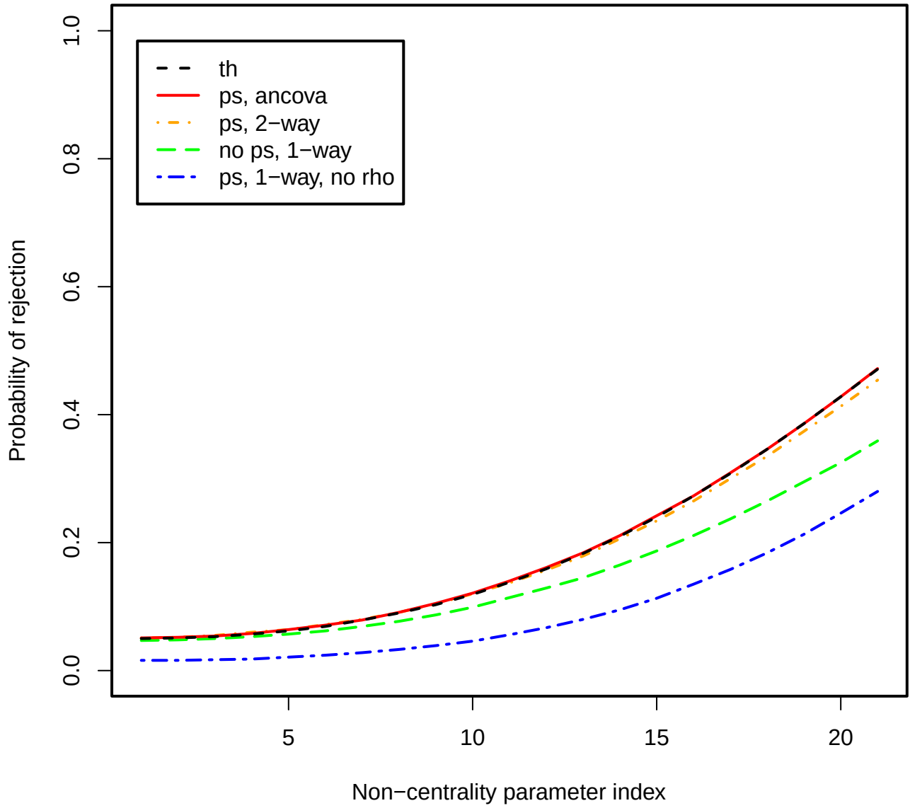
Figure 19: Power plot, \rho = 0.5 , J = 5 , I = 10 .
