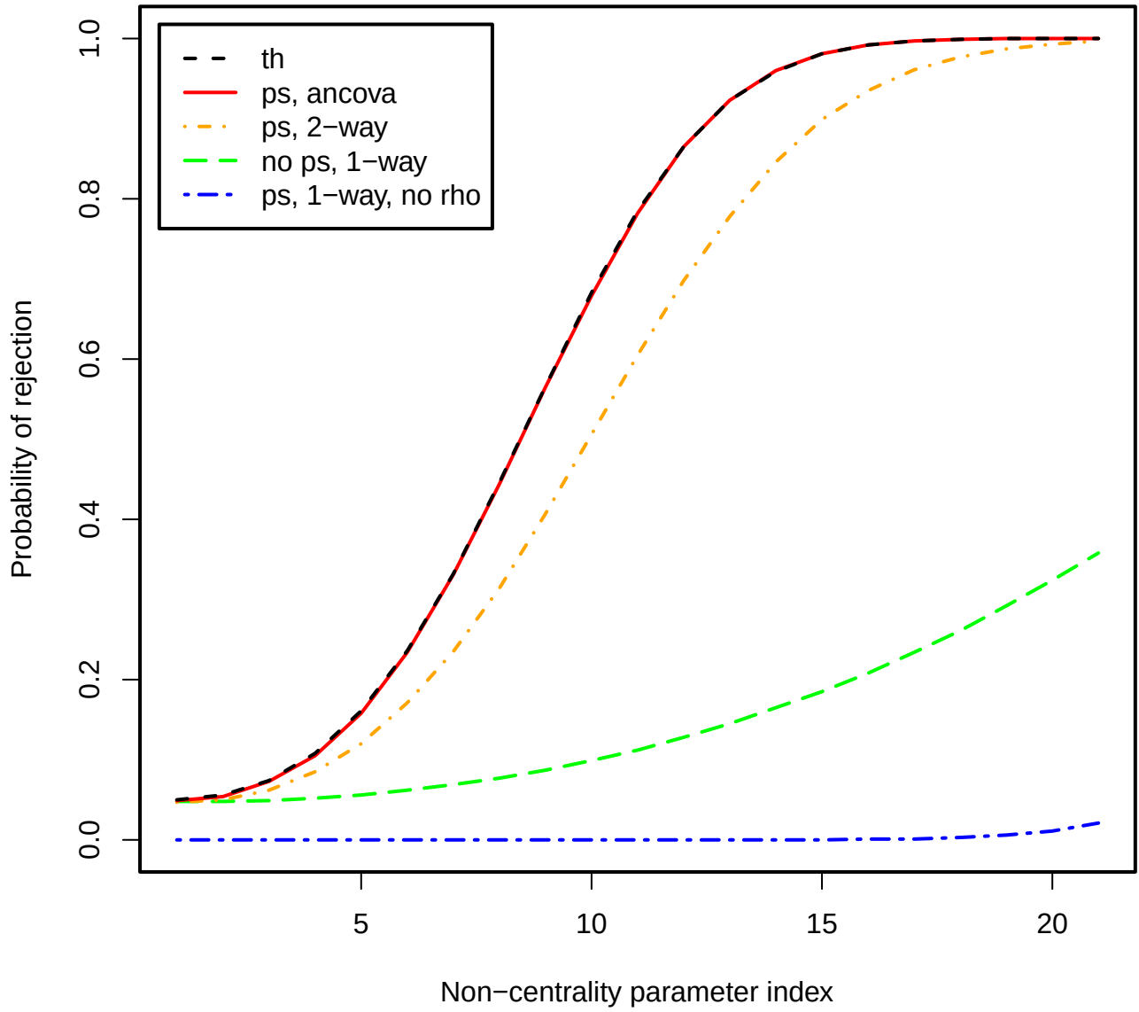
Figure 29: Power plot, \rho = 0.95 , J = 5 , I = 10 .
