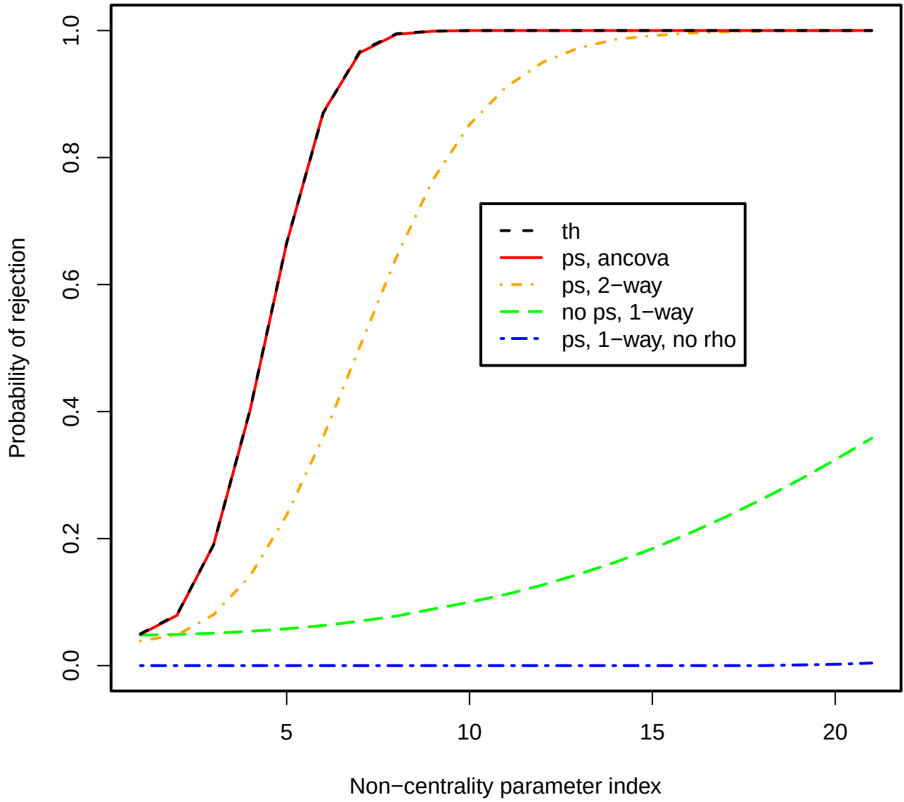
Figure 31: Power plot, \rho = 0.99 , J = 5 , I = 10 .
