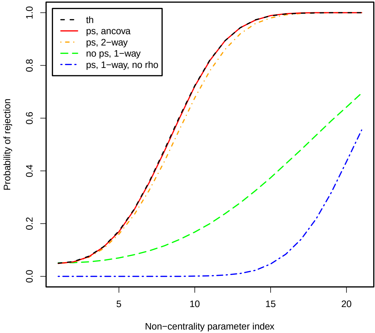
Figure 28: Power plot, \rho = 0.9 , J = 5 , I = 20 .
