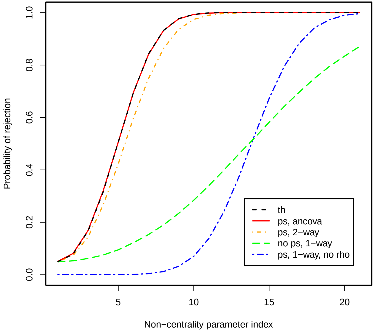
Figure 14: Power plot, \rho = 0.95 , J = 2 , I = 20 .
