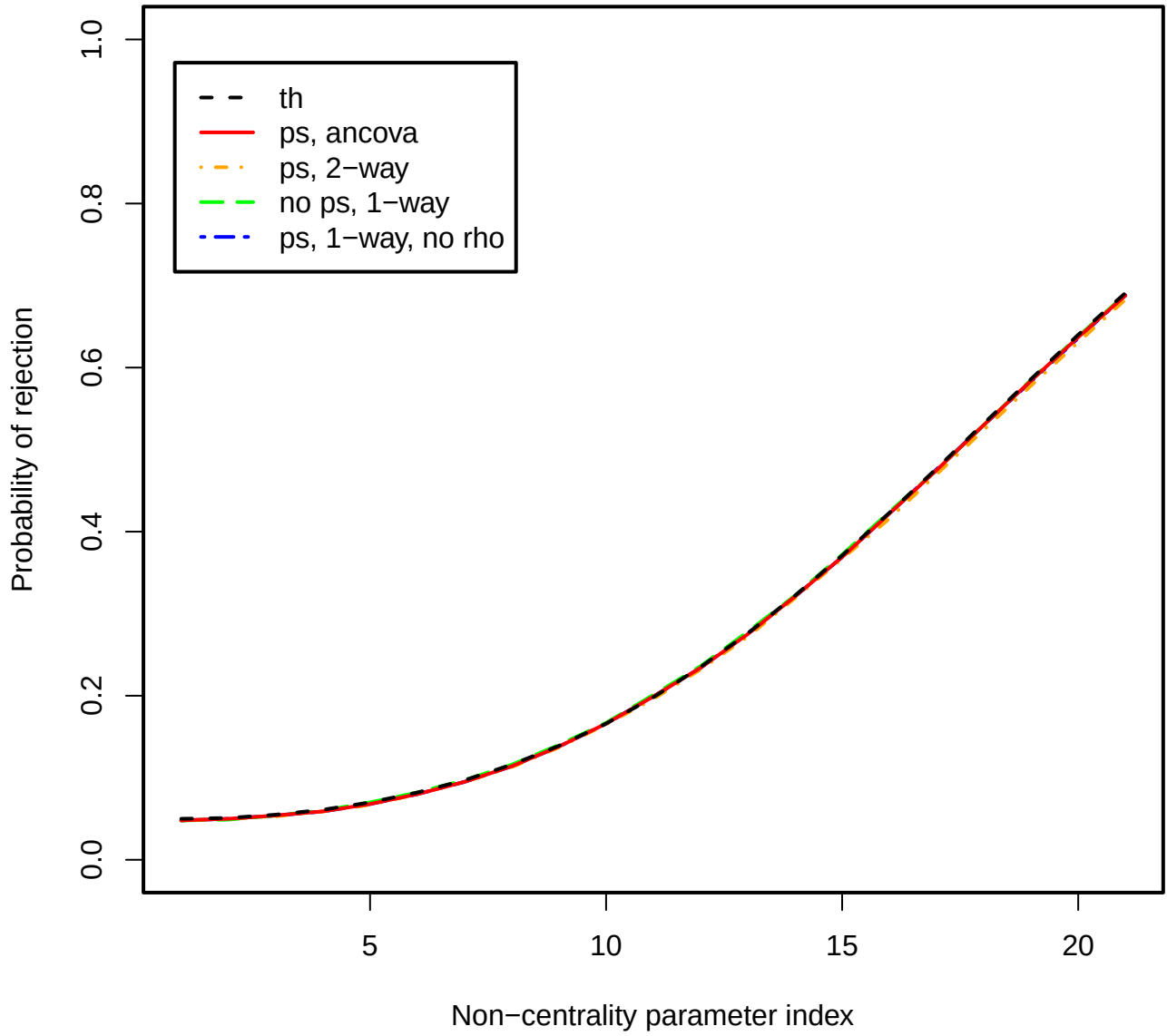
Figure 18: Power plot, \rho = 0.0 , J = 5 , I = 20 .
