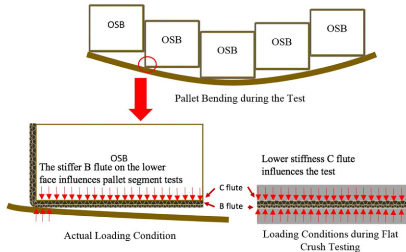
Figure 5. Compression of the bottom of the corrugated box during actual loading conditions and during flat crush testing.
