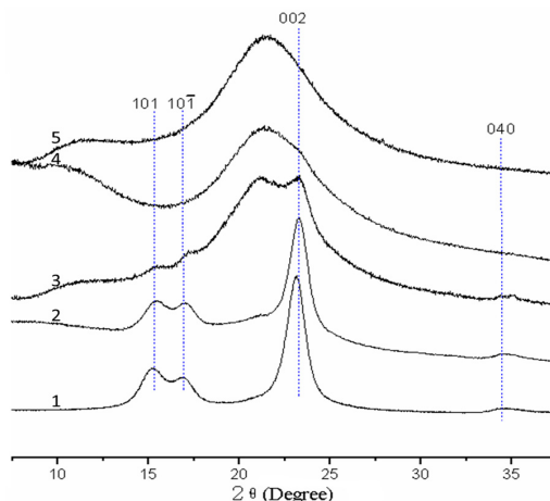
Figure 5. X-ray diffraction spectra of unmodified (spectrum 1) cellulose and succinylated cellulose prepared with the W_{\text{TBA}} at 5.0 wt% (spectrum 2), 7.5 wt% (spectrum 3), 10.0 wt% (spectrum 4), and 12.5 wt% (spectrum 5).
