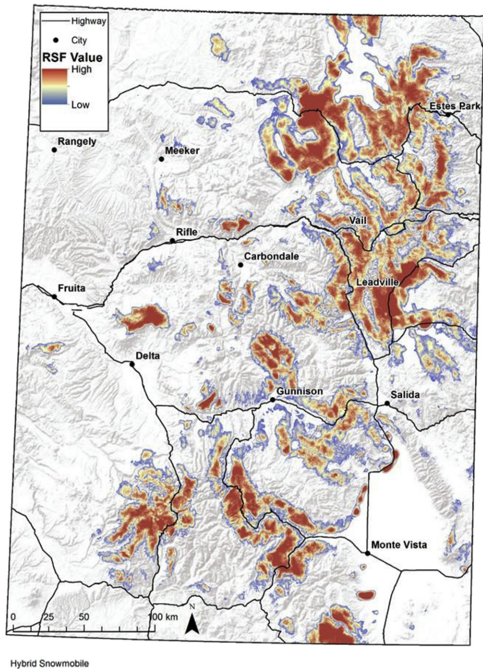
Figure C.3. Predicted probabilities of selection from the resource selection function model for hybrid snowmobile recreation across western Colorado. Warm colors indicate higher probability of selection, cool colors indicate an area is less likely to be selected.
