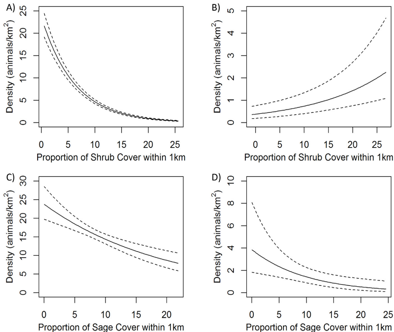
Fig 3. Modeled response of density (individuals/km 2 ) of small mammal species groups to proportion of shrub or sagebrush cover. Top panels show proportion of shrub cover, bottom panels show proportion of sagebrush cover; dotted lines show 95% confidence intervals. Panel A) shows white-tailed prairie dogs, B) least chipmunks, C) Wyoming ground squirrels, and D) leporids ( Sylvilagus sp. and Lepus townsendii ).
