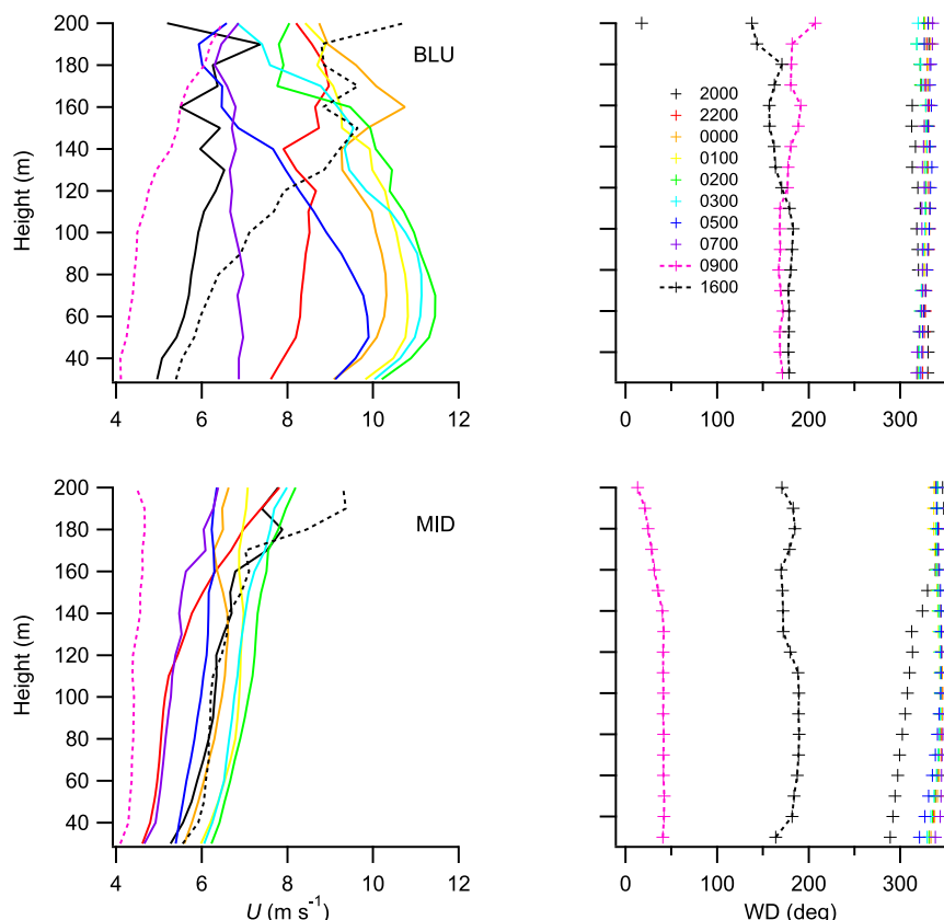
FIG. 12. Average hourly vertical profiles of sodar (left) wind speed and (right) direction for THRM GAP at BLU and MID with emphasis between evening and morning transitions. The start times (MST) for each hour interval are shown in the legend.
