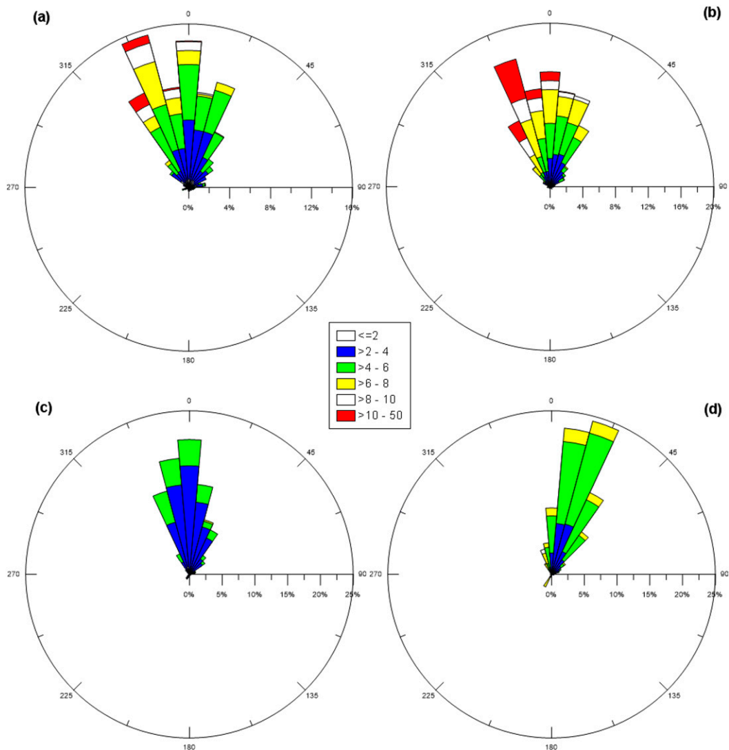
FIG. 17. Wind roses ( \text{m s}^{-1} ) from SMC for THRM (a),(b) GAP and (c),(d) non-GAP cases at the 15- and 45-m levels, respectively, using 5-min-average data showing the effects of BCV GAP category flows out on the SRP between 0000 and 0500 h MST.
