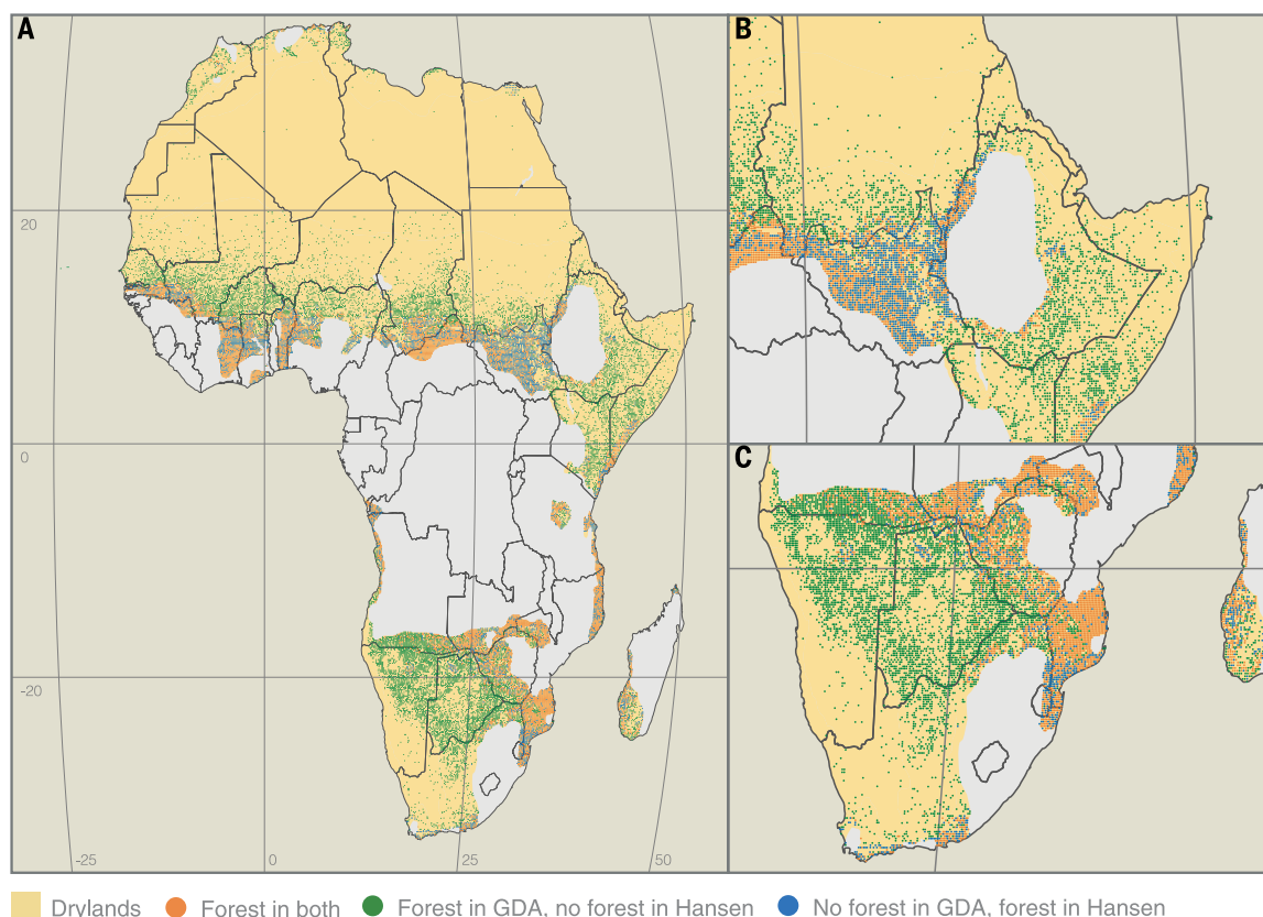
Fig. 2. Comparison of \geq 10\% tree cover in Africa's drylands.
