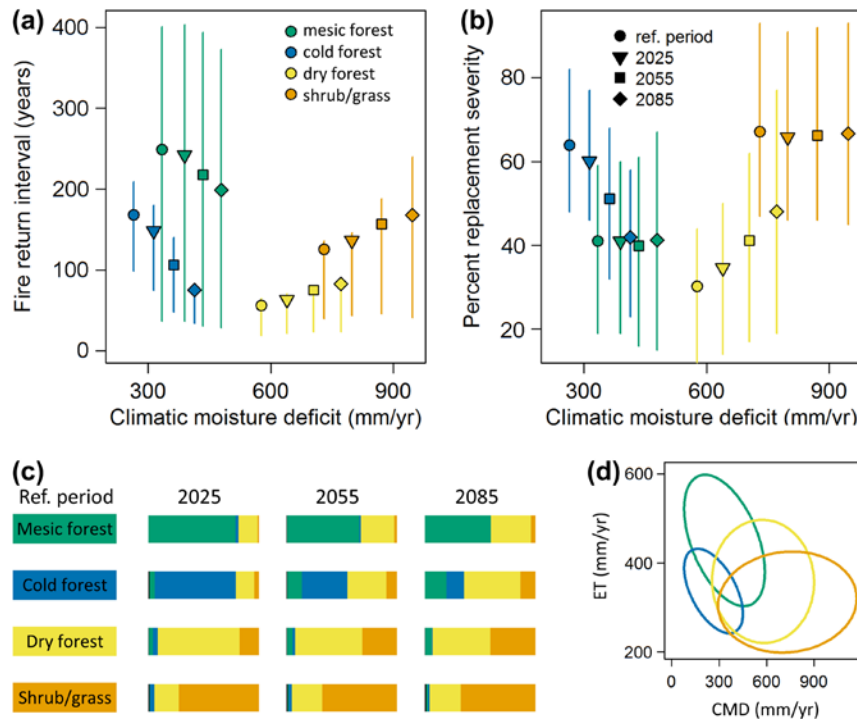
Figure 5. Plots describe (a) the fire return interval (FRI) and (b) percent replacement severity (PRS) for four vegetation groups for four time periods (see Methods) along the climatic moisture deficit gradient. The symbols (e.g. open circles) represent the mean values and the vertical lines show the inter-quartile range for FRI and PRS for reference and future time periods. The CMD values are representative of each time period (this is in contrast to the static CMD axis in Fig. 3). (c) Bar plots show the four reference period vegetation groups and the vegetation associated with incoming climates of each group; widths represent the relative proportion of each group. (d) Ellipses encapsulate 67% of data depicting the reference period climate space (in terms of climatic moisture deficit [CMD] and evapotranspiration [ET]) of each vegetation group; note the large amount of overlap between dry forest and shrubland/grassland. The sparse/barren vegetation class is excluded in this figure because it comprises only ~1% of the study area.
