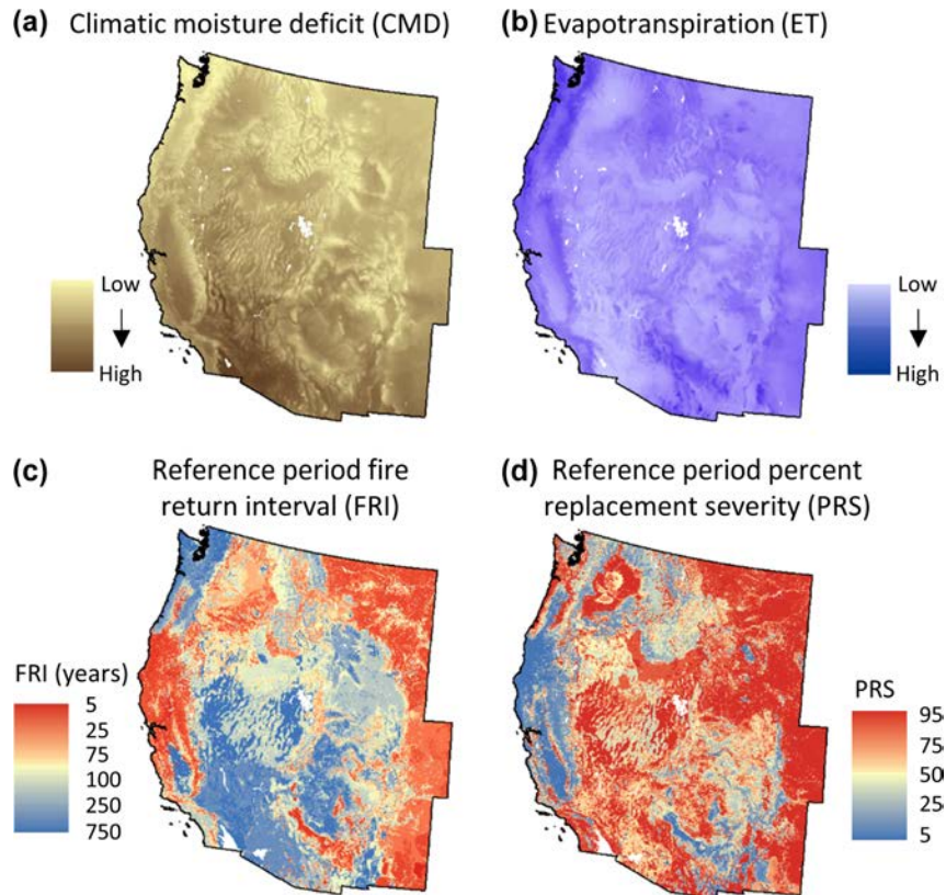
Figure 2. Maps show (a) the climatic moisture deficit (CMD) and (b) evapotranspiration (ET) for the western contiguous US. These climate variables represent the 1961–1990 time period and were used to define and identify climate analogs. Maps show (c) the mean fire return interval (FRI) and (d) percent replacement severity (PRS) (Rollins 2009; < www.landfire.gov >). Because climate analogs (and the associated fire regimes and vegetation) may be located outside of the ecoregions of interest, these maps show the extent of the western contiguous US.
