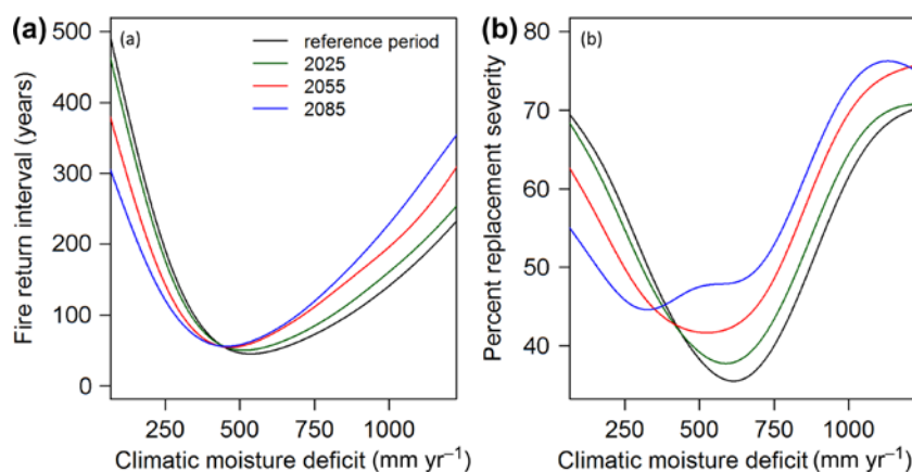
Figure 3. Fitted splines describe (a) the fire return interval (FRI) and (b) percent replacement severity (PRS) for reference and future time periods as a function of the climatic moisture deficit (CMD) for mountainous ecoregions in the western US. The climatic moisture deficit (x-axis) is static and is representative of the reference period climate (1961–1990).
