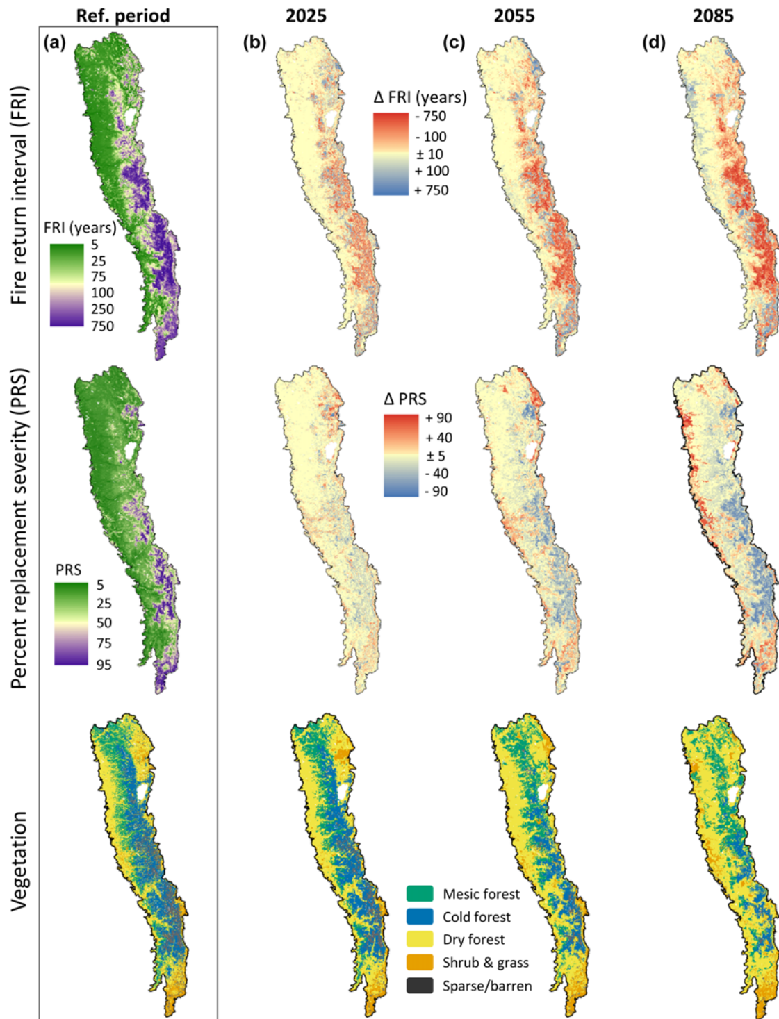
Figure 4. Maps show reference period fire return interval (FRI), percent replacement severity (PRS), and vegetation for the Sierra Nevada ecoregion (a). Also shown are changes in FRI, changes in PRS, and vegetation for three future time periods, 2025 (b), 2055 (c), and 2085 (d). See Fig. 1 to reference the location of this ecoregion.
