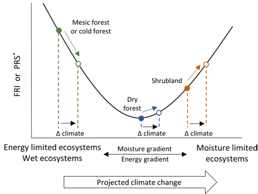
Figure 6. Conceptual model describing predicted climate-induced shifts in fire return interval (FRI) and percent replacement severity (PRS) along a resource gradient representing moisture and energy. As the climate warms, mesic forests and cold forests are expected to experience decreased FRI and PRS*. Dry ecosystems, such as shrubland/grassland, are expected to experience increased FRI, which is likely in response to decreased productivity and available biomass. Dry forests, especially those on the ecotone between forest and non-forest, are predicted to experience increased FRI and PRS, which may be an indication of transition from forest to non-forest. Note that climatic moisture deficit is projected to increase across the entire western US in coming decades (data not shown) (Wang et al. 2016). *Note that mesic forest and shrubland/grassland did not exhibit predicted decreases and increases in PRS, respectively (Fig. 5).
