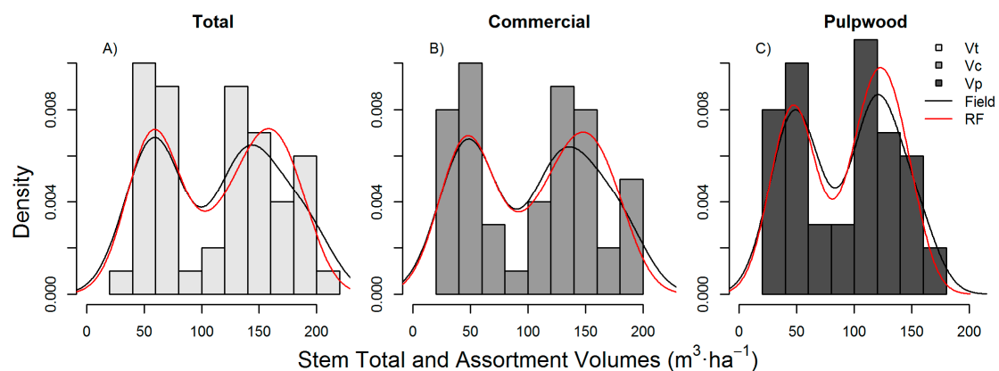
Figure 4. Distribution of observed (black line) and predicted (red line) stem volume from RF. The gray histograms is based from field data. (A) Total volume (Vt) (B) Commercial volume (Vc) and (C) Pulpwood volume (Vp).
