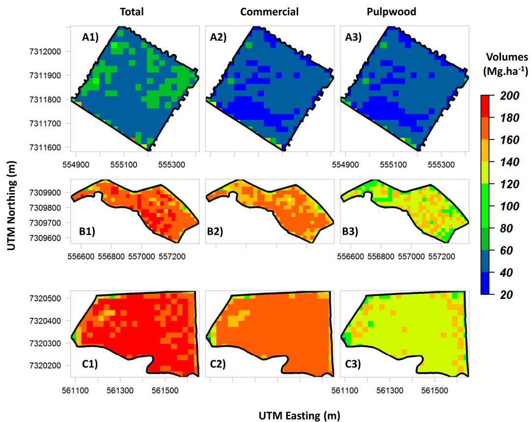
Figure 7. Predicted V_t (A1–C1), V_c (A2–C2) and V_p (A3–C3) of P. taeda at stand-level obtained from the RF models. Representative stand of early (i.e., 3–5 years) (A1–3), intermediate (i.e., 5–7 years) (B1–3) and advanced-stages of development (i.e., 7–9 years) (C1–3).
