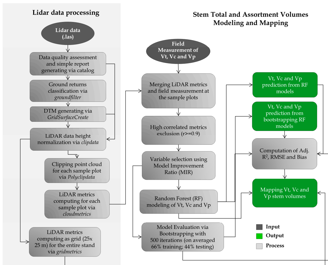
Figure 3. Procedure for predicting stem total and assortment volumes in an industrial P. taeda forest plantation using airborne laser scanning data and random forest.
