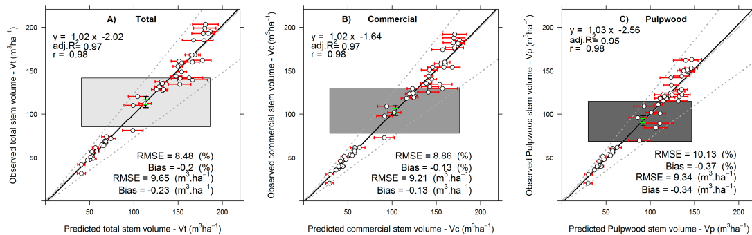
Figure 5. Equivalence plots of the observed and the mean of predicted Vt (A), Vc (B) and Vp (C) obtained from the 500 bootstrapped RF model runs. ( N = 50 ). The equivalence plot design presented herein is an adaptation of the original equivalence plots presented by [41]. The grey polygon represents the \pm 25\% region of equivalence for the intercept, and the green vertical bar represents a 95% of confidence interval for the intercept. The predicted stem volumes from the RF models are equivalent with reference to the intercept and slope since the green bar is completely within the grey polygon. If the grey polygon is lower than the green vertical bar, the predicted stem volumes are negatively biased; and if it is higher than the green vertical bar, the predicted stem volumes are positively biased. Moreover, the grey dashed line represents the \pm 25\% region of equivalence for the slope, the fit line is within the dotted lines and the black vertical bar is within the gray rectangle, indicating that the pairwise measurements are equivalent. A green bar that is wider than the region outlined by the grey dashed lines indicates highly variable predictions. The white dots are the pairwise measurements, and the solid line is a best-fit linear model for the pairwise measurements. The light grey dashed line represented the relationship 1:1. The horizontal red bars represent the standard deviation of the 500 bootstrapping predictions.
