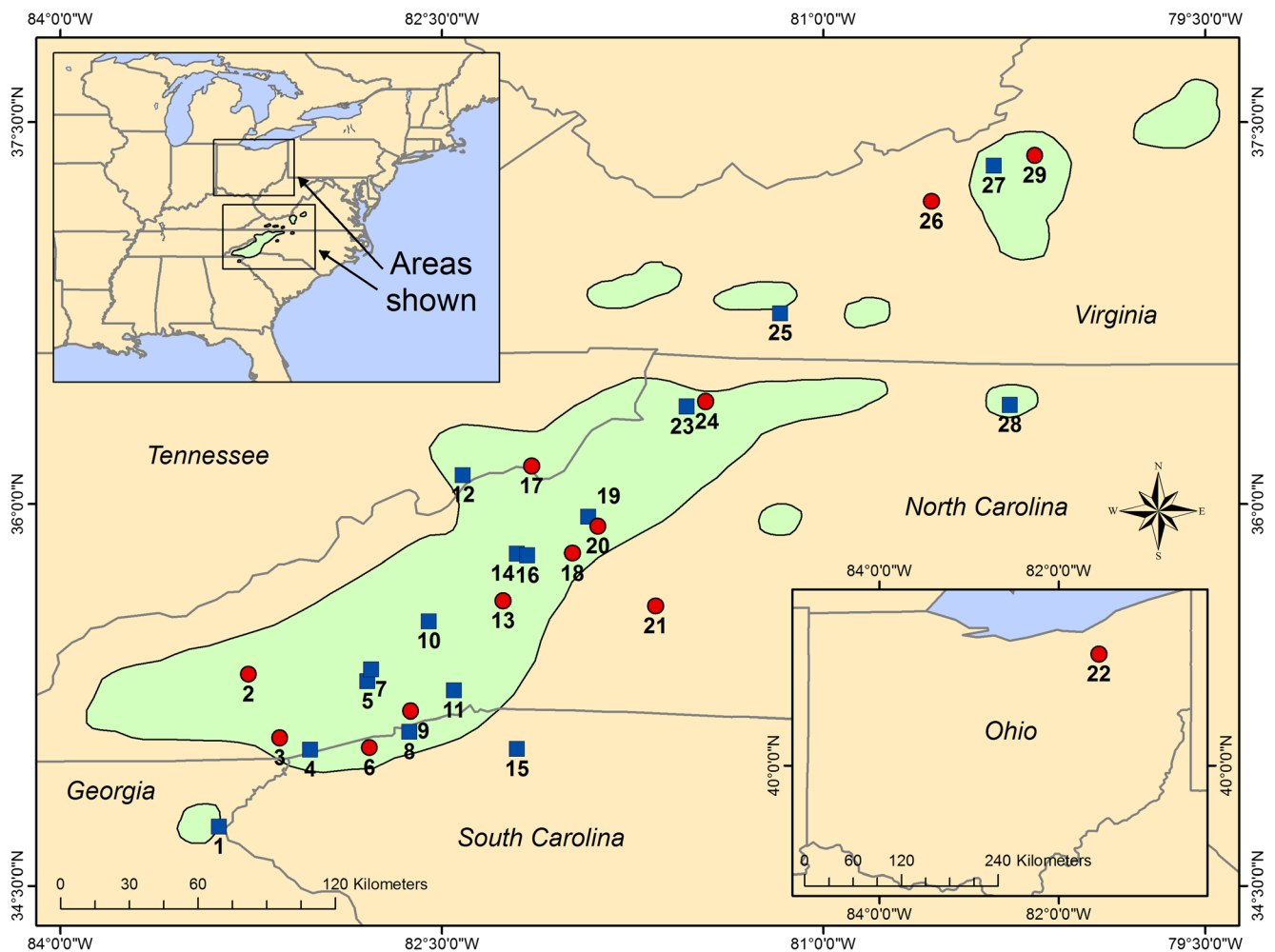
Fig. 1 Sampled populations of Carolina hemlock ( Tsuga caroliniana ). See Table 1 for population information. Blue populations (squares) are those for which collections of seed for gene conservation have been conducted. Seed had not been collected from red populations (circles) as of summer 2015
