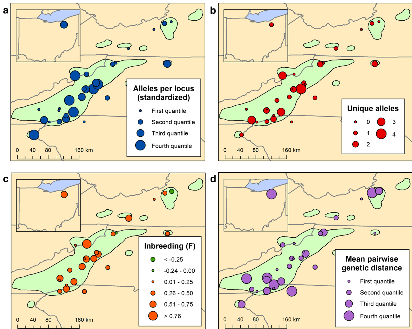
Fig. 2 Carolina hemlock population classifications of a alleles per locus ( A ), b unique alleles ( A_U ), c inbreeding coefficient ( F_{IS} ), and d mean pairwise chord distance ( D_C ), based on 16 polymorphic nuclear microsatellite loci
