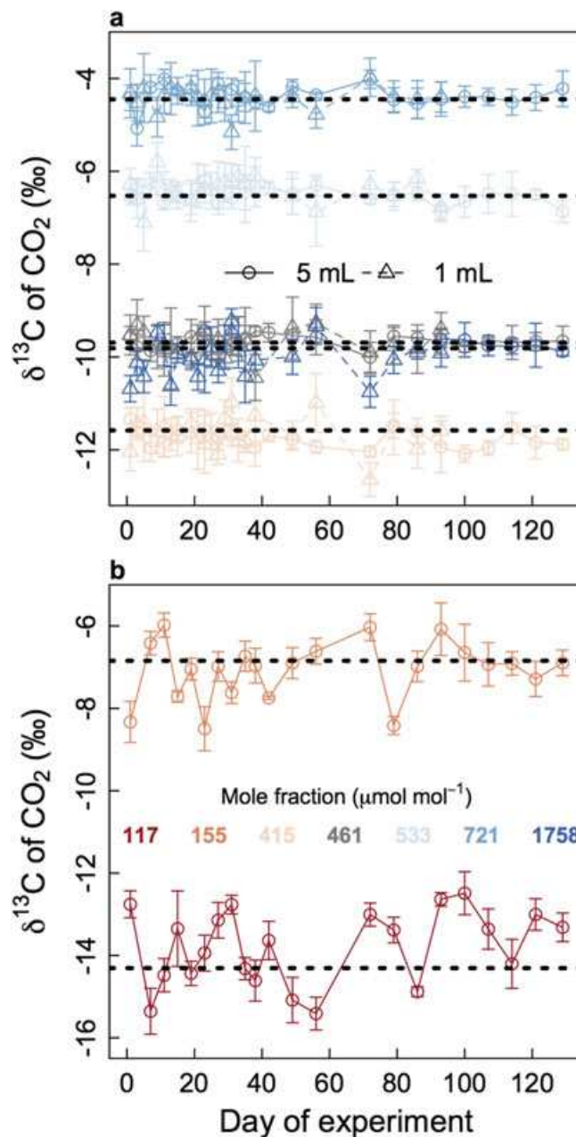
FIGURE 3 Values of \delta^{13}\text{CO}_2 in standards measured as unknowns over a period of 129 days, with 1- and 5-mL injections denoted by triangles and circles, respectively. Colors indicate \text{CO}_2 mole fractions for each time standard (117–1758 \mu\text{mol mol}^{-1} ) as indicated in the legend, from red (lower concentration) to tan-grey (intermediate) to blue (higher concentration). The dotted lines indicate the known \delta^{13}\text{CO}_2 values for each standard. Standards with [\text{CO}_2] < 400 \mu\text{mol mol}^{-1} had greater variability and are shown in B [Color figure can be viewed at wileyonlinelibrary.com ]
