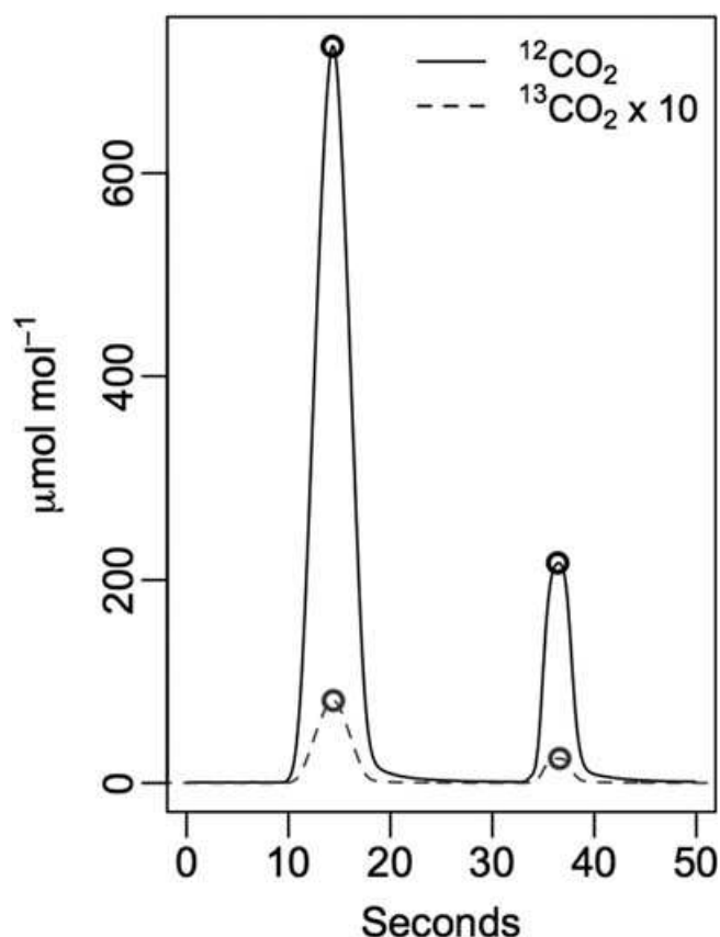
FIGURE 1 Peaks for ^{12}\text{CO}_2 and ^{13}\text{CO}_2 measured on the TGA200A following injection of 5- and 1-mL samples of a standard gas (720.8 \mu\text{mol mol}^{-1} \text{CO}_2 ), respectively. The trace for ^{13}\text{CO}_2 was multiplied 10-fold for clarity. Circles represent peak heights (local maxima) used to independently calibrate ^{12}\text{CO}_2 and ^{13}\text{CO}_2 for calculations of \delta^{13}\text{C} values and [\text{CO}_2] during post-processing
