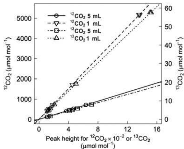
FIGURE 2 Relationships between the peak heights of ^{12}\text{CO}_2 and ^{13}\text{CO}_2 and the known values. The solid line is the linear regression line for ^{12}\text{CO}_2 measurements from 5-mL injections: y = 1.13x - 2.07 . The dashed line is for ^{12}\text{CO}_2 measurements from 1-mL injections: y = 3.79x + 7.02 . The dot-dashed line is for ^{13}\text{CO}_2 measurements from 5-mL injections: y = 1.12x - 0.02 . The dotted line is for ^{13}\text{CO}_2 measurements from 1-mL injections: y = 3.79x + 0.09
