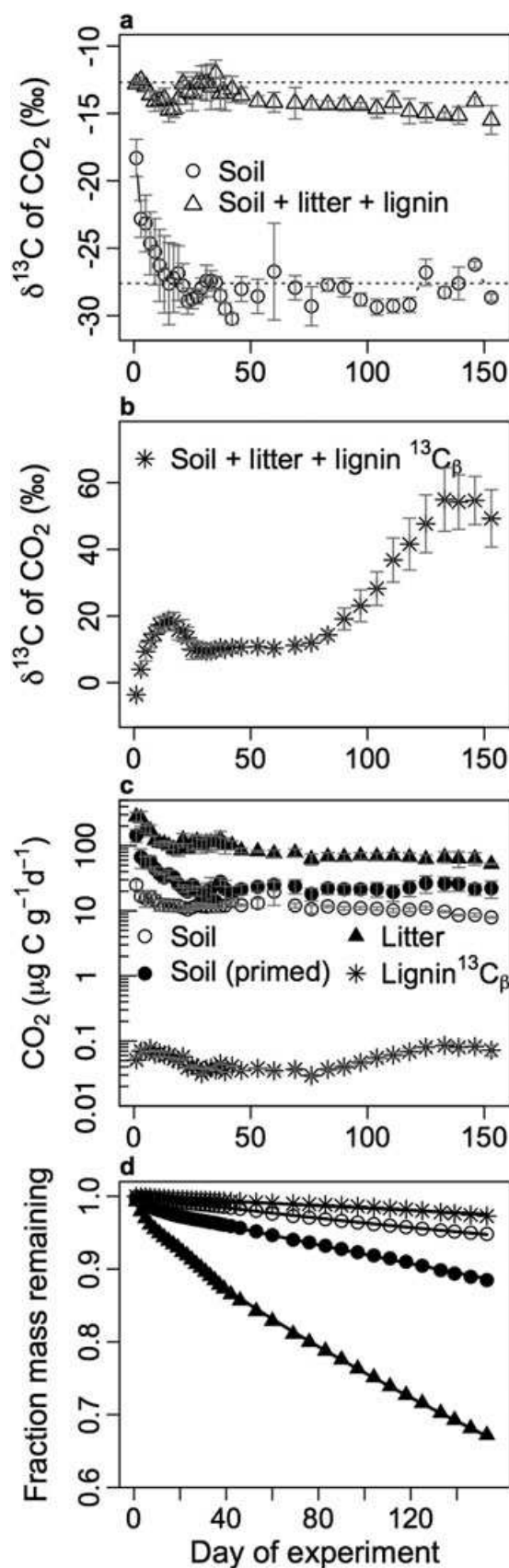
FIGURE 4 Temporal trends in \delta^{13}\text{C} values of \text{CO}_2 from soil incubation treatments (A, B), contributions of litter, SOM, and lignin ^{13}\text{C}_\beta to respiration (C), and cumulative mass loss and model fits indicated by lines (D). Error bars are standard errors ( n = 3 ), but are not included in (D) for clarity. Soil (primed) denotes \text{CO}_2 production from SOM in the treatment that received added litter
