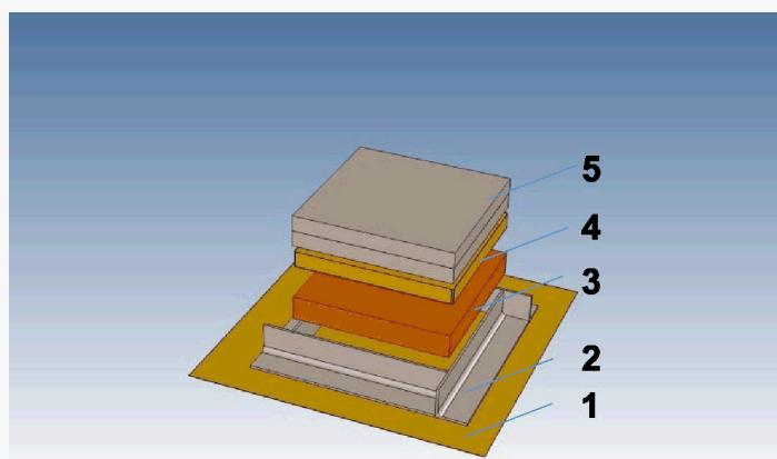
Fig. 2. Diagram of mat hot-pressing setup: 1) bottom caul and screen, 2) aluminum frame, 3) fiber mat, 4) top screen, and 5) two aluminum blocks
