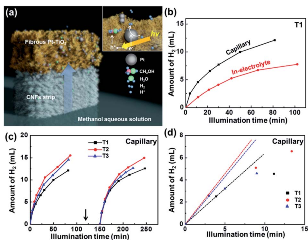
Fig. 4 (a) Schematics of the novel capillary design by using the CNF block for photocatalytic \text{H}_2 evolution. (b) \text{H}_2 yield of 3D nanofibrous Pt- \text{TiO}_2 sample T1 from both capillary design (black) and in-electrolyte design (red). (c) \text{H}_2 yield of three Pt- \text{TiO}_2 photocatalyst samples (T1, T2, and T3) versus illumination time in the capillary design. The curve after the electrolyte renewal and whole system purging indicates a good stability of the capillary setup for photocatalytic reactions. (d) Magnified \text{H}_2 evolution curves of the first 15 min in the presence of T1, T2 and T3 photocatalysts. Derived initial \text{H}_2 production rates were calculated by the indicated dashed lines.
