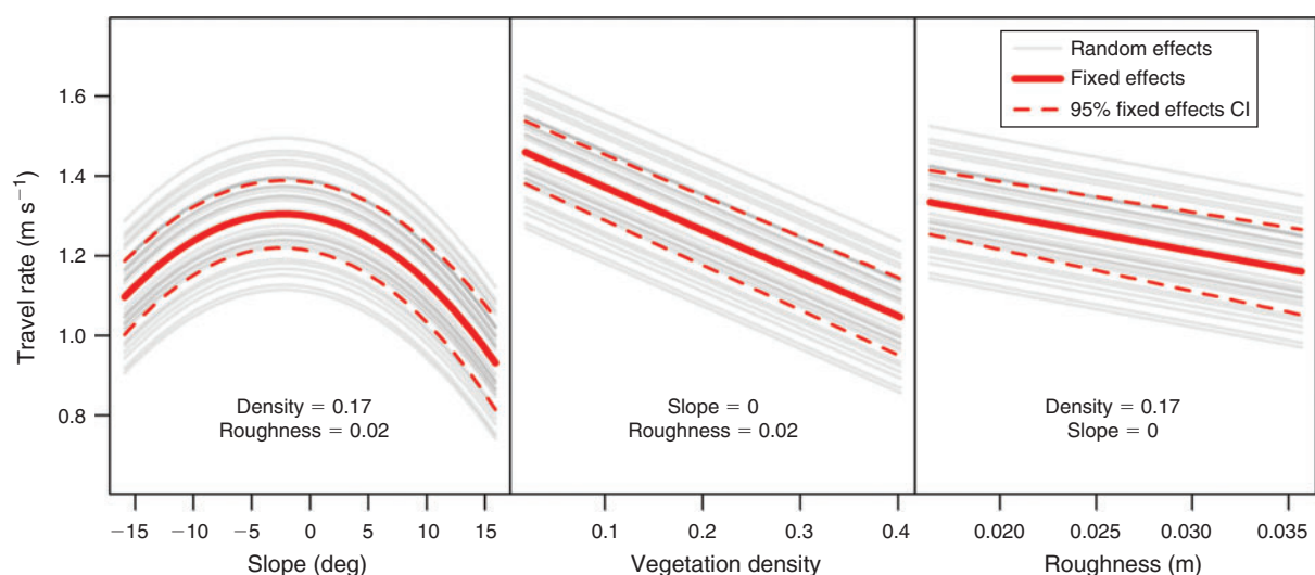
Fig. 7. Predicted results of linear mixed effects regression (LMER) for each landscape condition within the range of values found on transects throughout the study area, assuming a median value of the other two conditions.
