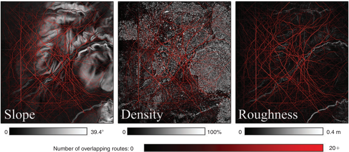
Fig. 9. Results of least-cost routes between 1000 randomly generated point location pairs throughout the study area with route overlap displayed against landscape parameters.
