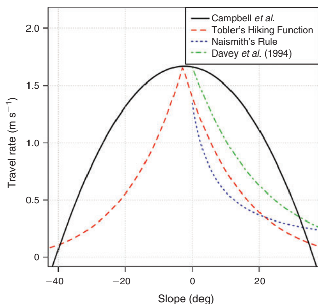
Fig. 11. Comparison of model results (calculated assuming zero vegetation density and zero ground surface roughness) to three well-established models used to estimate the effects of slope on travel rate. Davey et al. (1994)'s model was calibrated to match our model's 0° slope travel rate.
