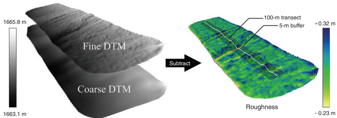
Fig. 2. Roughness calculation; digital terrain model (DTM) elevation values exaggerated 3\times to highlight texture.
