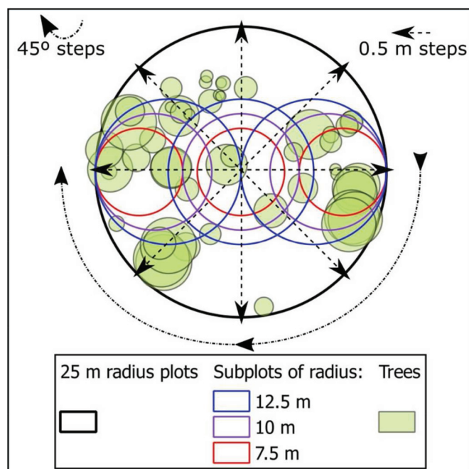
Fig. 2. Example of 25 m radius plot and subplots of radii 7.5 m, 10 m, and 12.5 m (for clarity, other subplot radii are omitted) moving in east to west, south east to northwest, south to north, and southwest to northeast directions. Field plots were moved in 0.5 m steps and are marked with dashed lines. Trees are plotted according to their crown radius. [Colour online.]
