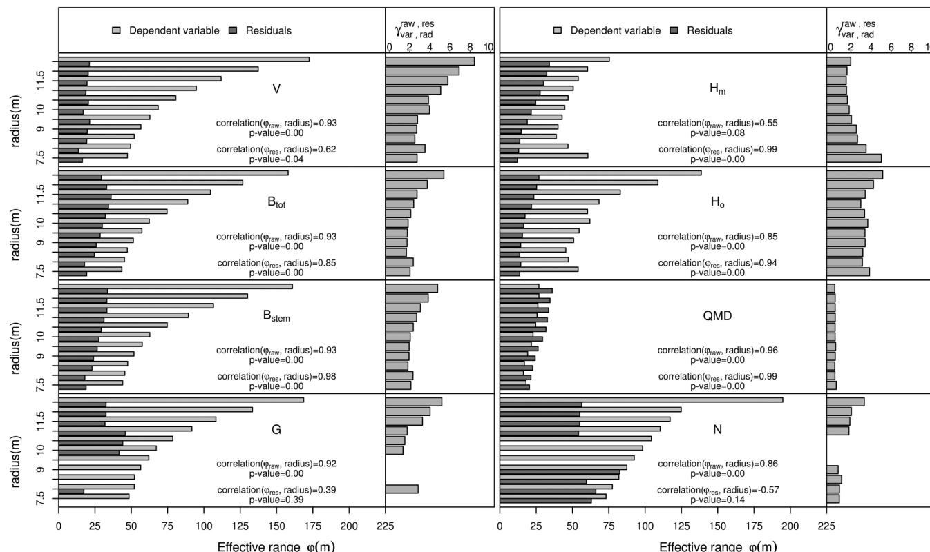
Fig. 4. Distances ( \phi ) for which correlation between pairs of observations decreases to 0.05 and parameters \gamma_{\text{var}, \text{rad}}^{\text{raw, res}} .
