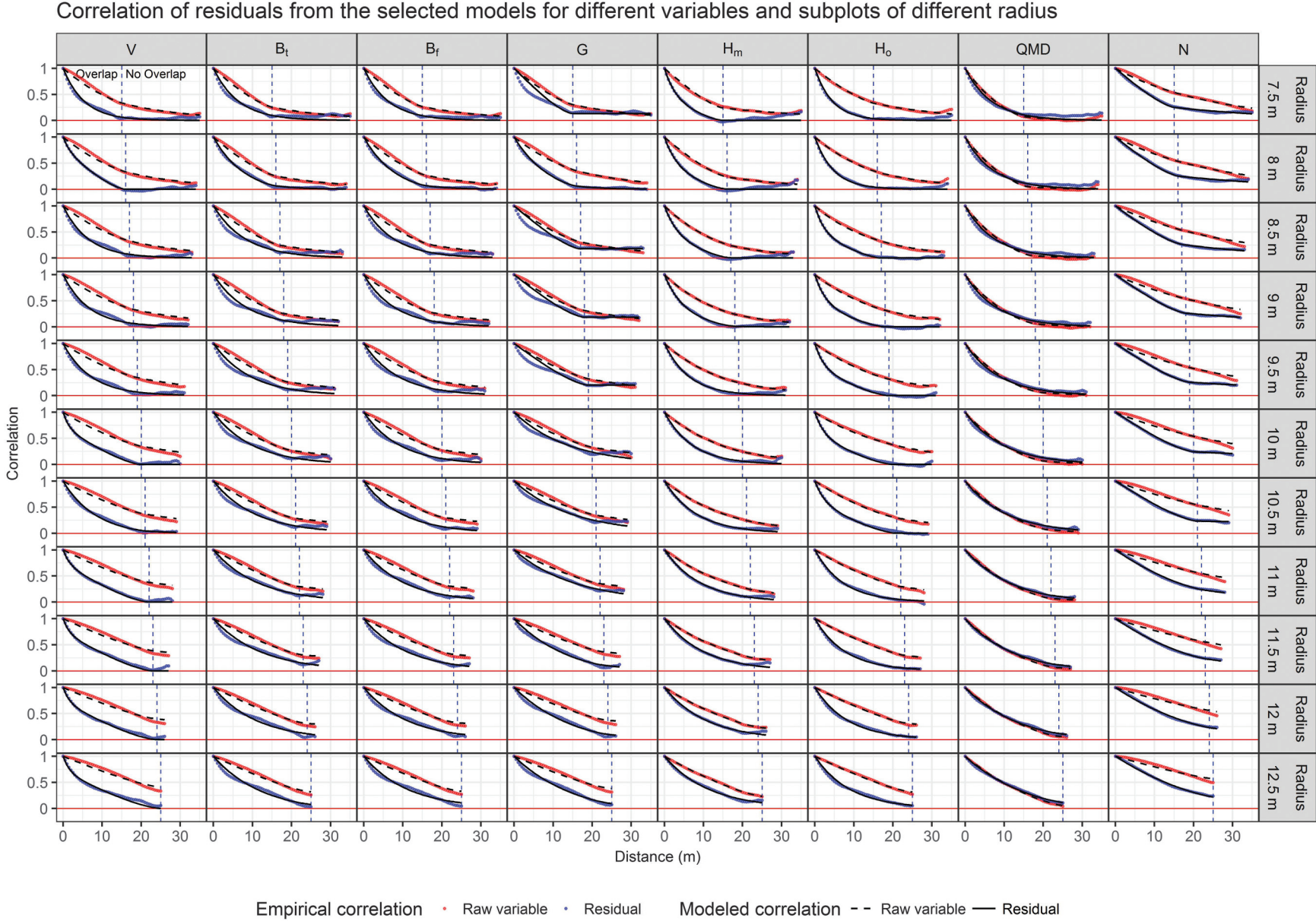
Fig. 3. Spatial correlation models for the residuals from m_{\text{vrb},\text{rad}}^{**} and for the raw variables.
