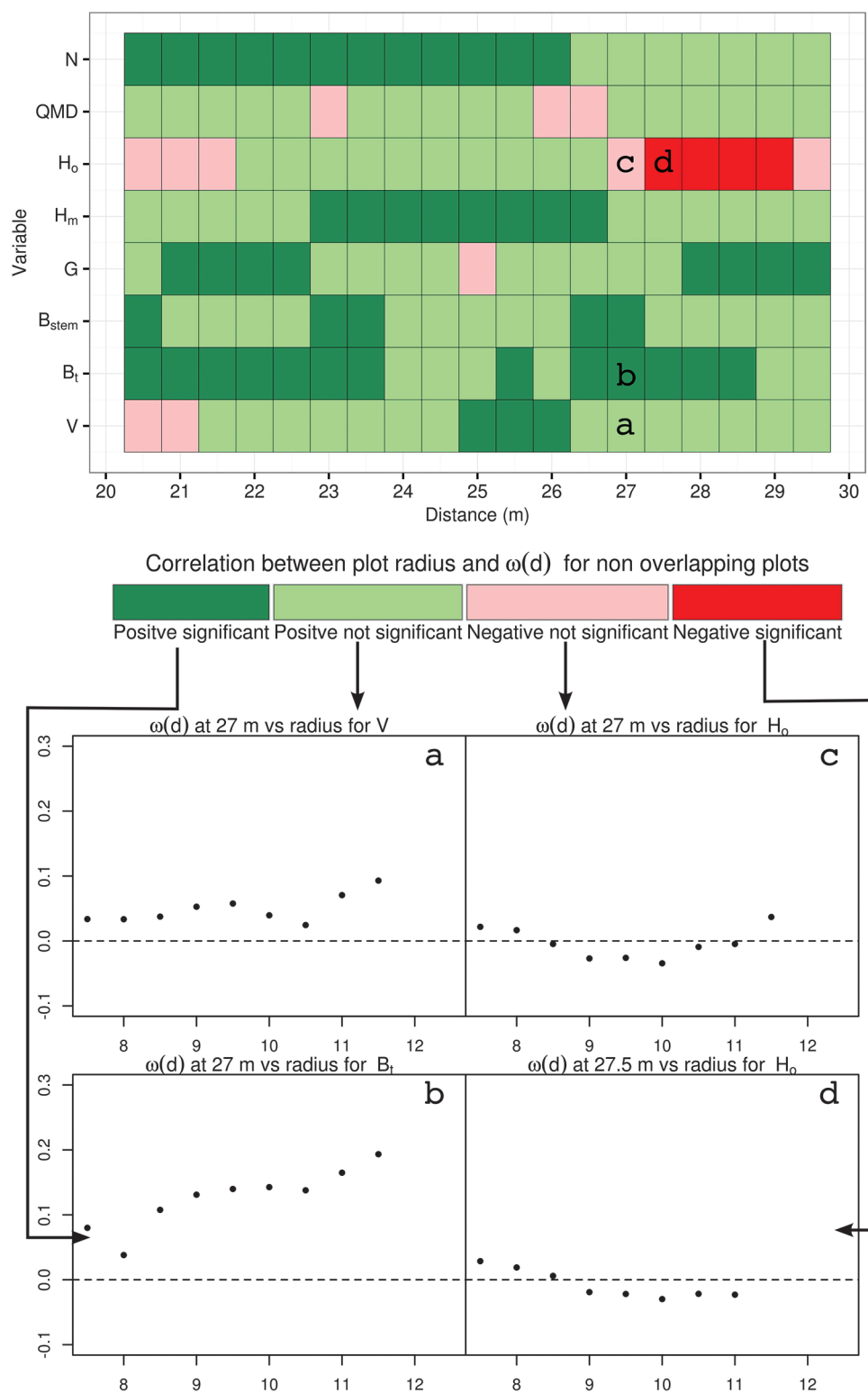
Fig. 5. Results for the Kendall's \tau significance test for each variable and subplot radius. Only non-overlapping plots are considered. Subfigures a , b , c , and d are examples included as a graphical legend for the figure in the upper panel. [Colour online.]
