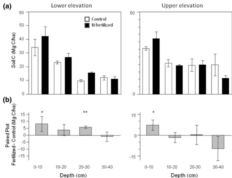
Fig. 2 a Bulk soil C content in 2005 is shown for control (white) and fertilized (black) plots to 40 cm depth (mean \pm 1 s.e., n = 3 ). b The fertilization effect (gray) is shown as a relative loss or gain in bulk soil C with fertilization (Mg C/ha), using differences between each pair of fertilized and control plots ( n = 3 ). * Indicates p < 0.1 ; ** indicates p < 0.05 for differences between paired plots
