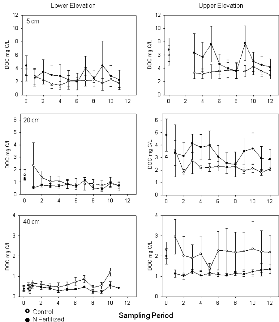
Fig. 5 Concentrations of dissolved organic carbon (DOC) in soil solution collected at three soil depths for control (white) and fertilized (black) plots are shown (mean \pm 1 s.e., n = 3 ). The zero-time point represents the average of eight pre-fertilization measurements for the 5 and 20 cm depths, and the average of two measurements during the first year of fertilization for the 40 cm depth (Table 4). Sampling periods 1–12 were distributed from August 2005 to August 2006
