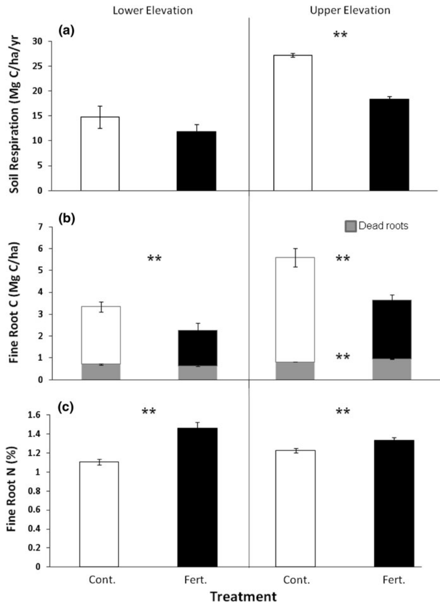
Fig. 4 a Soil respiration rates are shown for control (white) and fertilized (black) plots for two tropical forests. Note that reported daily rates from June to August 2006 have been scaled up to an annual rate here for comparability with C pools in fine roots and soils. b Fine root C pools are shown; dead fine root biomass is shown in grey for both treatments, and live fine roots are shown for control (white) and fertilized (black) plots. Live root biomass declined significantly with N fertilization in both forest types, and dead root biomass increased significantly with fertilization in the upper elevation forest. c Fine root N concentrations increased with N fertilization in both tropical forests, inversely corresponding to the decline in live fine root biomass. Cont. control plots, Fert. fertilized plots (all data are mean \pm 1 s.e., n = 3 ). * Indicates p < 0.1 ; ** indicates p < 0.05 . Stacked * in (b) indicates significant difference for live and dead fine roots
