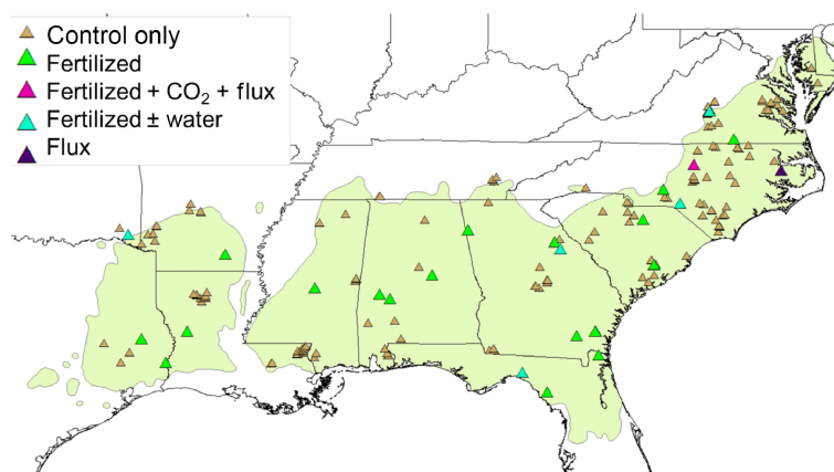
Figure 1. Map of loblolly pine distribution, plot locations used in data assimilation, and the experiment type associated with each plot. The control-only treatments were plots without any associated experimental treatment or flux measurements. Fertilized treatments were plots with nutrient additions. CO 2 treatments were plots with free-air concentration enrichment treatments. The flux treatments were plots with eddy-covariance measurements of ecosystem-scale carbon and water exchange. The water treatments included throughfall exclusion and irrigation experiments.
