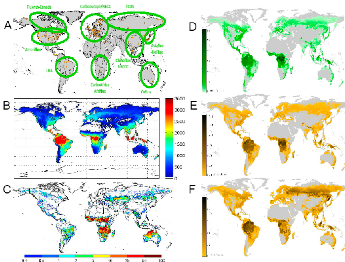
Figure 6. (A) Global network of eddy covariance flux towers in 2010; a larger number of towers exist, but not integrated in the FLUXNET database ( http://fluxnet.ornl.gov/fluxnetdb ). (B) Example of global distribution of the gross primary productivity obtained by fusion of FLUXNET measurements with global satellite fraction of absorbed photosynthetically active radiation, and gridded climate fields. (C) Global distribution of burned area from EOS-Terra-MODIS. (D) Global distribution of biomass obtained by disaggregating data from FAO reported by each country using satellite observations ( http://www.iiasa.ac.at/Research/FOR/biomass.html ), (E) below-ground biomass. (F) Soil carbon (from World Inventory of Soil Emission ISRIC-WISE database).
