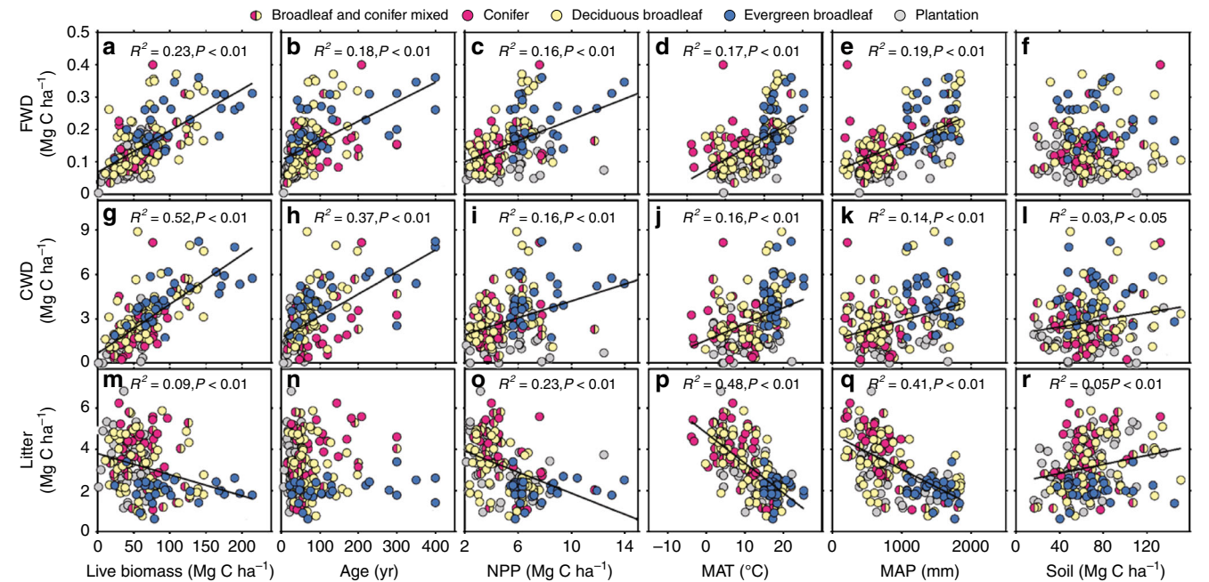
Fig. 3 Relationships between carbon density of dead organic matter, and biotic and climatic factors. The y axis is carbon density ( \text{Mg C ha}^{-1} ) of a–f fine woody debris (FWD), g–l coarse woody debris (CWD), and m–r litter. All plots showed the linear relationships between a, g and m above ground biomass carbon density, b, h and n forest age, c, i and o net primary production (NPP), d, j and p mean annual temperature (MAT), and e, k and q precipitation (MAP), and ( f, l and r ) soil carbon density and carbon density of each component of dead organic matter. There were no significant linear relationships between carbon density of litter and forest age, and between carbon density of FWD and carbon density of soil
