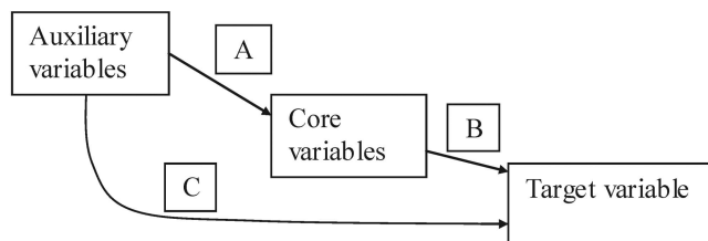
Figure 2. Reductive bridging when no core variables are immediately available. Arrow A indicates that core variables are predicted using auxiliary data and that a standard reductive bridging then is performed (arrow B). Alternatively, conversion factors based on auxiliary data can be used directly (arrow C).
