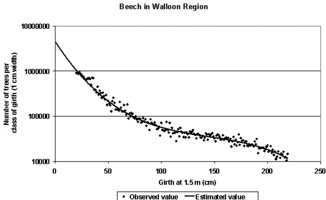
Figure 3. The observations and the fitted regression curve for predicting the total number of beech trees for a given circumference class (cm). R^2 = 0.978 ; the coefficient of variation for the estimated intercept was 2.7%.
