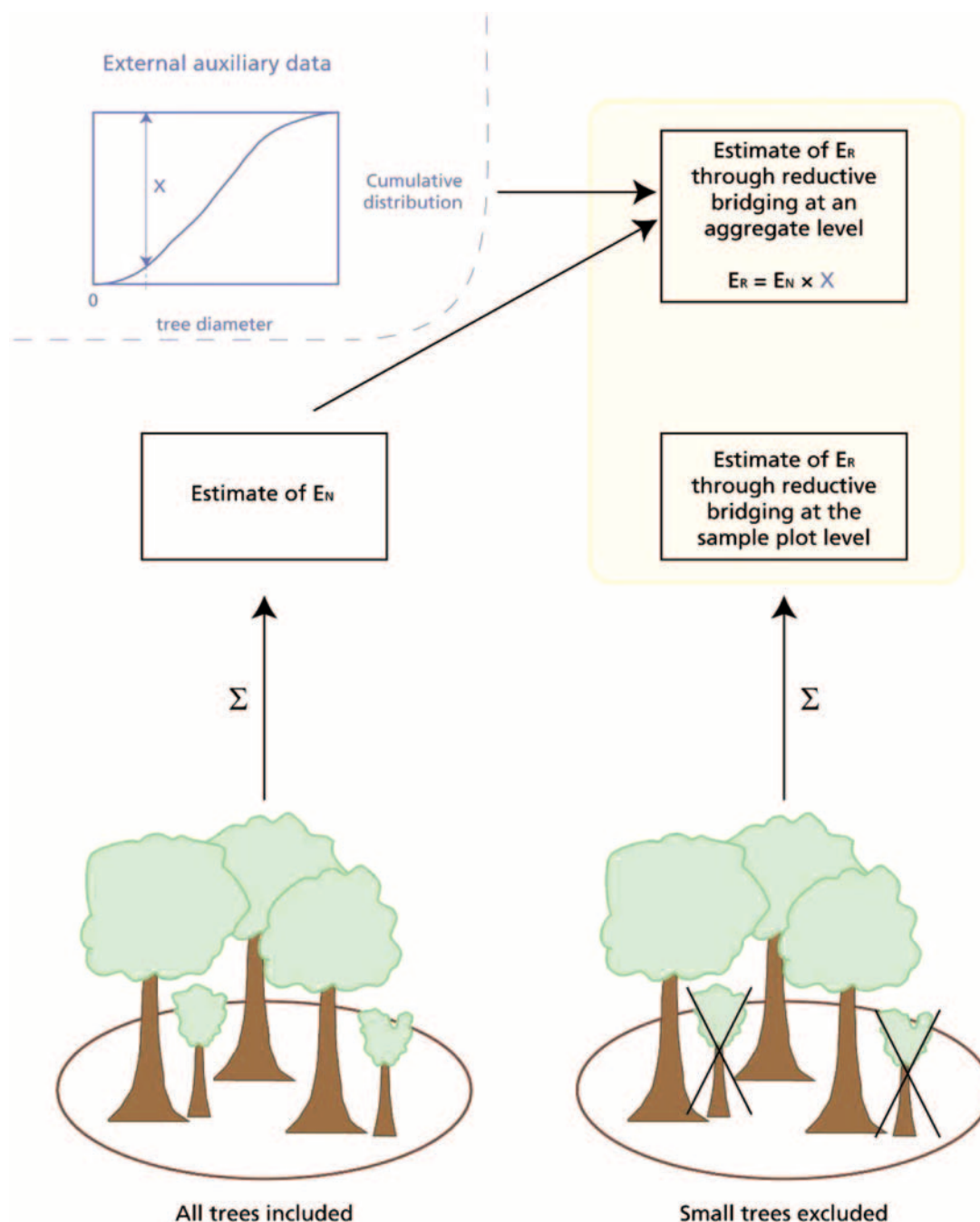
Figure 1. Application of a bridge (reductive) at the level of individual sampling units (right) and at the aggregate level (left); E_N is the target quantity according to the national definition and E_R the corresponding quantity according to the reference definition.
