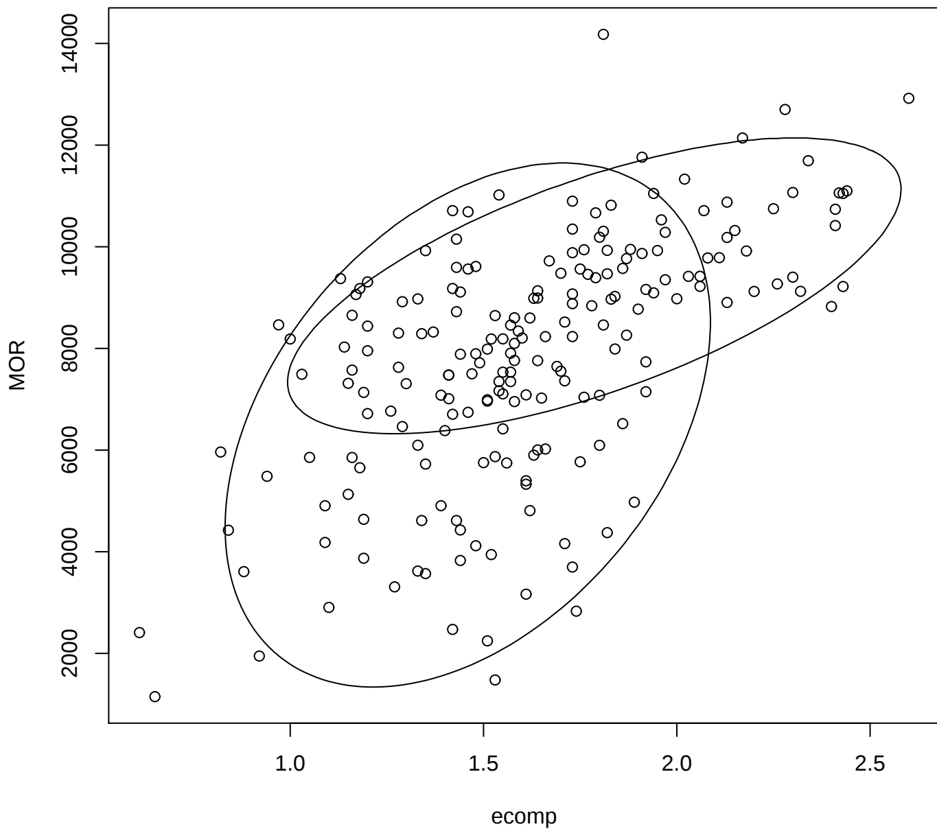
Figure 35: Scatter plot of MOR versus ecomp, and 0.90 probability content contours for the two bivariate normal components of the fitted mixed bivariate normal model.
