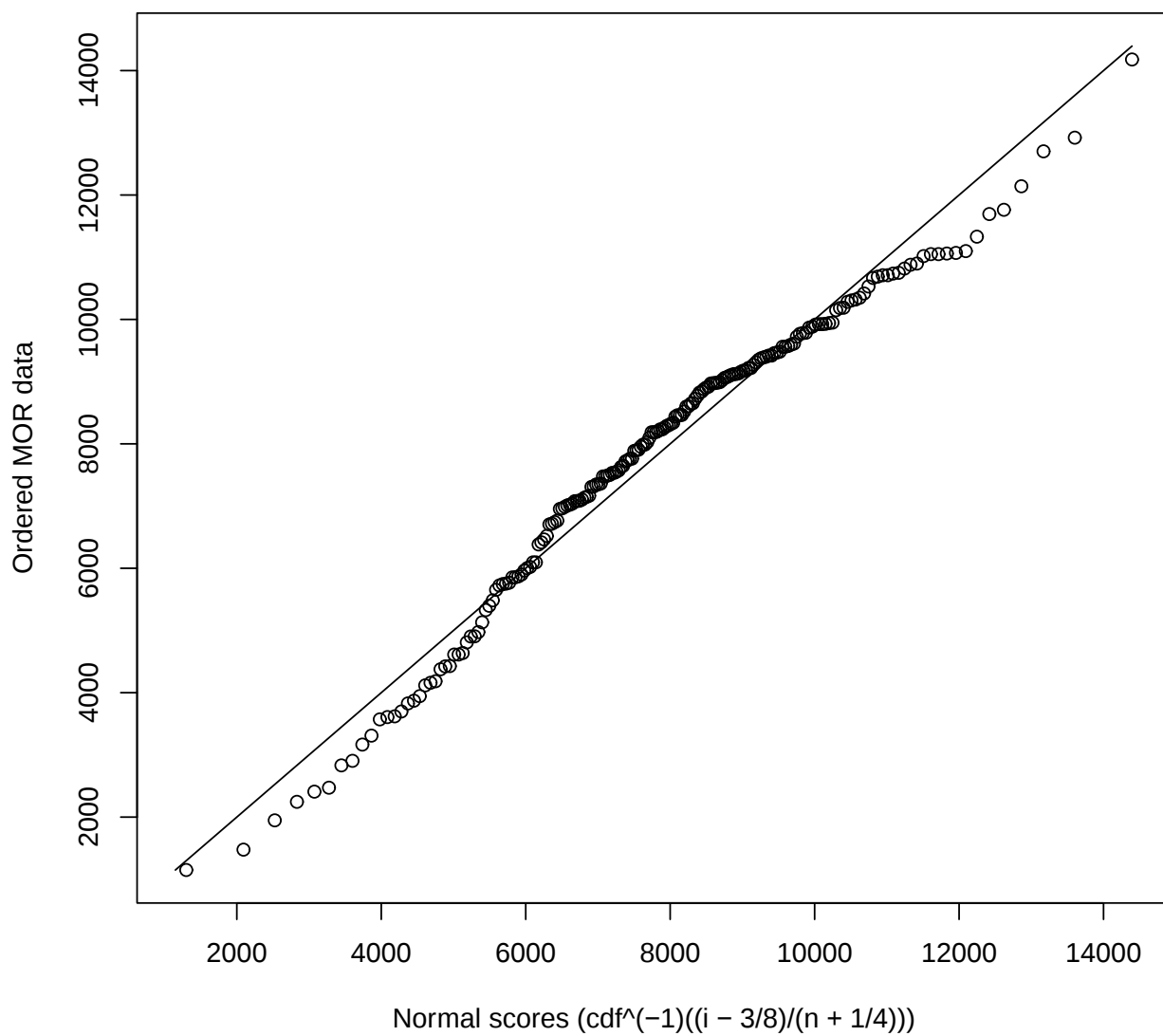
Figure 21: MOR. Ordered data versus predicted ordered data under the fitted normal model. The solid line is the y = x line. If a normal model is appropriate, the plotted data points will lie approximately along the y = x line.
