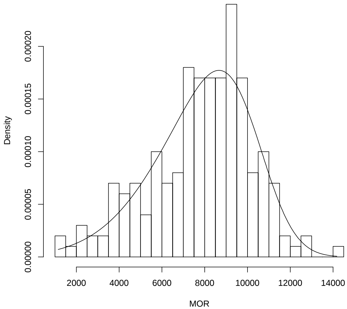
Figure 27: Histogram of the MOR data overlaid with the fitted skew normal probability density function.
