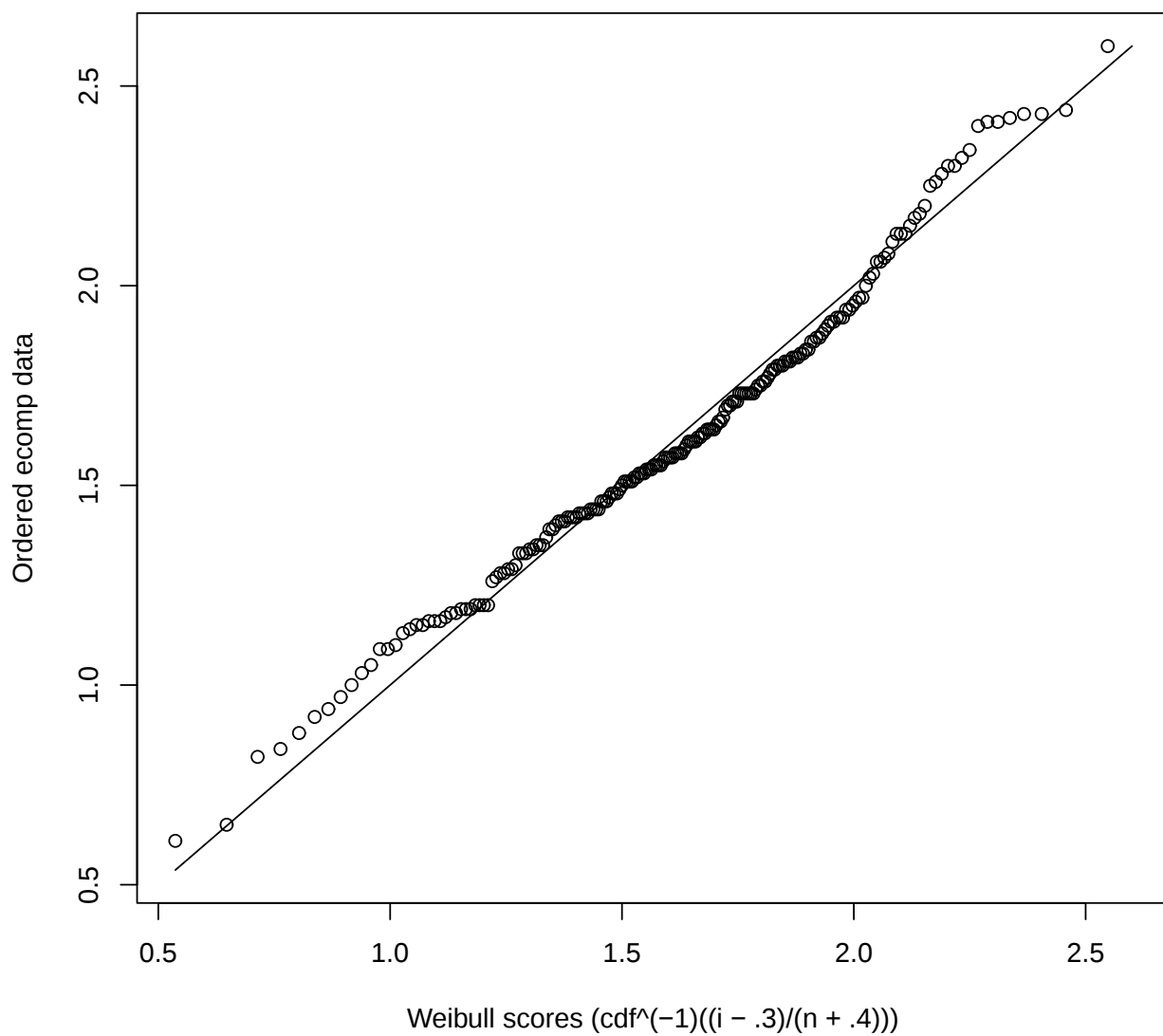
Figure 8: ecomp. Ordered data versus predicted ordered data under the fitted Weibull model. The solid line is the y = x line. If a Weibull model is appropriate, the plotted data points will lie approximately along the y = x line.
