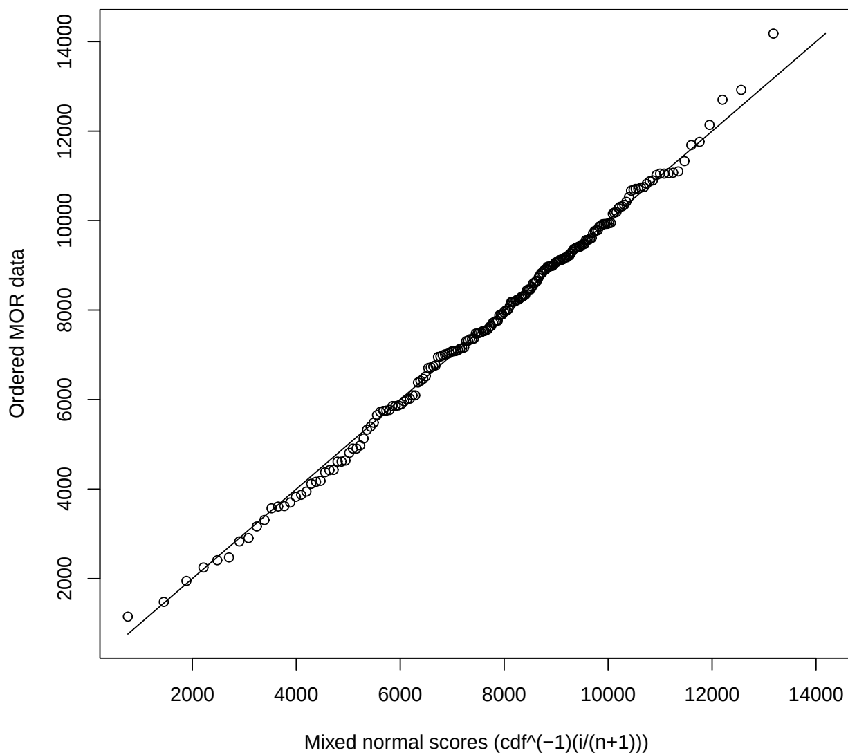
Figure 24: MOR. Ordered data versus predicted ordered data under the fitted mixed normal model. The solid line is the y = x line. If a mixed normal model is appropriate, the plotted data points will lie approximately along the y = x line.
