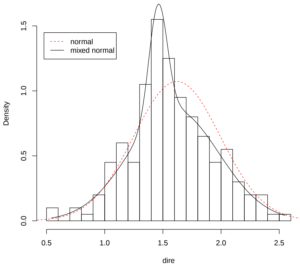
Figure 18: Histogram of the dire data overlaid with the fitted normal and mixed normal probability density functions.
