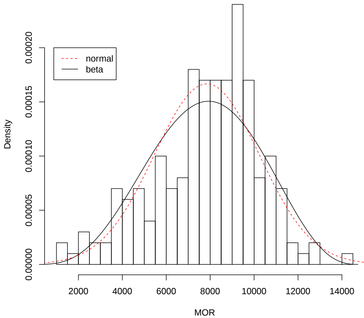
Figure 26: Histogram of the MOR data overlaid with the fitted normal and three-parameter beta probability density functions.
