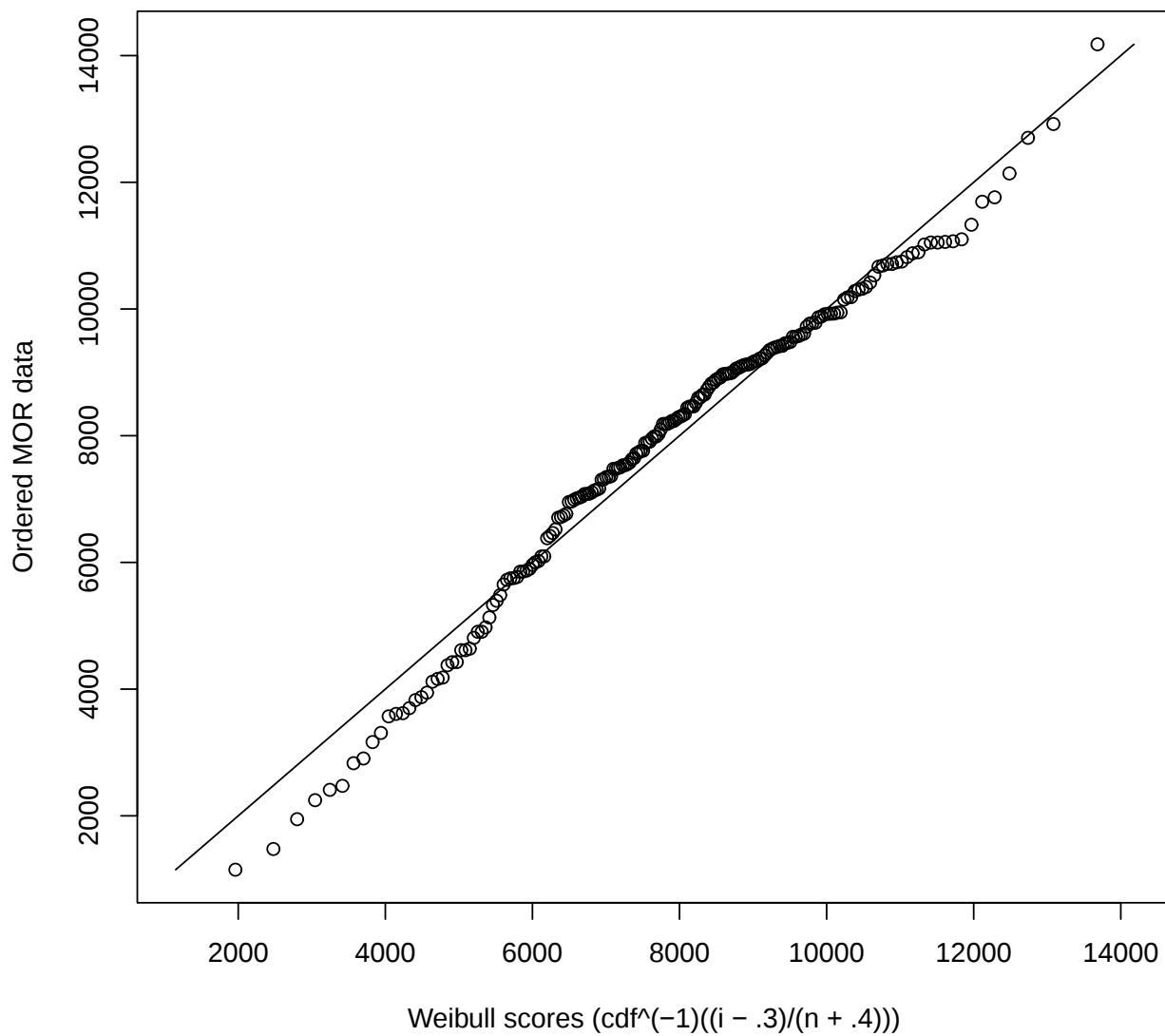
Figure 20: MOR. Ordered data versus predicted ordered data under the fitted Weibull model. The solid line is the y = x line. If a Weibull model is appropriate, the plotted data points will lie approximately along the y = x line.
