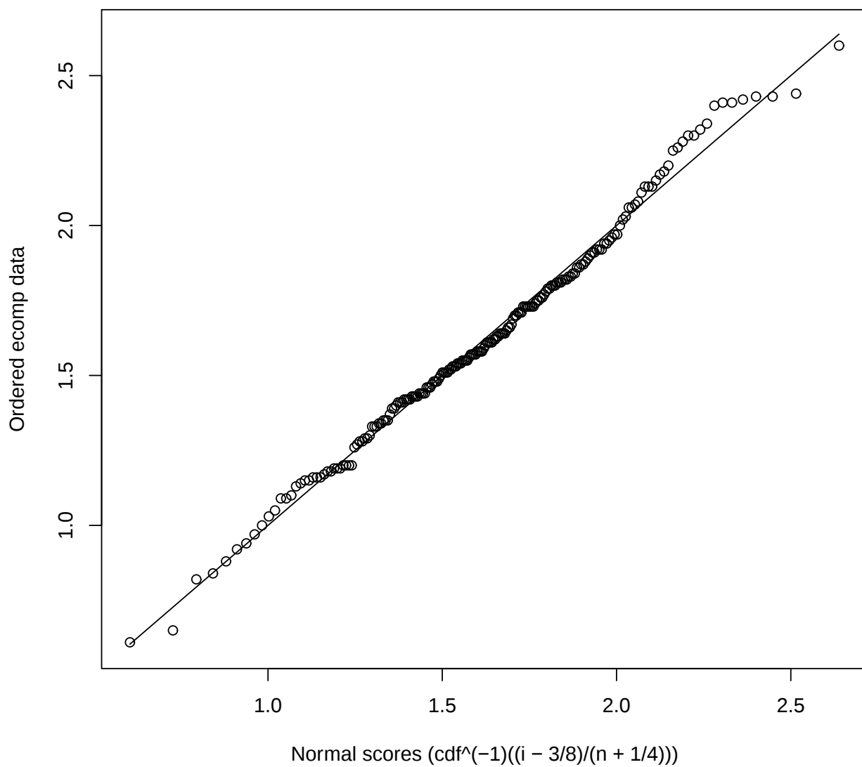
Figure 9: ecomp. Ordered data versus predicted ordered data under the fitted normal model. The solid line is the y = x line. If a normal model is appropriate, the plotted data points will lie approximately along the y = x line.
