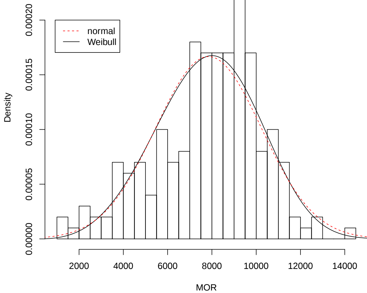
Figure 25: Histogram of the MOR data overlaid with the fitted normal and Weibull probability density functions.
