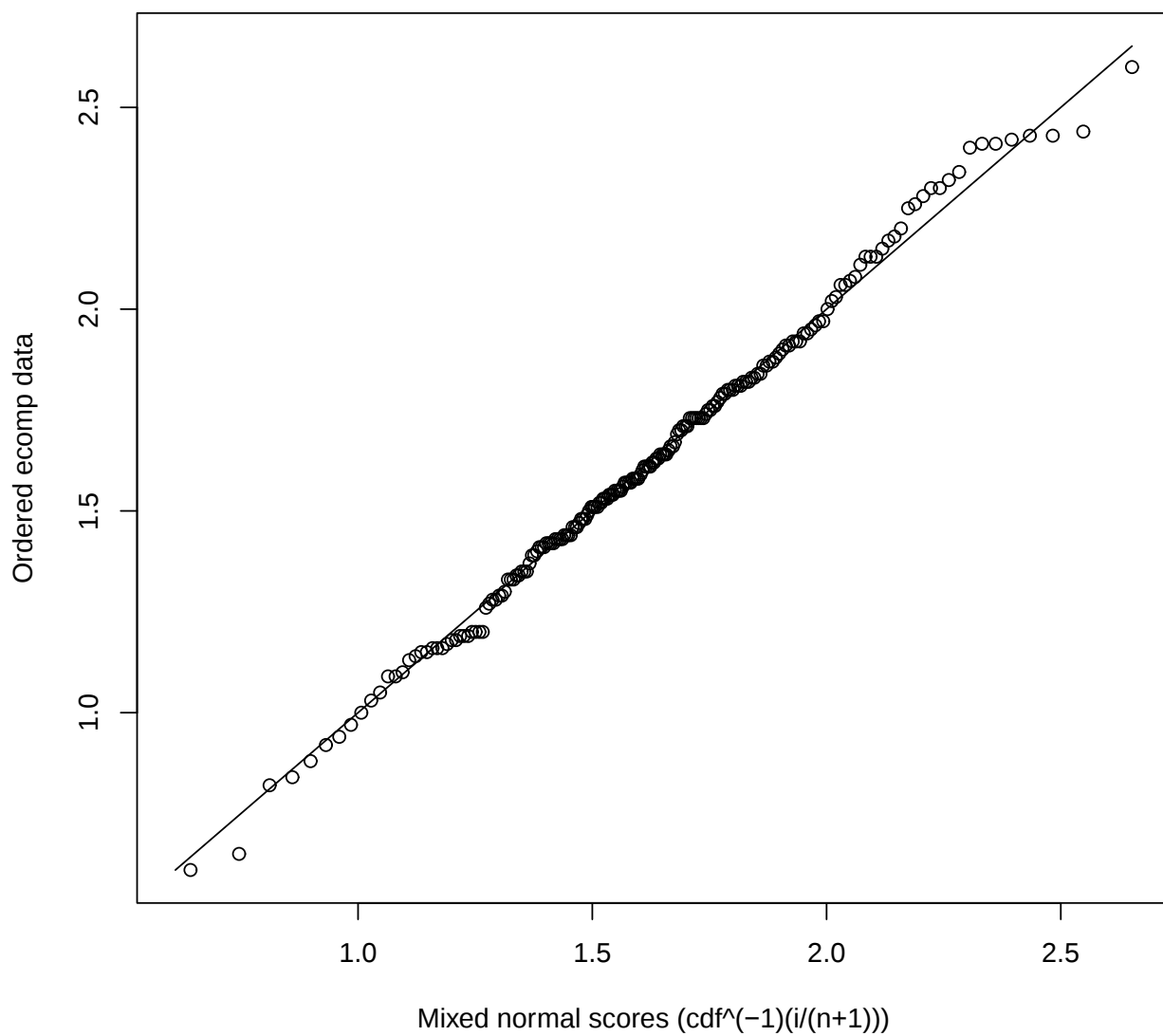
Figure 10: ecomp. Ordered data versus predicted ordered data under the fitted mixed normal model. The solid line is the y = x line. If a mixed normal model is appropriate, the plotted data points will lie approximately along the y = x line.
