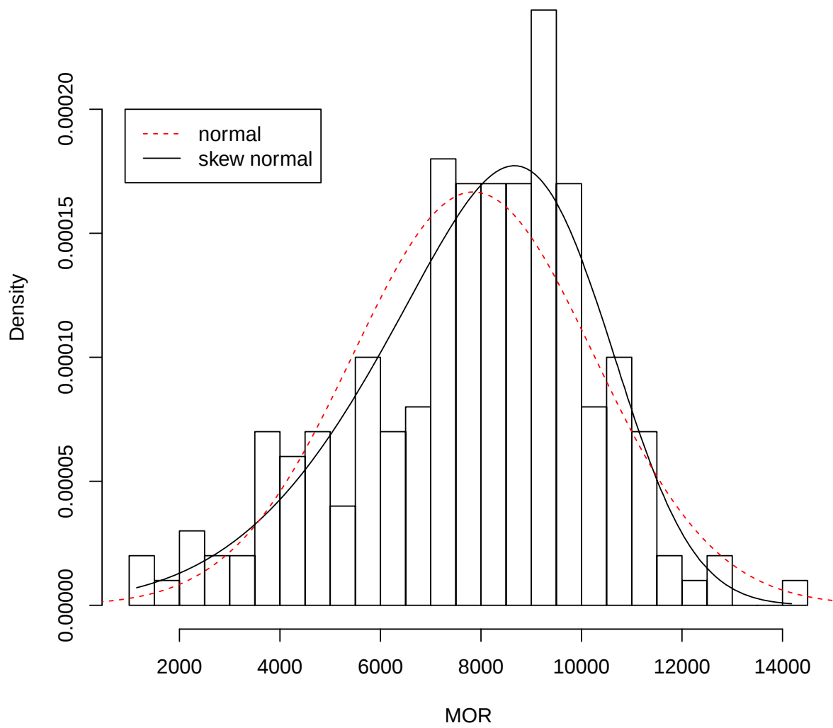
Figure 28: Histogram of the MOR data overlaid with the fitted normal and skew normal probability density functions.
