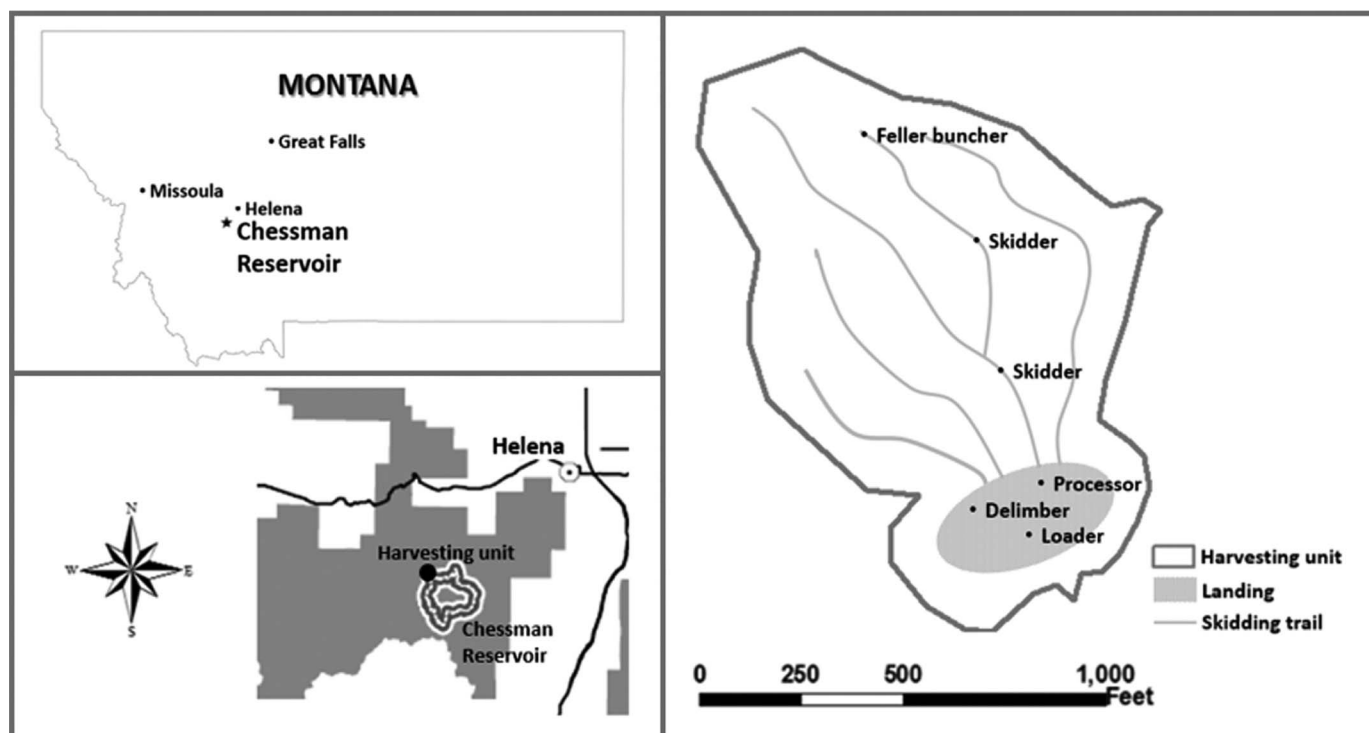
Figure 2. Site map showing the harvesting unit with general locations of equipment in the unit: the feller-buncher working the edge of the cut, the skidders transporting whole trees to the landing, the processor and delimber processing the trees, and the loader piling and loading the processed logs onto a truck.
