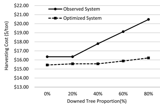
Figure 5. Unit costs before and after the configuration adjustment.
