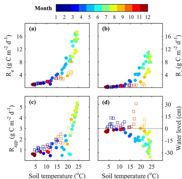
Fig. 5. The relationship between daily mean soil temperature and (a) ecosystem respiration ( R_e ), (b) site average belowground respiration ( R_s ), (c) aboveground plant respiration ( R_{agg} ), and (d) water level in 2010. Solid circles represent non-flooded scenarios and open squares represent flooded scenarios. Please refer to online materials for original figure in color.
