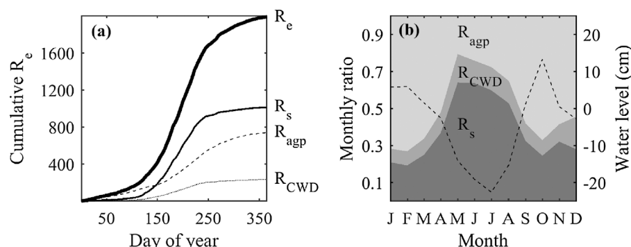
Fig. 4. Partitioning ecosystem respiration ( R_e ) into below-ground respiration ( R_s ), decomposition of coarse woody debris ( R_{CWD} ) and aboveground plant respiration ( R_{agg} ) in a lower coastal plain forested wetland in 2010. (a) Cumulative daily values ( g\ CO_2-C\ m^{-2}\ yr^{-1} ); (b) Monthly ratios of component fluxes to R_e (left axis) and monthly average water level (dashed lines, right axis).
