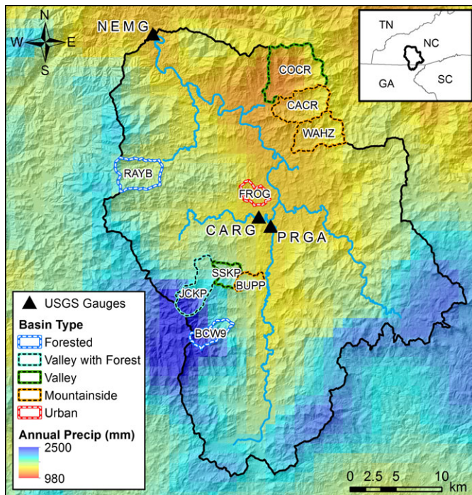
FIGURE 1. Upper Little Tennessee River Basin with Monitored Tributaries and U.S. Geological Survey (USGS) Gage Sites and Average Annual Precipitation (PRISM) Showing a Strong Precipitation Gradient from the Southern and Western Streams to the Northeastern Streams. Stream codes are given in Table 1. Stream basin polygons are color coded by development type. GA, Georgia; NC, North Carolina; TN, Tennessee; SC, South Carolina.
