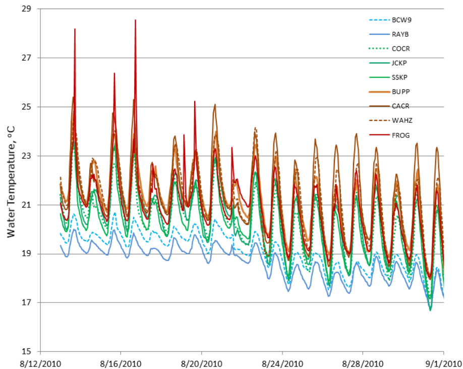
FIGURE 7. Comparison of Subhourly Temperature Time Series for All Nine Smaller Streams from August 13-31, 2010. Highest water temperatures occur in July and August in the study region. The forested streams are generally two degrees cooler than the valley development streams and feature much lower diurnal variation than all other sites. The urban and mountainside development streams feature the highest water temperatures.
