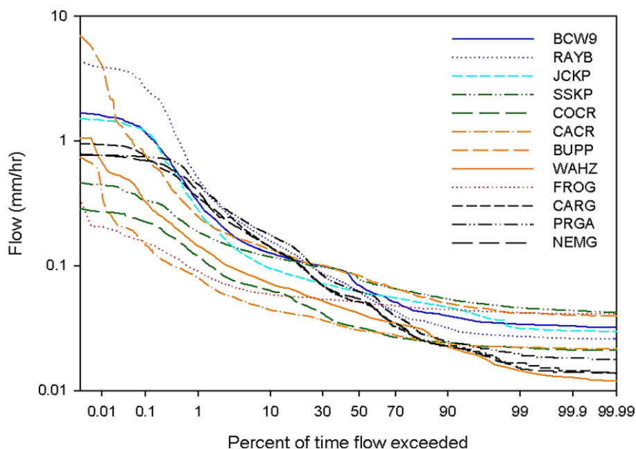
FIGURE 2. Flow Duration Curves for Study Sites during the 13-Month Common Sampling Period. Unexpectedly, the forested streams featured the very high peak flows and also low flows, probably due to the higher precipitation in the south and west sides of the study areas. High flow behavior among the streams seems to track with variability in average annual precipitation (Figure 1).
