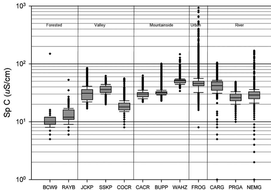
FIGURE 6. Specific Conductance (SpC) Values from All Measurements Collected at Study Sites. Specific conductance was substantially lower in the forested streams, but was highly variable among the streams within each development type, as well as among the larger river sites. Median SpC values are not highly correlated with any land cover statistic.
