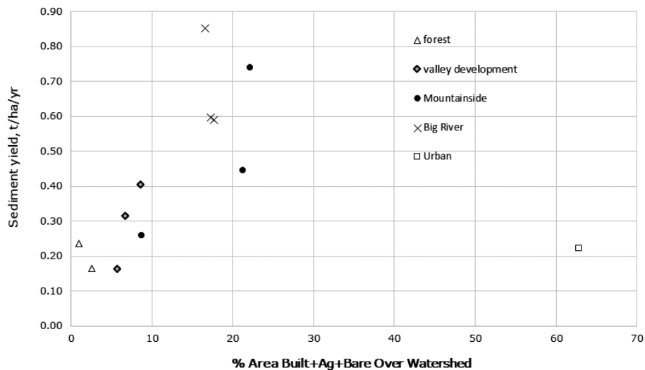
FIGURE 5. Sediment Yield as a Function of the Percentage of Watershed Area Characterized by the Sum of Built Lands, Agriculture, and Bare Soils. Sediment yield from the one urban stream, FROG, is clearly governed by different processes than the rural streams. The river sites feature particularly high sediment yields, indicating sediment sourcing from riverbanks in the main valley (Leigh, 2015).
