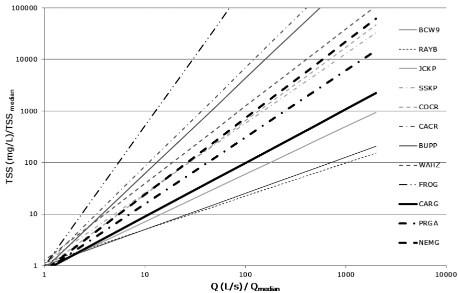
FIGURE 4. Normalized total suspended solids (TSS) vs. Discharge Rating Curves for Each Study Site Showing that the Slope of the Curve Increases with Increasing Watershed Development for the Nine Smaller Streams. The larger river systems appear to integrate the basin response, and these curves lie toward the middle of the set of curves from the smaller streams.
