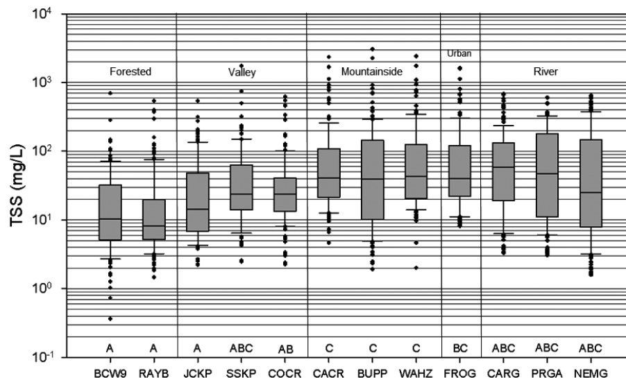
FIGURE 3. Box Plot of Total Suspended Solids Concentrations and Holm-Sidak Test Results from Storm Samples Collected over 18 Months at the Study Streams. Box is defined by 25th and 75th percentiles, solid line in box is median, and whiskers are 10th and 90th percentiles. Storm total suspended solids (TSS) concentrations in the mountainside development streams were very similar to the urban stream and were higher than the valley development streams. Storm TSS values in the valley development streams were generally higher than in forested streams, but the average values were not statistically different. Storm TSS values in the river sites were highly variable, but average values were similar to the mountainside and valley development sites.
