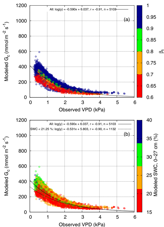
Figure 8. Hourly modeled canopy conductance vs. observed VPD for the summer months (June–September) of the years 1999–2006, restricted to 10:00–16:00 PST (additional restrictions were imposed to the calculation of G_c ; see Sect. 2.7). Note that observed air temperature and relative humidity were used to drive CLM. The years 1998 and 2005 were not included for consistency with Fig. 7. Data points were segregated according to the soil moisture stress parameter \beta_t in panel (a) and according to modeled SWC in panel (b) (see Fig. 6). Lines correspond to the linear regression between \log G_c and VPD using all data points (solid lines) and using only points within the lowest SWC bin (red circles, dashed line).
