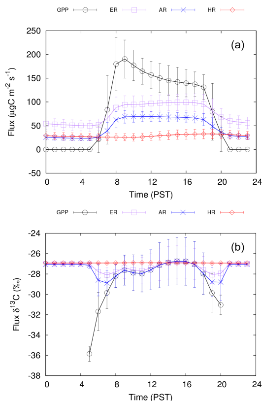
Figure 4. Mean diurnal cycle of modeled carbon fluxes (a) and their respective carbon isotope ratios (b) for the summer months (June–September) of the years 1998–2006. Fluxes include gross primary production (black circles), ecosystem respiration (purple squares), autotrophic respiration (blue crosses), and heterotrophic respiration (red diamonds). Bars correspond to \pm 1 SD.
