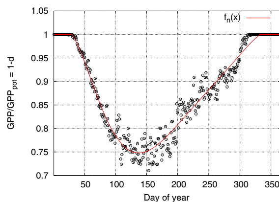
Figure A3. Modeled fraction of potential GPP ( \text{GPP}/\text{GPP}_{\text{pot}} ). Data points correspond to daily means averaged over 1850–2006 (calibrated CLM simulation). The fitted curve is f_n(x = \text{day of year}) = -1.39697 \times 10^{-14}x^6 + 1.71948 \times 10^{-11}x^5 - 8.26883 \times 10^{-9}x^4 + 1.90682 \times 10^{-6}x^3 - 1.97639 \times 10^{-4}x^2 + 0.0055728x + 0.966272 for 31 \leq x \leq 332 and f_n(x) = 1 elsewhere. Note that \text{GPP}/\text{GPP}_{\text{pot}} = 1 - d , where d is the nitrogen down-regulation factor as defined in Eq. (9) within text.
