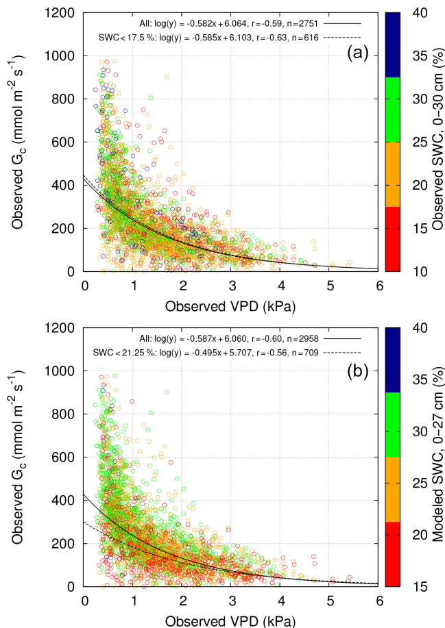
Figure 7. Hourly observed canopy conductance vs. observed VPD for the summer months (June–September) of the years 1999–2006, restricted to 10:00–16:00 PST (additional restrictions were imposed to the calculation of G_c ; see Sect. 2.7). The years 1998 and 2005 were not included due to missing data. Data points were segregated according to observed SWC in panel (a) and according to modeled SWC in panel (b) (see Fig. 6). Lines correspond to the linear regression between \log G_c and VPD using all data points (solid lines) and using only points within the lowest SWC bin (red circles, dashed lines).
