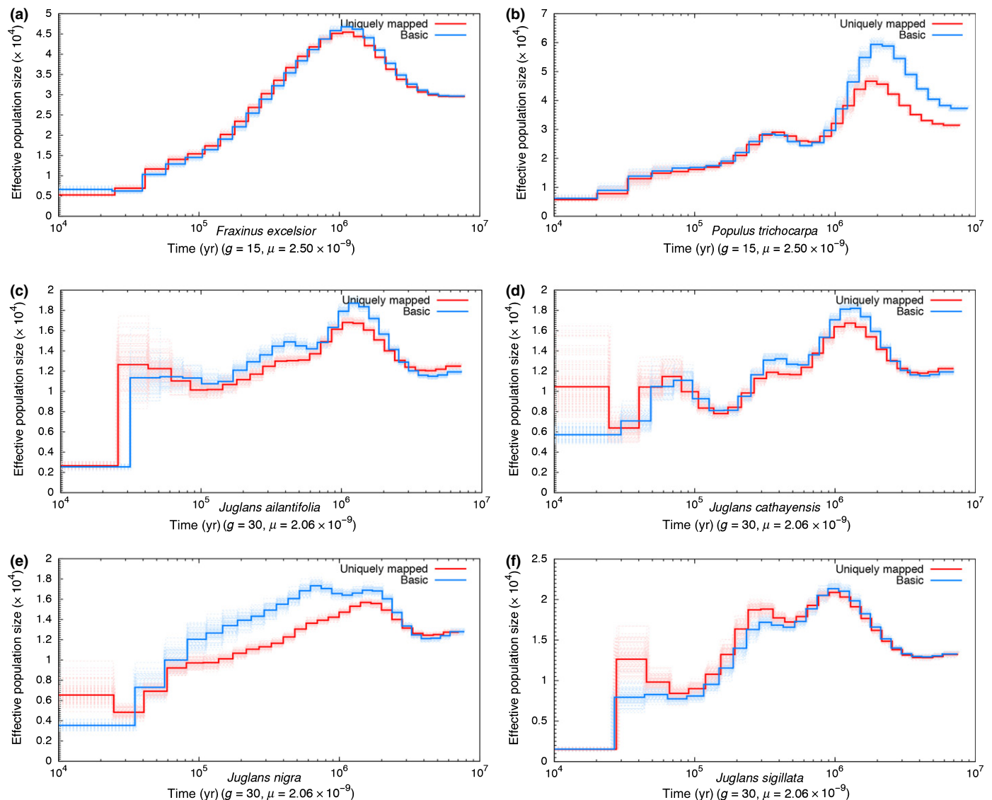
Fig. 2 Comparison of pairwise sequentially Markovian coalescent estimates of the changes in effective population size over time for Fraxinus excelsior (a), Populus trichocarpa (b), Juglans ailantifolia (c), Juglans cathayensis (d), Juglans nigra (e), and Juglans sigillata (f) when using a basic strategy of data filtering (blue) vs using only uniquely mapped repeats (red). g , generation time (yr); \mu , mutation rate.
