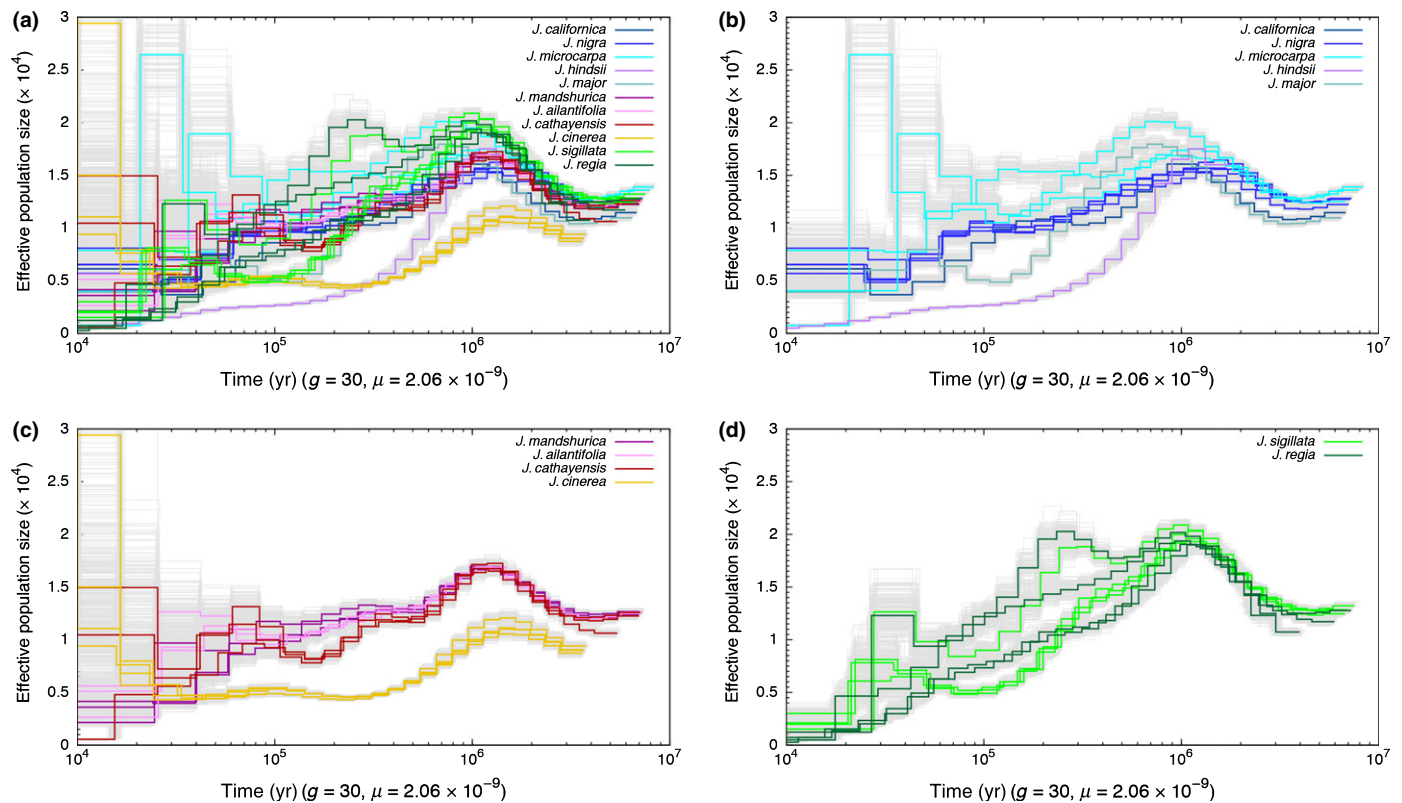
Fig. 1 Pairwise sequentially Markovian coalescent estimates of the changes in effective population size over time for 11 temperate species of Juglans . (a) All the individuals; (b) section Rhysocaryon ; (c) section Cardiocaryon ; (d) section Dioscaryon . Each line represents one individual. Gray lines indicate 95% confidence intervals. g , generation time (yr); \mu , mutation rate.
