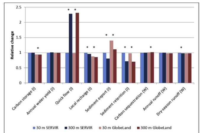
Fig. 4. Effects of spatial resolution on ecosystem service model results: 2010 SERVIR and GlobeLand data at 30 and 300 m resolution using InVEST (I) and WaSSI (W). Values are normalized relative to model results obtained from the 30 m SERVIR data. Asterisks indicate statistically significant differences in mean value by subwatershed between different input resolutions (Wilcoxon signed ranks test; all p \leq 0.05 ).
