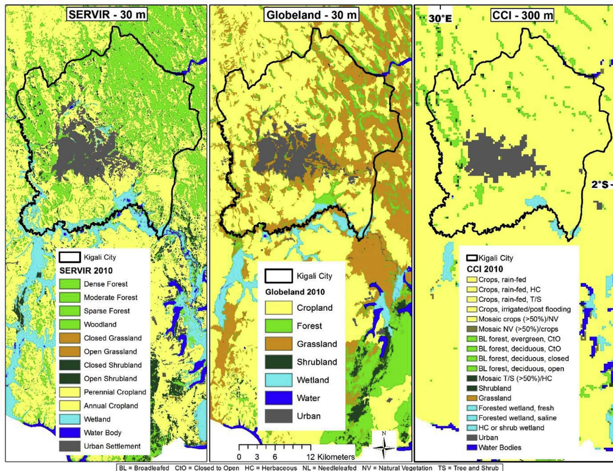
Fig. 2. Land cover for Kigali City: (a) SERVIR Scheme II 30 m, 2010; (b) GlobeLand 30 m, 2010; (c) CCI 300 m, 2010.
