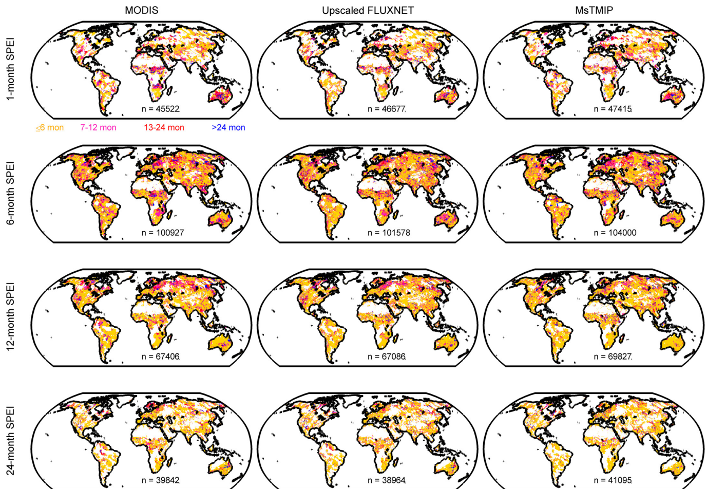
Extended Data Figure 6 | Spatial patterns of recovery time. Panels show mean recovery time by grid cell for all combinations of GPP dataset and integration time. Colours denote recovery time as shown. Inset values show number of drought and recovery events, n . White areas are water, barren, or did not experience any relevant drought events.
