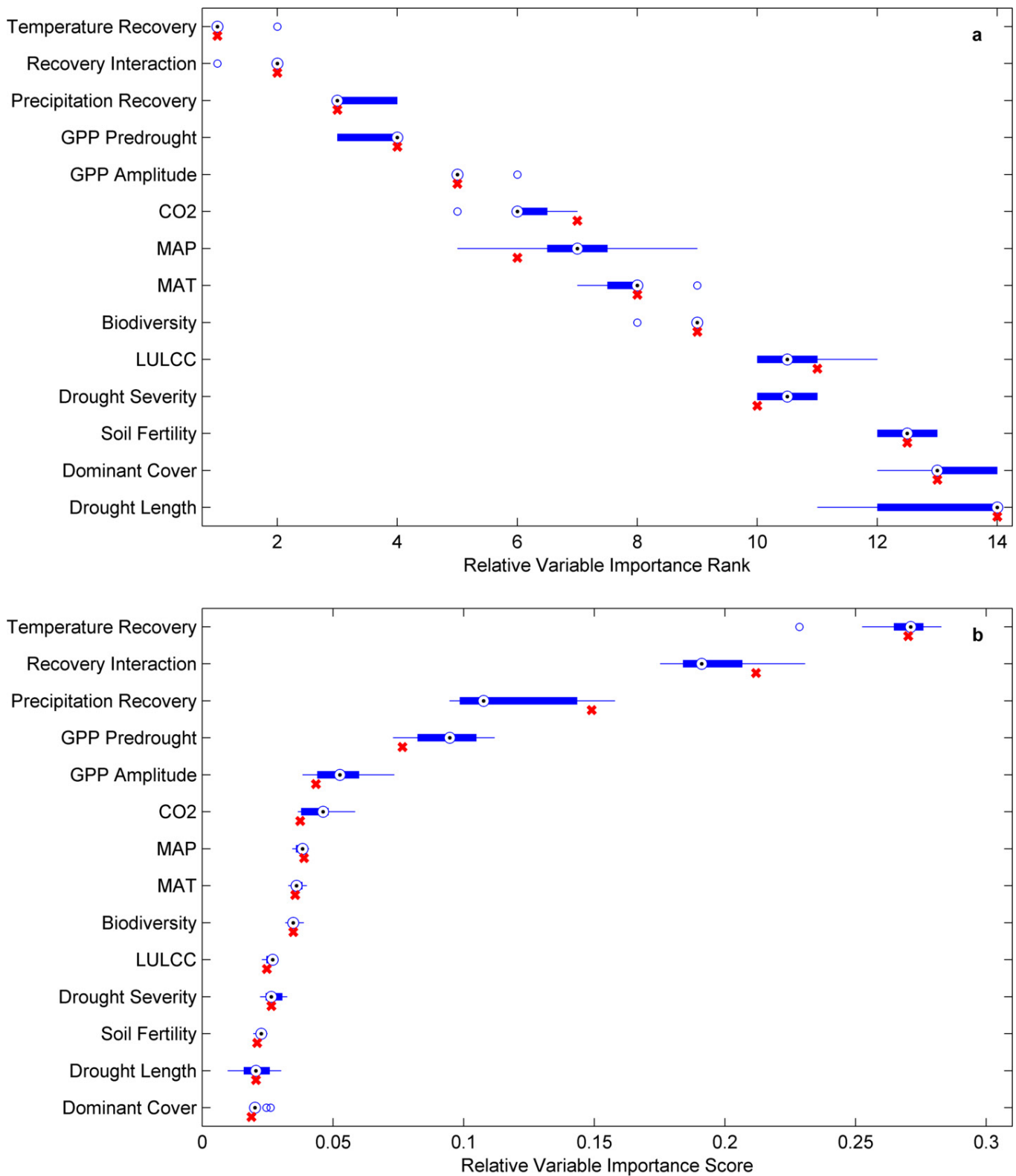
Extended Data Figure 1 | Variable importance scores. a, Covariates by rank of variable importance. b, Covariates by value of relative variable importance. Scores allow the skill of a trained Random Forest to be decomposed and mapped to individual covariates. Box plots are based on all possible combinations of GPP dataset and integration time. The box range covers the 25th to 75th percentiles; whiskers extend from about the 0.50th to 99.50th percentiles; outlying values are given by open circles. Red crosses give the composite value from the weighted median with
