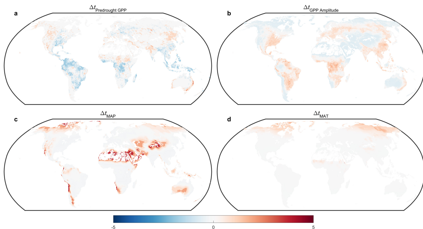
Extended Data Figure 2 | Spatial gradients of recovery time. a , Pre-drought GPP. b , GPP amplitude. c , MAP. d , MAT. Mapped values for a and b are based on the mean across all events (all GPP datasets, all integration times, and all time steps) by grid cell. For c and d the covariates from training the Random Forests algorithm (see Methods) are used directly. Recovery time is then projected spatially by matching response function
