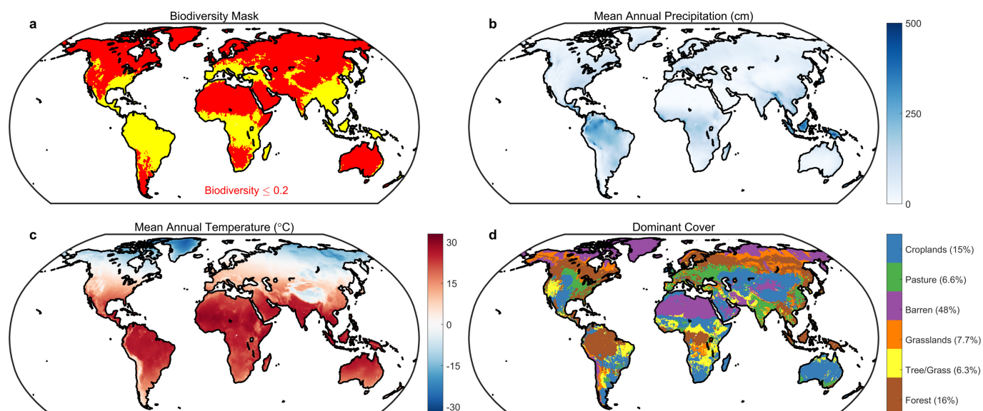
Extended Data Figure 3 | Enviroclimatic spatial gradients associated with recovery time. a , Mask of normalized biodiversity \leq 0.2 ; these areas show an increase in recovery time with decreasing biodiversity across space. b , MAP. c , MAT. d , LULCC. Values in parentheses give areal extent
