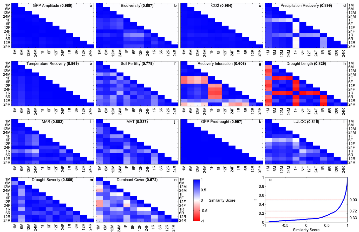
Extended Data Figure 7 | Response function similarity. Panels a to n show similarity score (correlation) across all possible combinations of GPP dataset and integration time by covariate. Each panel gives the covariate name and median of all off-diagonal scores. Integration time and GPP dataset are abbreviated in the y-axis labels as number–letter couplets (the number indicates the integration time in months, the letter indicates the GPP dataset (M, MsTMIP; F, upscaled FLUXNET; R, remotely sensed
