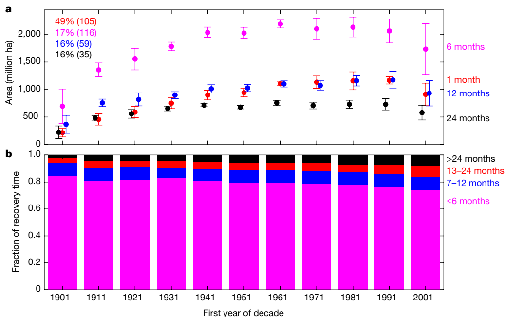
Figure 3 | Decadal changes in drought recovery. a , Global area undergoing a drought recovery for 1-month (red), 6-month (magenta), 12-month (blue), and 24-month SPEI (black). Data are mean \pm s.d. ( n = 10 ) from annual values. The colour-coded values are linear trend estimates (all *P < 0.05 ) in per cent relative to first decade and in million hectares per
