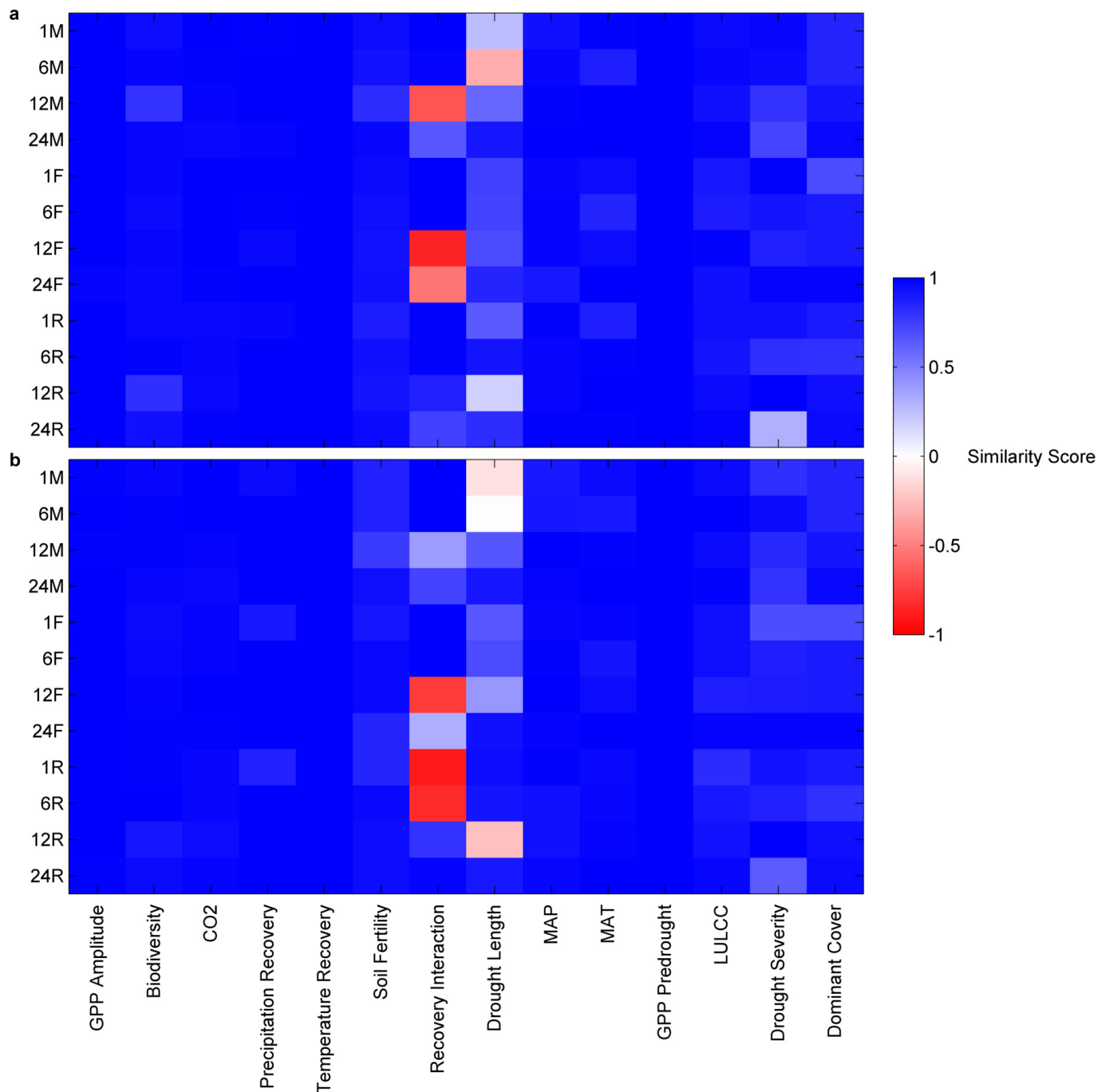
Extended Data Figure 8 | Response function similarity. Each colourmap pixel shows the similarity score (correlation) between the mirroring and fixed window approaches to calculate the pre-drought baseline across the common time frame for all three datasets (2000 to 2008). a , 3-month fixed
