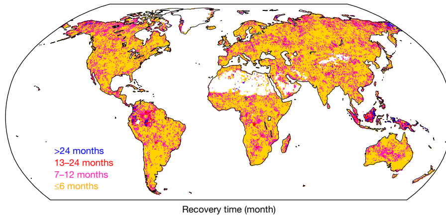
Figure 2 | Spatial pattern of drought recovery time. Recovery time by grid cell across all combinations of GPP and integration time (see Methods). White areas are water, barren, or did not experience any relevant drought events.
