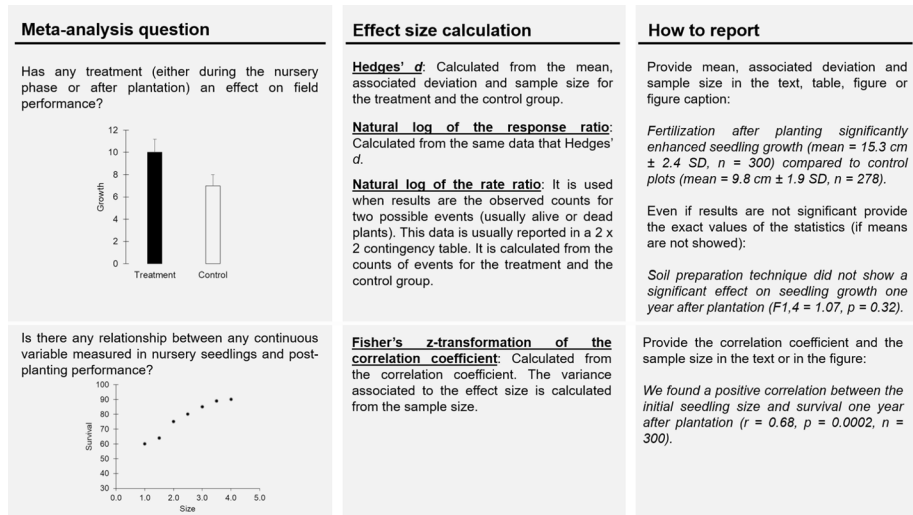
Fig. 1 Examples of questions on seedling quality research that can be addressed through meta-analysis (left column). The centre column contains information regarding the effect size used for each type of meta-analysis (rows), and the right column provides examples of proper reporting of data in primary studies for both examples
