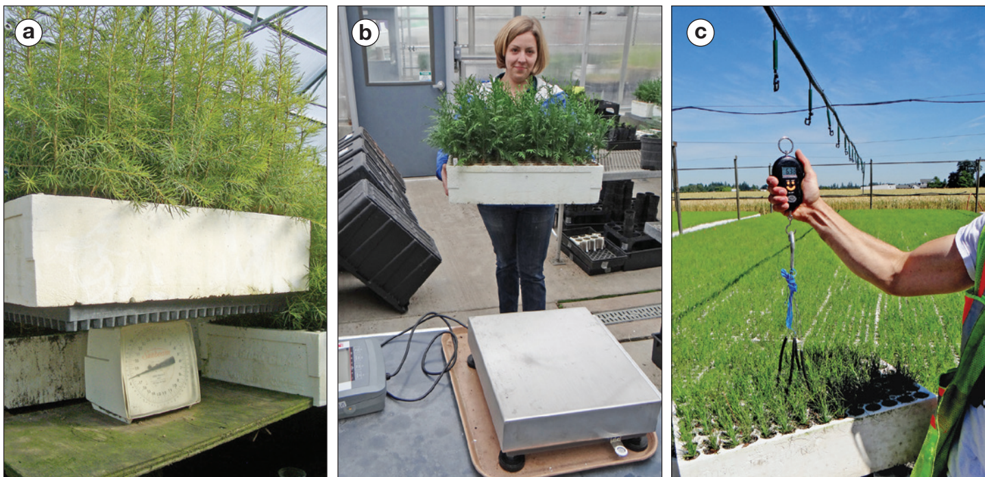
Figure 5. Weighing containers, a common method of monitoring irrigation needs in container nurseries, can be accomplished with (a) dedicated balances in the crop, (b) carrying or carting a balance to different locations in the nursery, or (c) using a hand-held balance. (Photos by R. Kasten Dumroese, 2006, 2015, 2014; from Dumroese et al. 2015)
