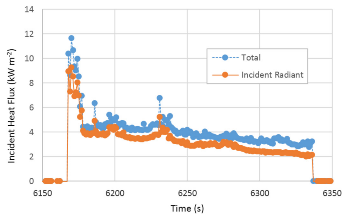
Figure 7. Total and radiant heat flux measured at the FBP as the flame front passed the in situ instrument location (Figure 1). The difference between total and radiant is indicative of convective heat flux. Time on the x-axis was not calibrated and thus is only relative.
