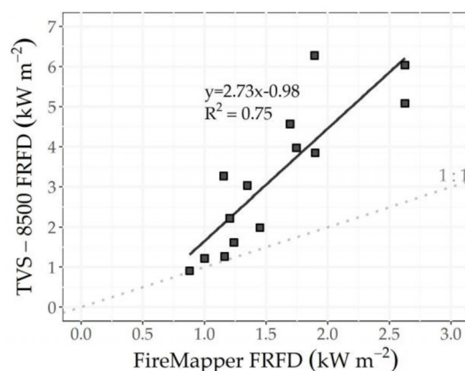
Figure 16. Spatially and temporally coincident comparisons of Fire Radiative Flux Density (FRFD) estimated from the ground-based TVS-8500 (middle infrared, low-oblique view) and the airborne FireMapper™ (long-wave infrared, nadir view). Estimates of FRFD are the average over all active fire pixels detected in the fuel plot only.
