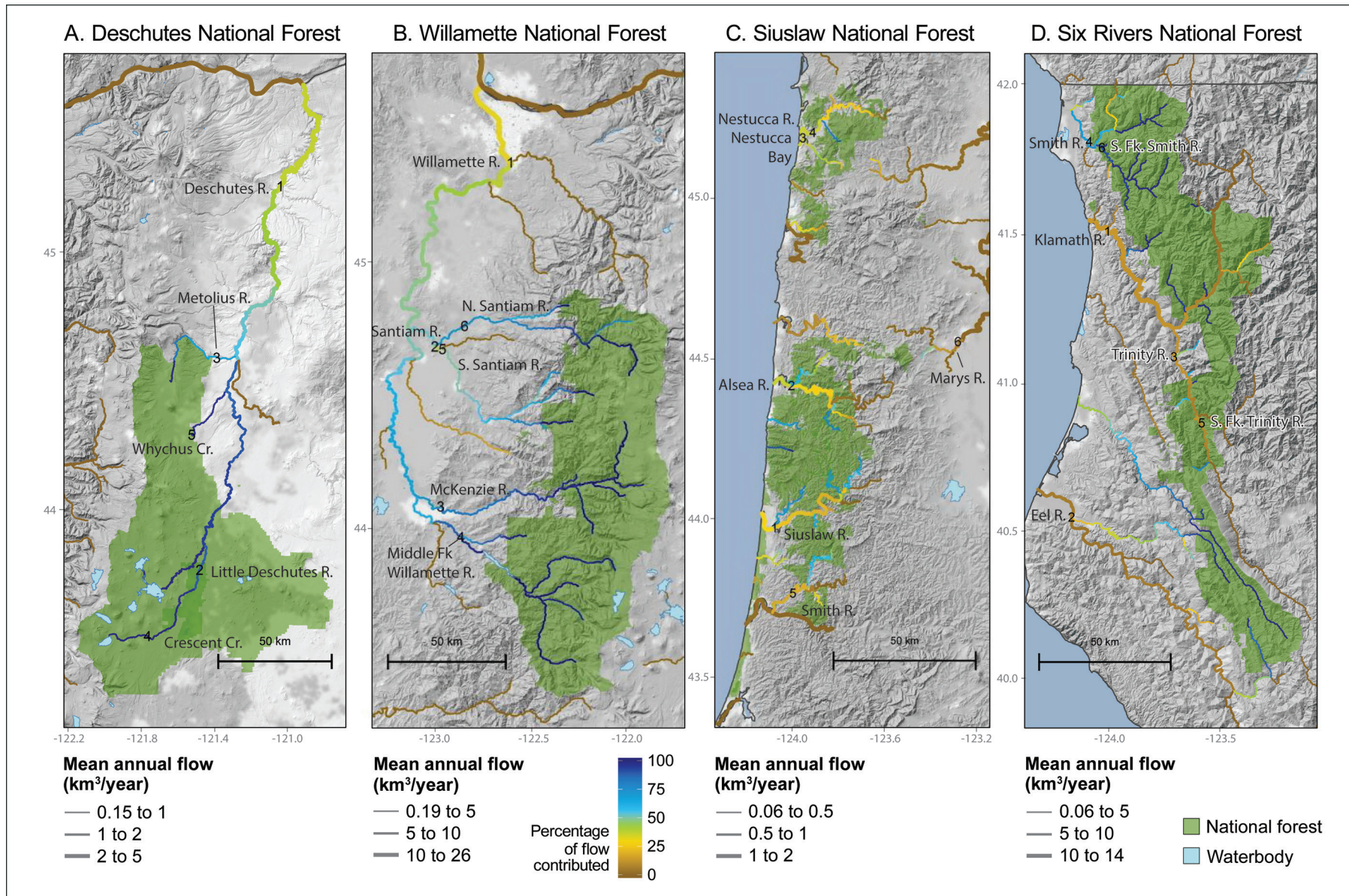
Figure 7-13—Contribution of selected national forests in the Northwest Forest Plan area to the mean annual flow of adjacent watersheds: (A) Deschutes National Forest, central Oregon Cascades; (B) Willamette National Forest, western Oregon Cascades; (C) Siuslaw National Forest, Oregon Coast Range; and (D) Six Rivers National Forest, coastal northern California. ( https://www.fs.fed.us/rmrs/projects/national-forest-contributions-streamflow ).
