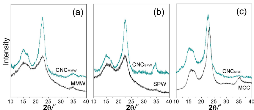
Figure 5. X-ray powder diffractograms of the hydrolyzed residuals (HRs), MCC, and the CNCs. (a) MMW and its resulted CNC MMW ; (b) SPW and its resulted CNC SPW ; (c) MCC and its resulted CNC MCC .
