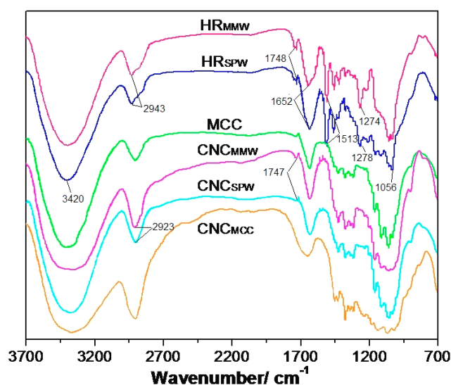
Figure 1. Fourier transform infrared spectroscopy (FTIR) spectra of hydrolyzed residues, MCC, and their cellulose nanocrystals (CNCs).
