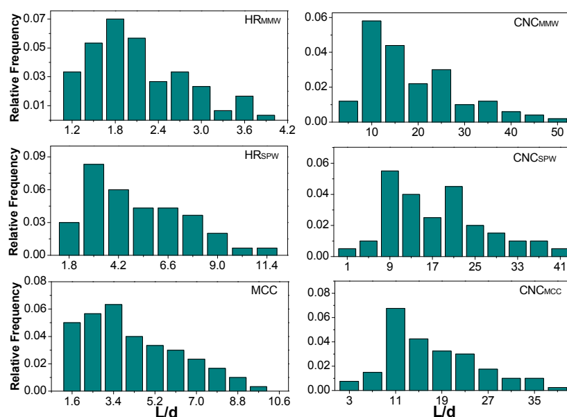
Figure 3. Aspect ratio distributions of HR MMW , HR SPW , MCC, and their CNCs.
