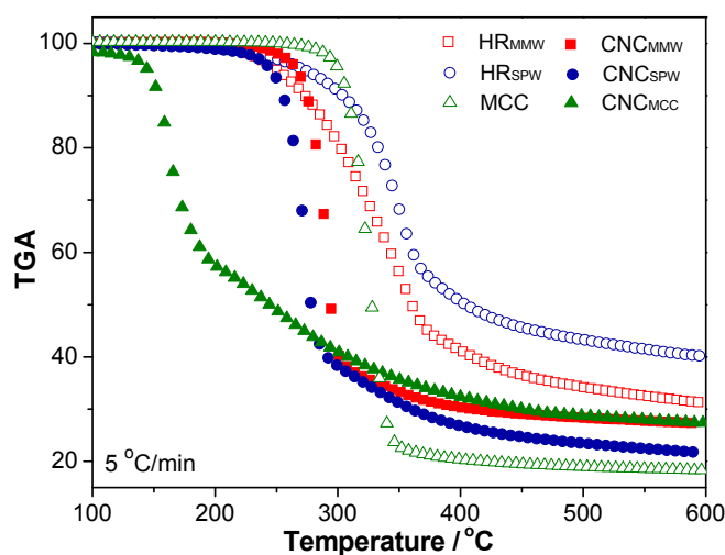
Figure 6. Thermogravimetric curves of the hydrolyzed residuals, MCC and the resulted CNCs.
