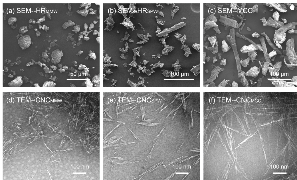
Figure 2. Scanning electron microscope (SEM) and transmittance electron microscope (TEM) images of HR MMW , HR SPW , MCC, and their CNCs. (a) hydrolyzed residues from medium milled wood, HR MMW ; (b) hydrolyzed residues from sulfite pretreated wood, HR SPW ; (c) microcrystalline cellulose, MCC; (d) cellulose nanocrystals from HR MMW , CNC MMW ; (e) cellulose nanocrystals from HR SPW , CNC SPW ; (f) cellulose nanocrystals from MCC, CNC MCC . (a), (b), (c) were SEM images and (d), (e), (f) were TEM images
