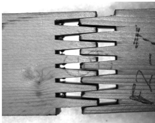
Figure 9. Finger joint after failure showing smooth wood surfaces that could be easily refit together.
