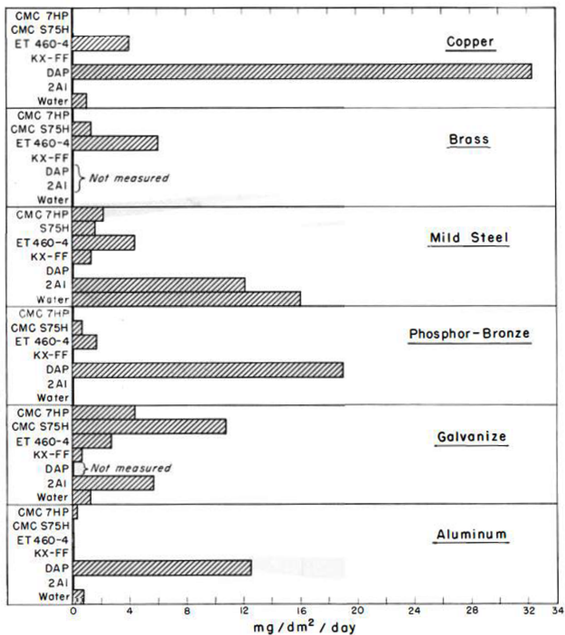
Figure 10.--Weight loss due to corrosion during a 48-hour test using the total immersion procedures described in The Chemical Engineer Handbook. (Perry, 1950.)
