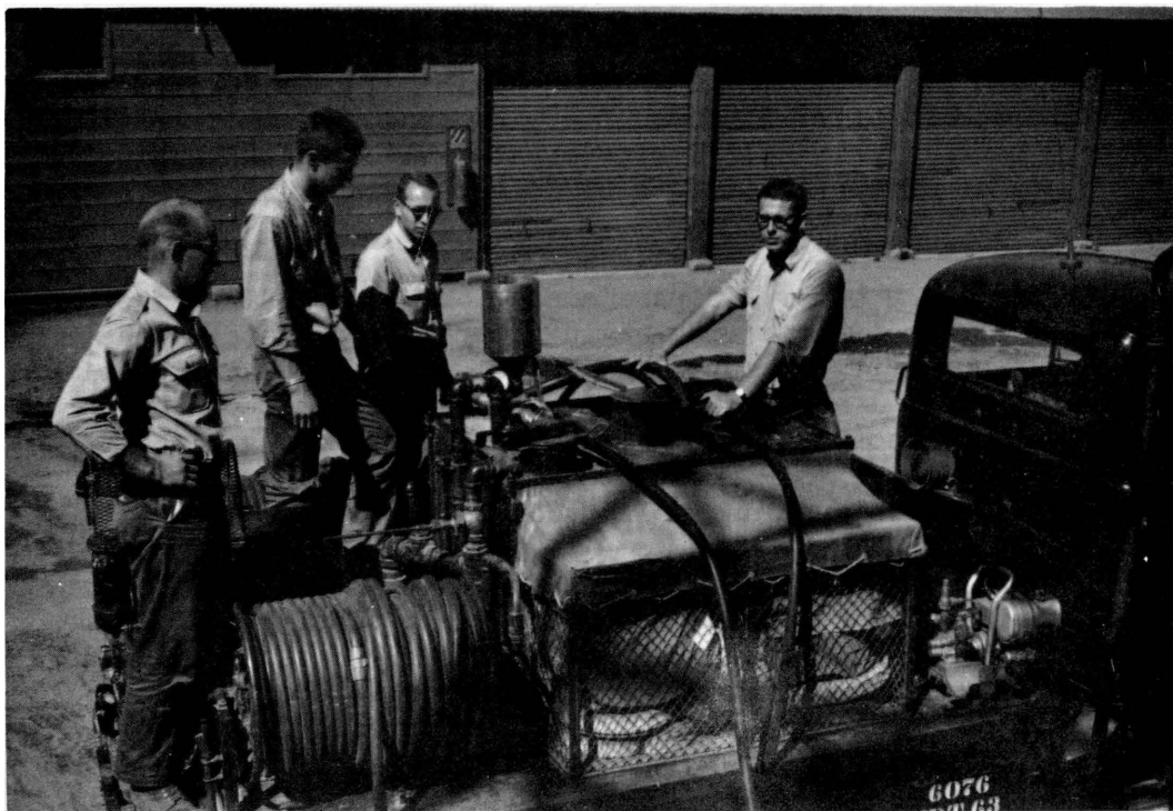
Figure 5.--Viscous water mixing equipment installed on a U. S. Forest Service fire truck at Mt. Shasta Ranger Station.
