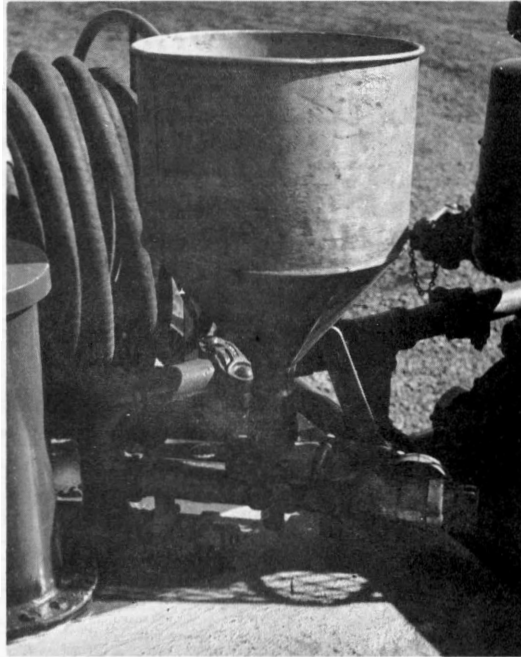
Figure 6.-- Closeup of viscous water mixing equipment installed on a California Division of Forestry truck at Cathay Fire Station.
