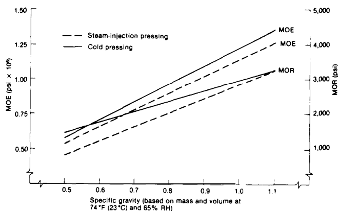
Figure 3.—Regression equation plots of compression properties versus specific gravity for cold pressing, and steam-injection pressing. (ML835277)
