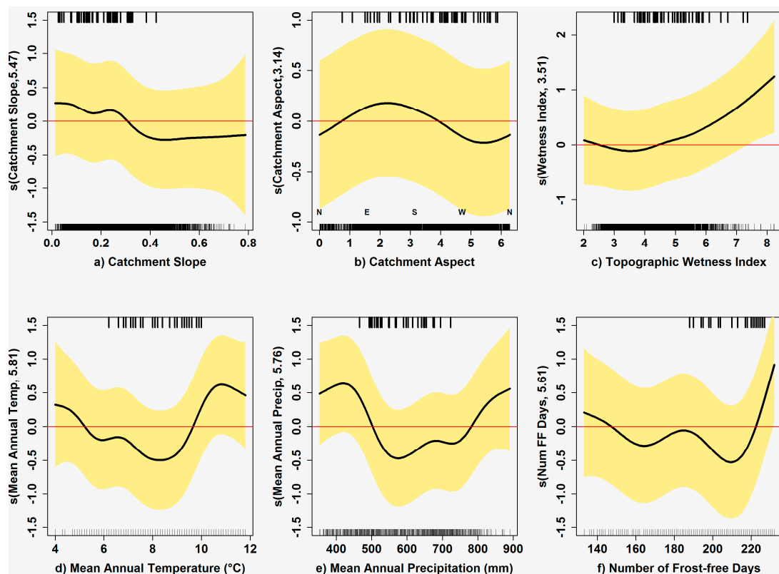
Figure 3. Generalized Additive Model (GAM) smooth plots for the models with three terrain and one climate predictor represent the change in the Refugial Gradient (RG) value ( y -axis) relative to variation in terrain and spatial climate ( x -axis). Relationships with terrain variables (a–c) remained the same for all models that included one climate variable. Neighborhoods that were more densely populated with refugia occurred on gentle slopes, but sparsely populated neighborhoods were more likely on moderate and steep slopes (a). Refugia were more abundant in neighborhoods on east-southeasterly aspects (b) and areas with higher soil moisture (c). Greater density of refugia tended to occur at the high and low end of the range in variability in climate (d–f). Confidence intervals, shaded yellow, include the uncertainty about the overall mean (R-mgcv gam plot option seWithMean = TRUE [55]). Rugs at the bottom of each plot represent the distribution of random samples; the top rugs represent the distribution of field samples.
