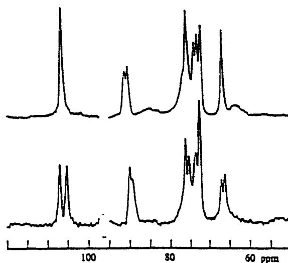
Figure 2. Solid state ^{13}\text{C} NMR spectra of: (a) the \text{I}_\alpha form; (b) the \text{I}_\beta form. The spectra were generated from linear combinations of spectra (d) and (e) in Figure 1. Discontinuities in the spectra occur where the spinning side bands of polyethylene would have occurred (7).
