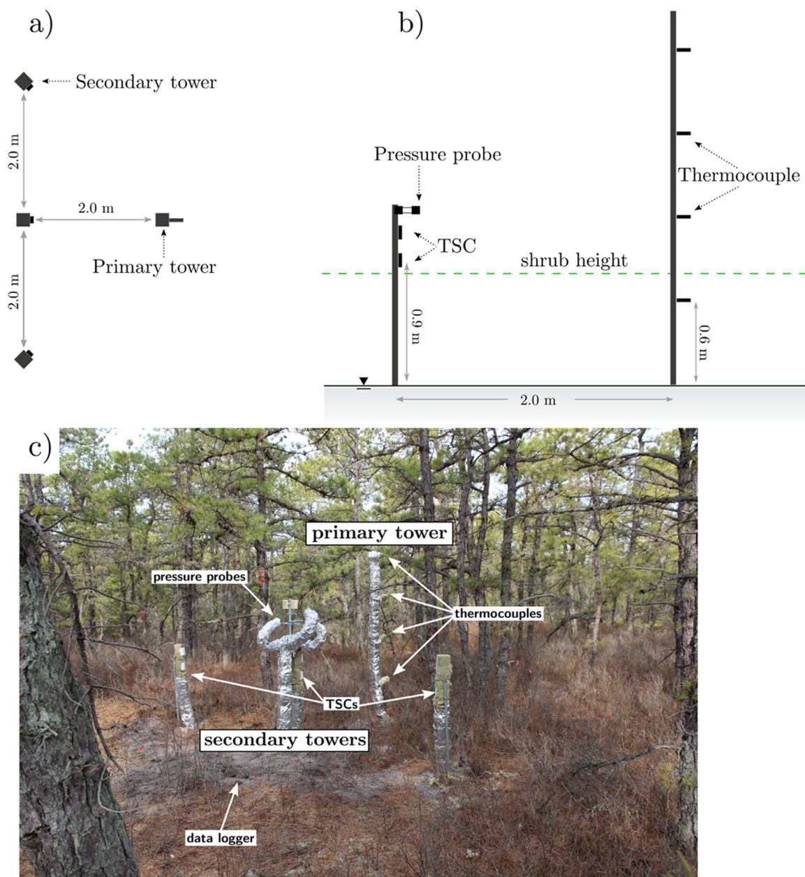
Fig. 2. Configuration of instrument array for fire behavior measurement, shown in (a) plan view, (b) section view, and (c) in-situ.
