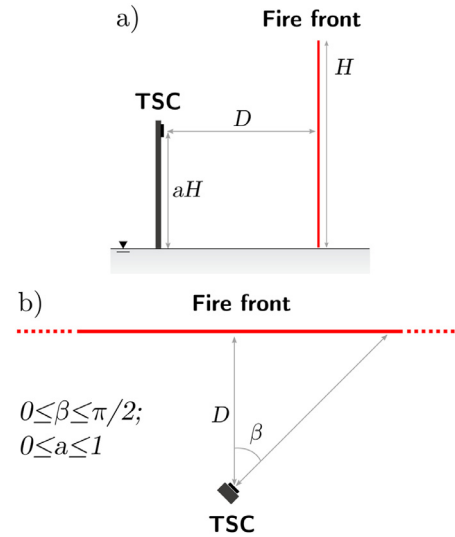
Fig. 10. a) Section and b) plan view of the theoretical orientation of the sensor and flame front.
