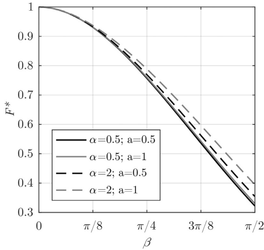
Fig. 11. Examples of view factor corrections for different flame height to distance ratios ( \alpha=0.5 , \alpha=2 ) and different sensor heights ( a=0.5 , Eq. (6); a=1 , Eq. (7)).
